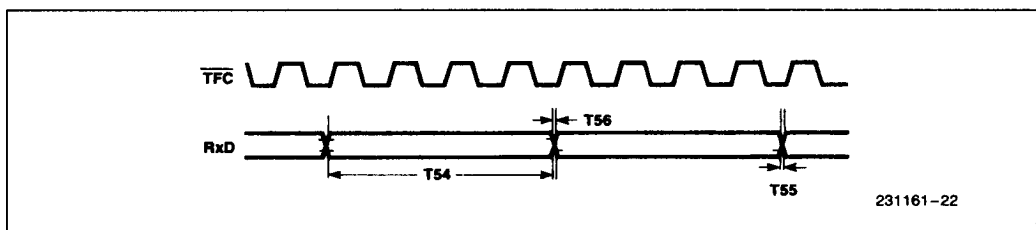
Receive Data Timings (Manchester)
