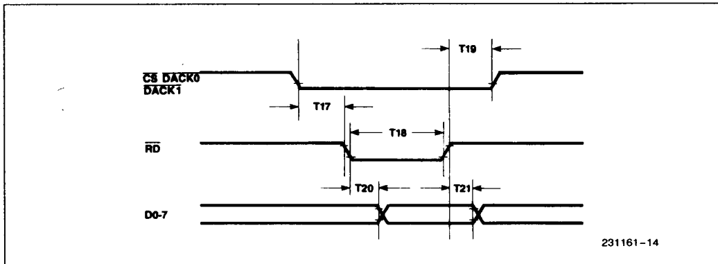
Read Timing
