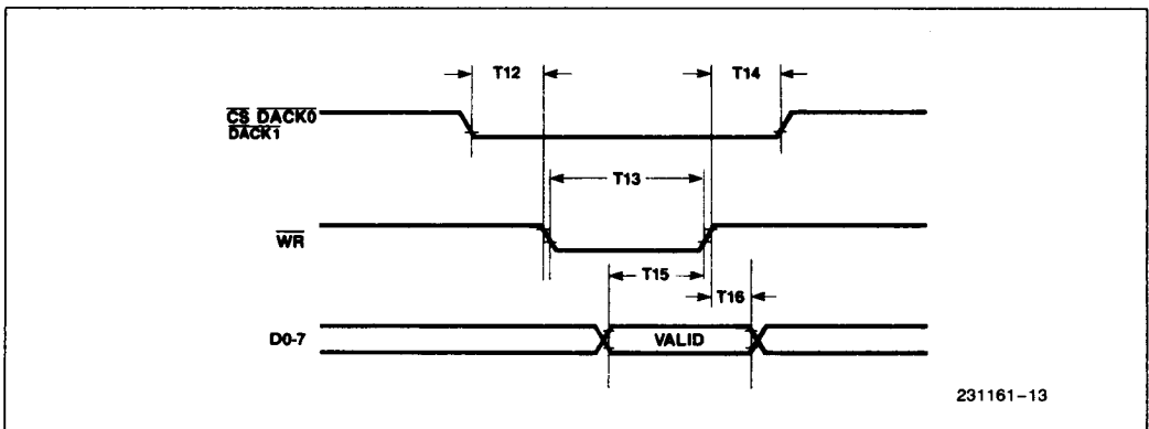
Write Timing
