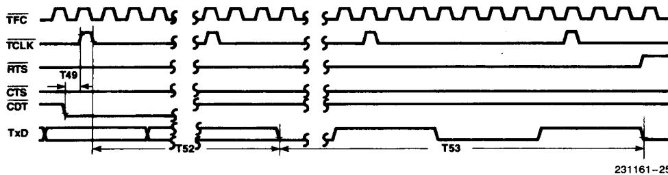
Transmit Timings—Collision Detect and Jamming
