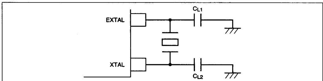
Figure 1 Example of Crystal Resonator Connection
