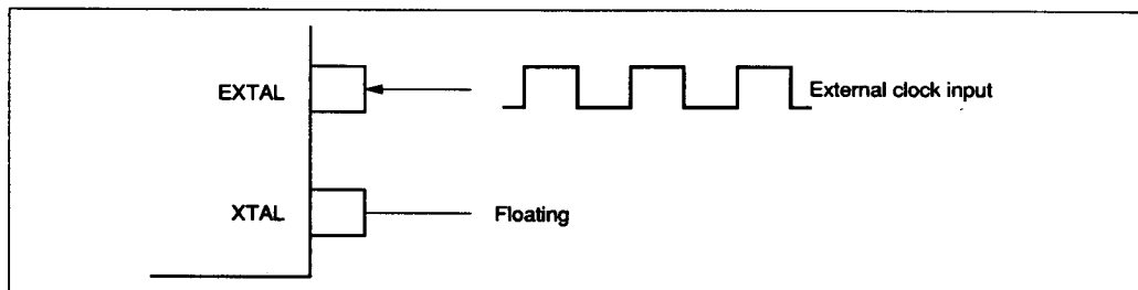
Figure 2 Example of External Clock Connection
