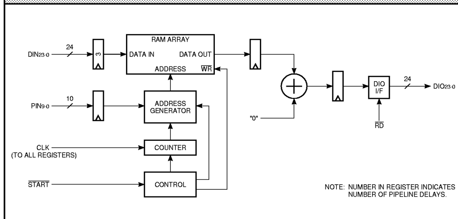
FIGURE 3. LOOK UP TABLE MODE
