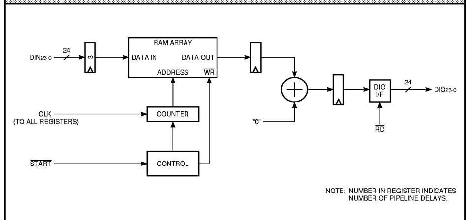
FIGURE 5. DELAY MEMORY MODE
