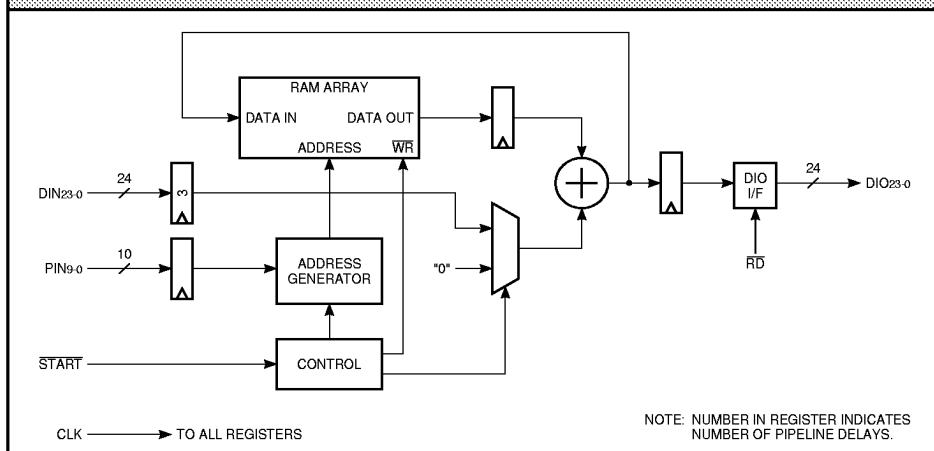
FIGURE 4. BIN ACCUMULATE MODE
