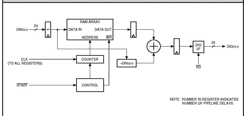
FIGURE 6. DELAY AND SUBTRACT MODE
