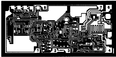
DIE SIZE 0.109 × 0.055 inch, 5995 sq. mils (2.77 × 1.40mm, 3.88 sq. mm)
