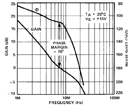
GAIN, PHASE SHIFT vs FREQUENCY
