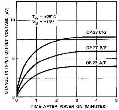
WARM-UP OFFSET VOLTAGE DRIFT
