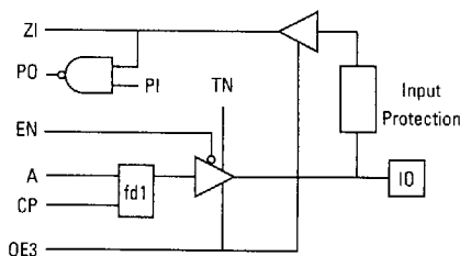
Figure 2. RUPCI Logic Diagram
