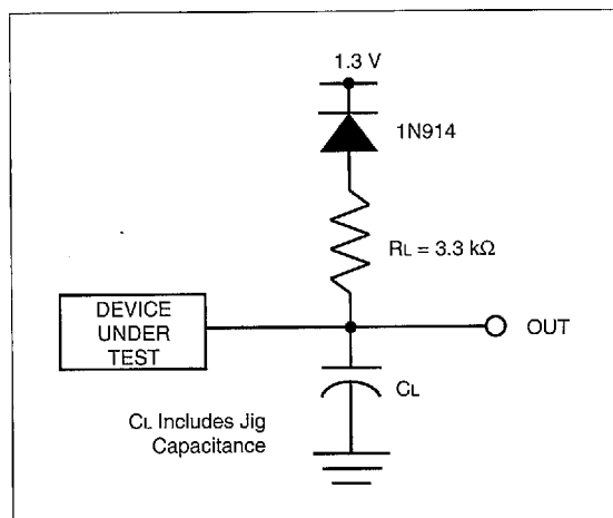
Fig. 7 Transient Equivalent Testing Load Circuit
