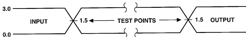
Fig. 5 Transient Input/Output Reference Waveform for V_{CC} = 5.0 \pm 0.25 V (High Speed Testing Configuration)
