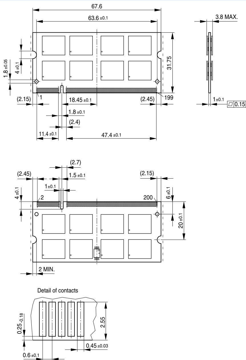
FIGURE 2 Package Outline SO-DIMM L-DIM-200-22
