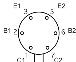
TO-78 (Bottom View)
