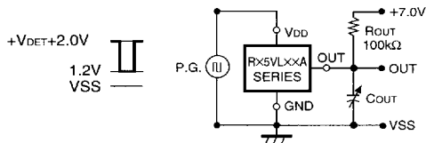
FIG. 7 Output Delay Time Test Circuit
