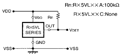
FIG. 4 Detector Threshold Test Circuit
