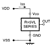
FIG. 3 Supply Current Test Circuit
