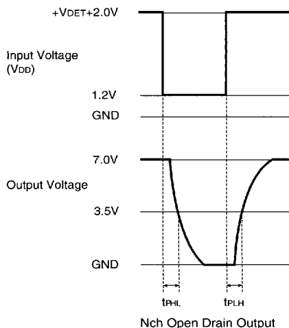
Nch Open Drain Output
