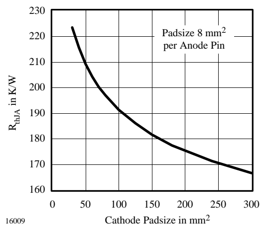
Figure 6. Thermal Resistance Junction Ambient vs. Cathode Pads Size
