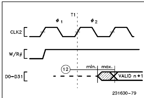
Figure 9-5a. Write Data Valid Delay Timing (25 MHz, 33 MHz)
