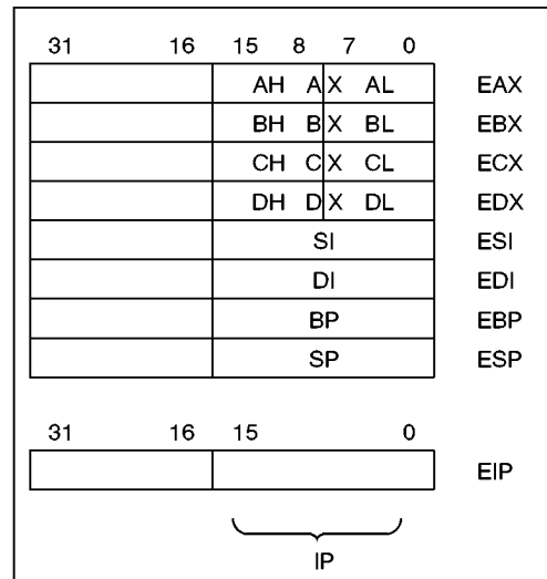
Figure 2-2. General Registers and Instruction Pointer
