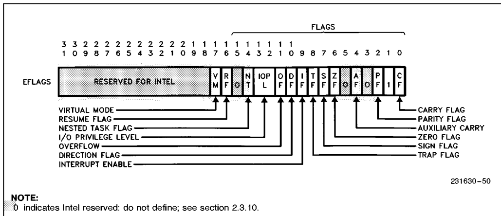
Figure 2-3. Flags Register
