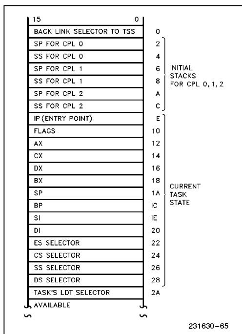
Figure 4-16. 80286 TSS
