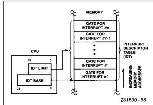
Figure 4-4. Interrupt Descriptor Table Register Use
