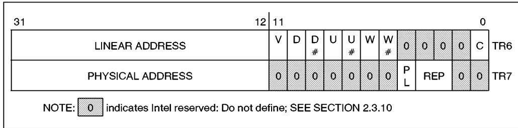
Figure 2-12. Test Registers
