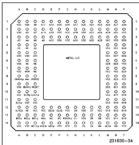
Figure 1-2. Intel386™ DX PGA Pinout—View from Pin Side
