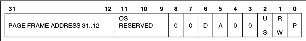
Figure 4-21. Page Table Entry (Points to Page)
