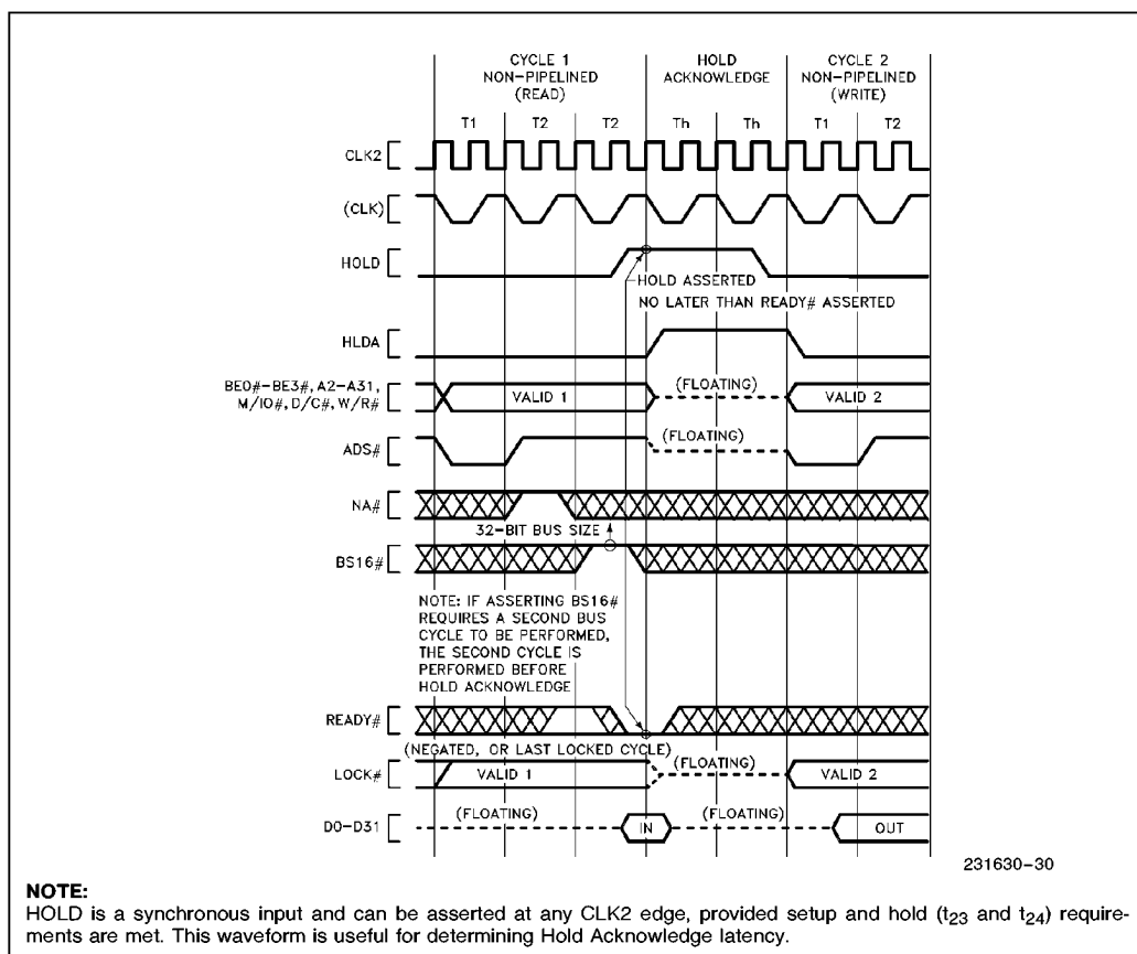
Figure 5-26. Requesting Hold from Active Bus (NA# negated)
