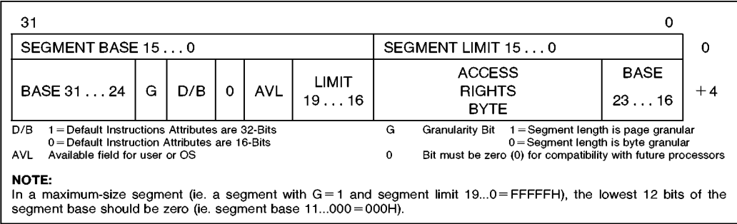
Figure 4-6. Segment Descriptors
