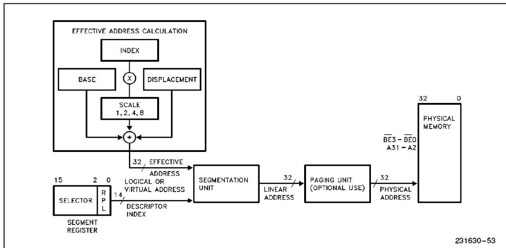
Figure 2-11. Address Translation
