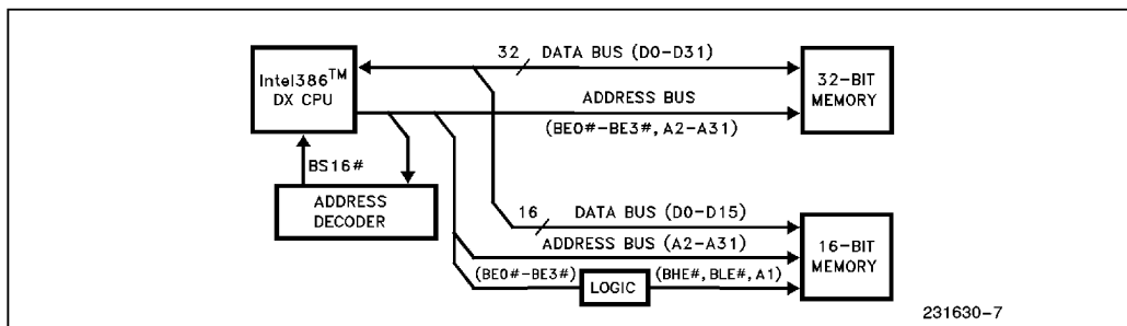
Figure 5-6. Intel386™ DX with 32-Bit and 16-Bit Memory
