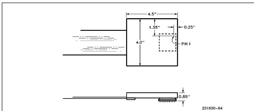
Figure 7-1. Processor Module Dimensions
