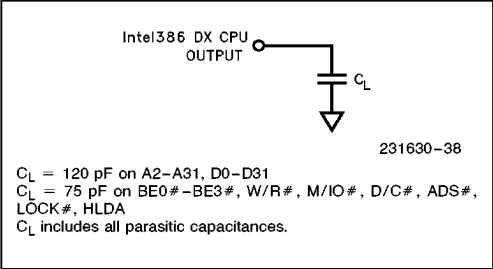
Figure 9-2. A.C. Test Load
