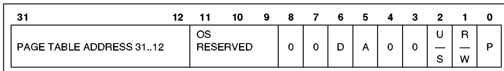
Figure 4-20. Page Directory Entry (Points to Page Table)
