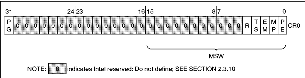
Figure 2-5. Control Register 0
