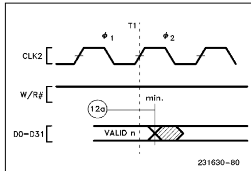
Figure 9-5b. Write Data Hold Timing (25 MHz, 33 MHz)
