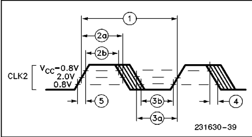
Figure 9-3. CLK2 Timing
