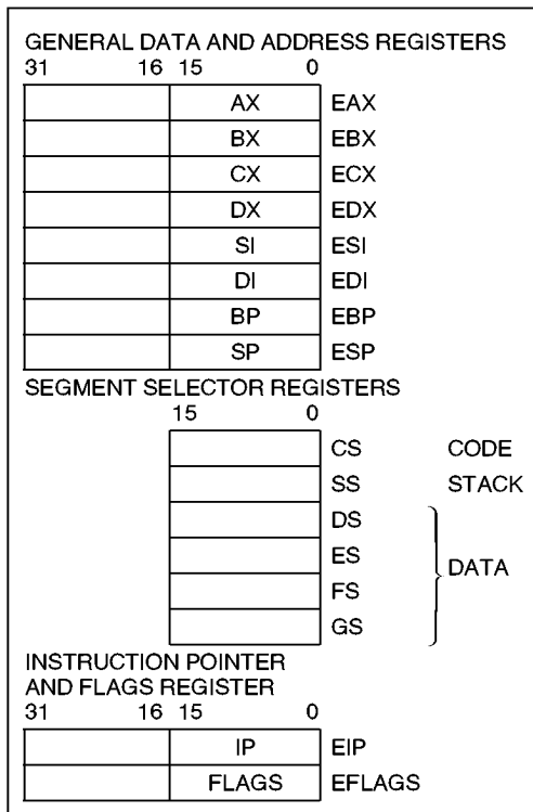
Figure 2-1. Intel386™ DX Base Architecture Registers
