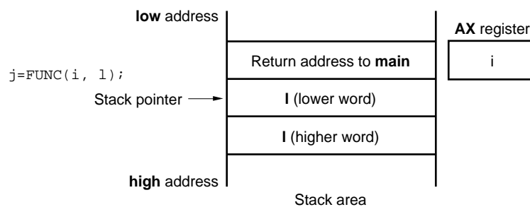
Figure 12-5. Stack Positions of Arguments
