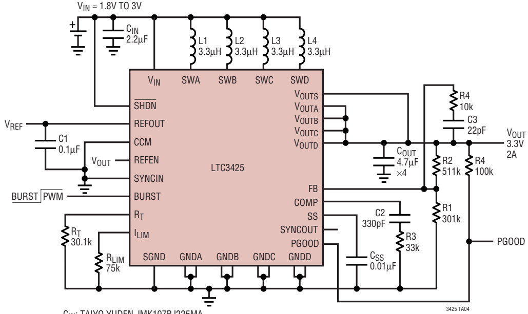
Application with User Commanded Burst Mode Operation and Buffered Reference Output Enabled
