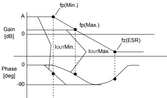
Fig.33 Open loop gain characteristics
