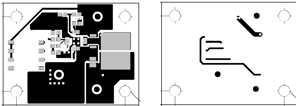
Fig.38 Layout diagram
