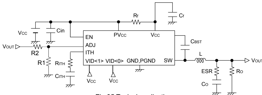
Fig.35 Typical application
