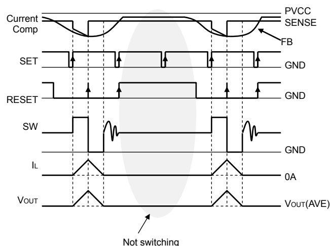
Fig.25 SLLM™ switching timing chart
