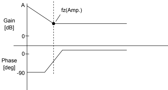
Fig.34 Error amp phase compensation characteristics
