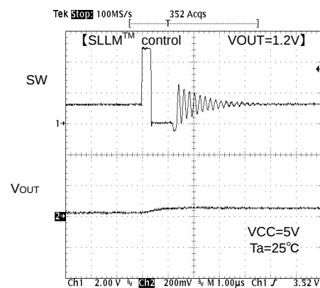
Fig.14 SW waveform Io=0mA
