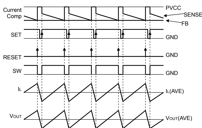
Fig.24 PWM switching timing chart
