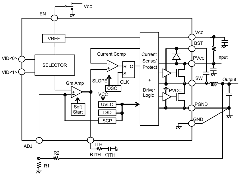
Fig.2 Block Diagram
