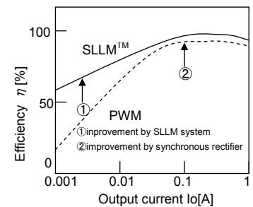
Fig.21 Efficiency
