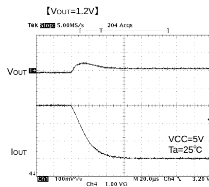
Fig.17 Transient Response Io=4A→1A(20μs)
