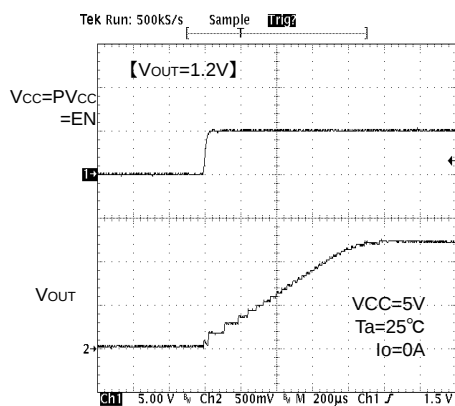
Fig.13 Soft start waveform
