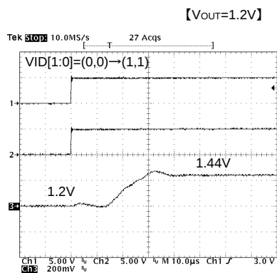
Fig.18 Change Response
