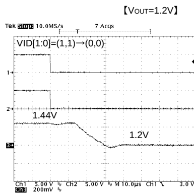
Fig.19 Change Response
