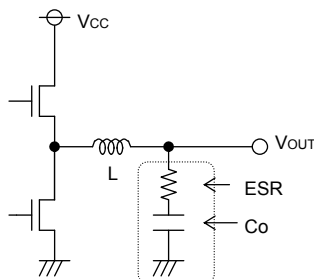
Fig.31 Output capacitor
