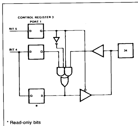
Figure 40 : Data Direction : CPU-to-I/O Operation.
