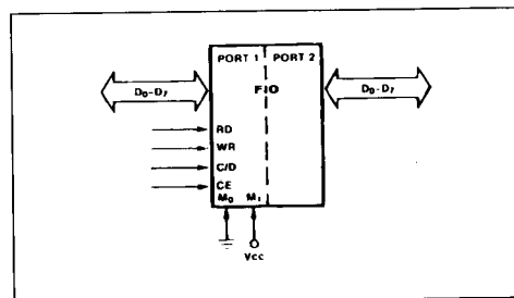
Figure 15: Non-Z-BUS (nonmultiplexed) Microprocessor Configuration.
