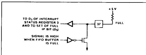
Figure 20 : Full Pin.
