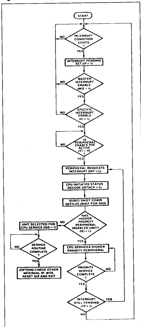
Figure 31 : Interrupt Flowchart.
