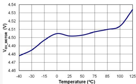
Figure 13. Motor OVP Threshold Voltage ( V_{OV\_MOTOR} ) vs. Temperature
