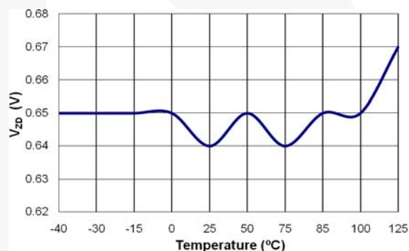
Figure 15. PWM Zero Duty Voltage ( V_{ZD} ) vs. Temperature
