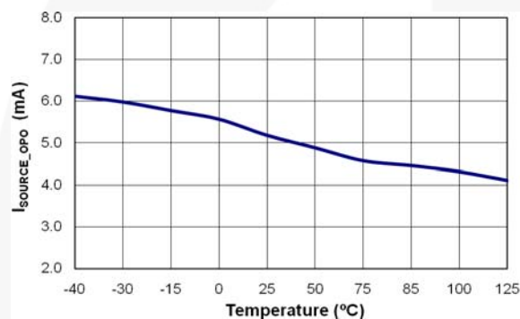
Figure 8. OPO Current Source ( I_{SOURCE\_OPO} ) vs. Temperature
