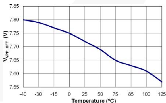
Figure 17. V_{PP} Turn-Off Threshold Voltage ( V_{VPP\_OFF} ) vs. Temperature
