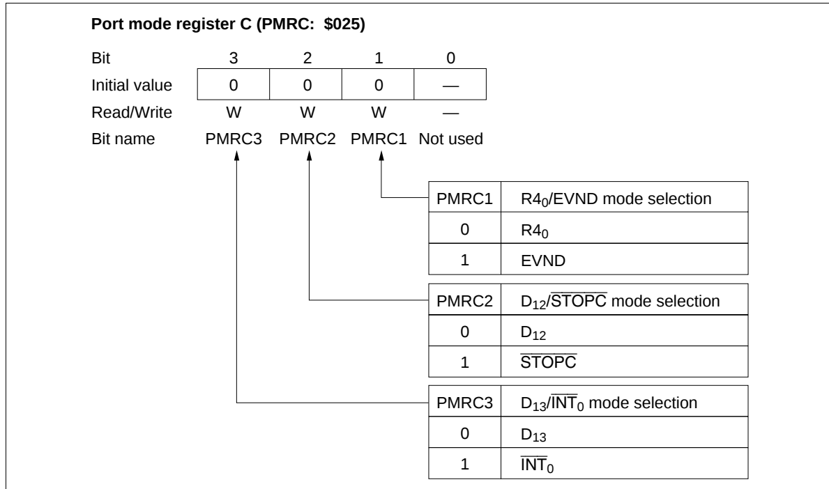
Figure 47 Port Mode Register C (PMRC)
