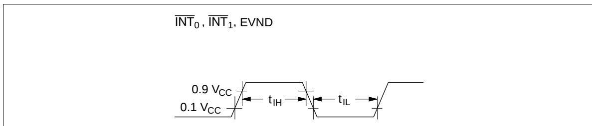
Figure 70 Reset Timing
