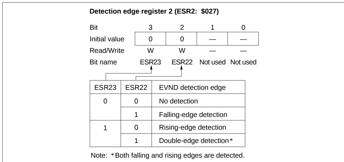
Figure 48 Detection Edge Select Register 2 (ESR2)
