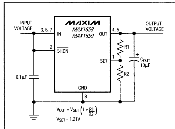
Figure 3. Adjustable Output Configuration Using External Feedback Resistors
