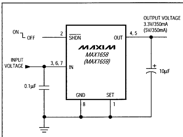
Figure 2. Preset Output Configuration
