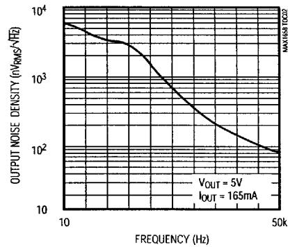
OUTPUT NOISE DENSITY vs. FREQUENCY
