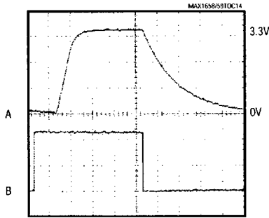
100µs/div A: OUTPUT VOLTAGE (1V/div) B: \overline{SHDN} PIN VOLTAGE (2V/div)
