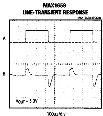
A: INPUT VOLTAGE (1V/div), V_{IN} = 7V (HIGH), V_{IN} = 6V (LOW) B: OUTPUT VOLTAGE (100mV/div)
