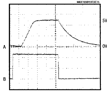
100µs/div A: OUTPUT VOLTAGE (2V/div) B: \overline{SHDN} PIN VOLTAGE (2V/div)
