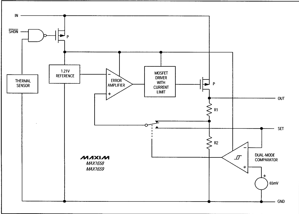
Figure 1. Functional Diagram
