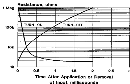
Response Time VTL2C1
