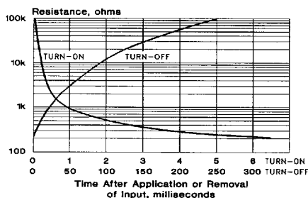
Response Time VTL2C2
