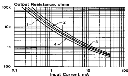
Output Resistance vs Input Current VTL2C2
