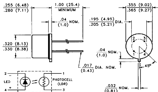
TO-5 PACKAGE OUTLINE
