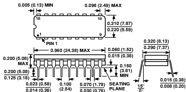
18-Lead Cerdip (Q-18)
