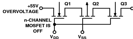
Figure 12. +55 V Overvoltage Input to the ON Channel
