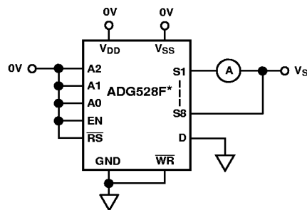
Test Circuit 6. Input Leakage Current (with Power Supplies OFF)
