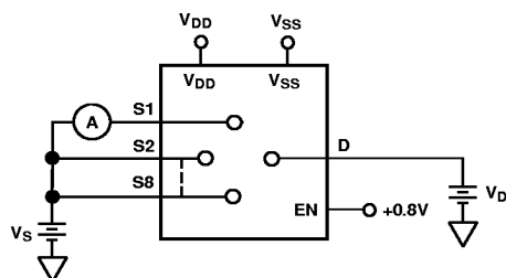
Test Circuit 5. Input Leakage Current (with Overtolerance)
