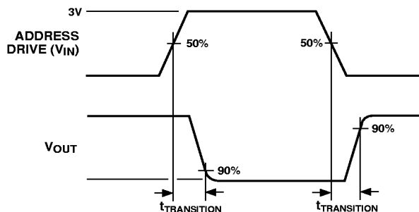
Test Circuit 7. Switching Time of Multiplexer, t_{TRANSITION}
