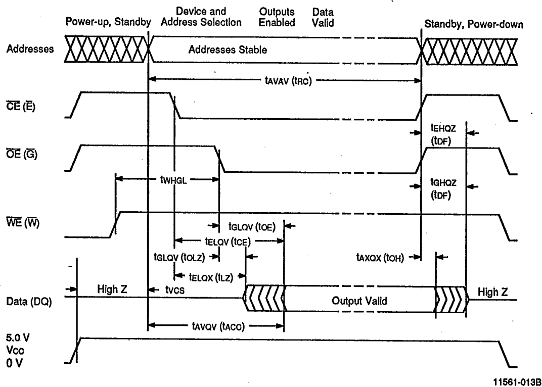
Figure 5. AC Waveforms for Read Operations
