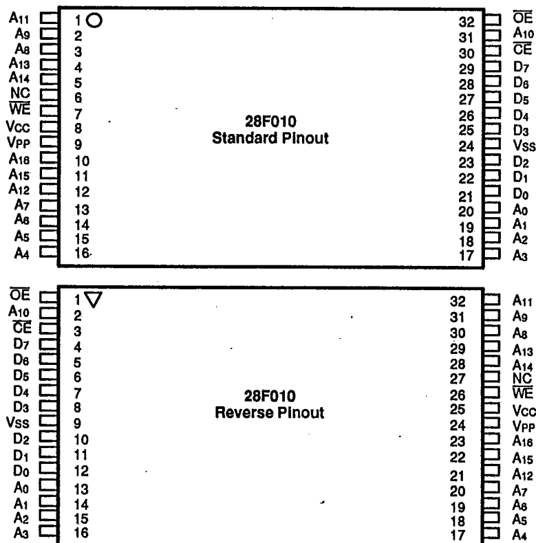
28F010 128K x 8 Flash Memory in 32 Lead TSOP
