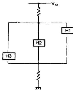
Figure 8 Hall effect element electrical connections
