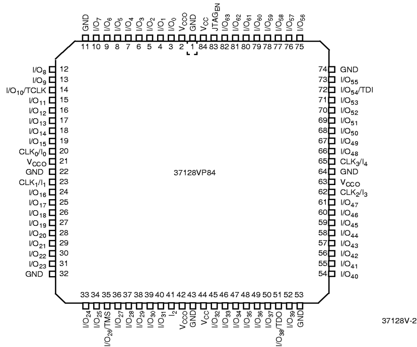
84-pin PLCC Top View
