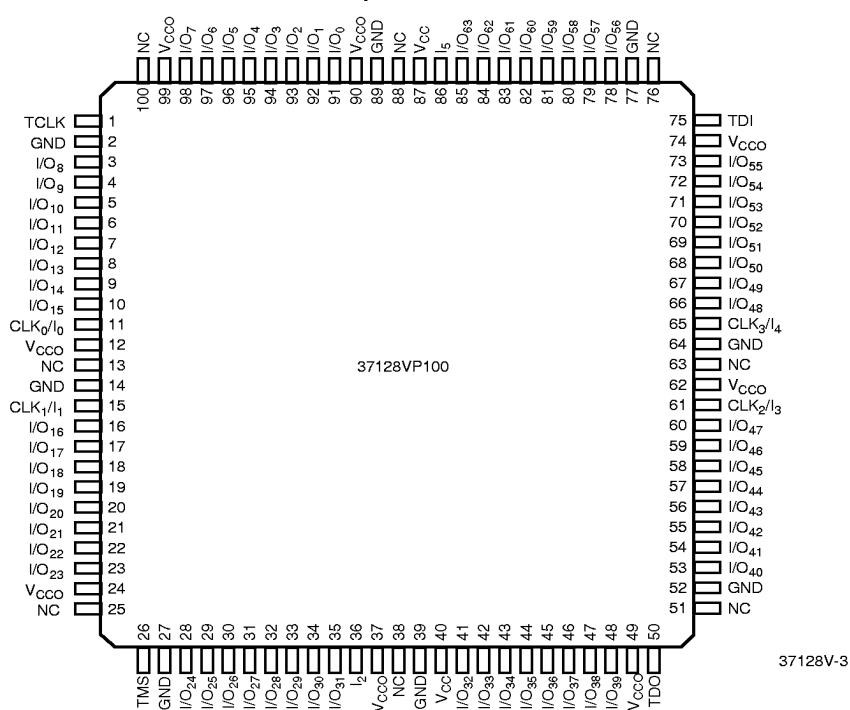
100-pin TQFP Top View
