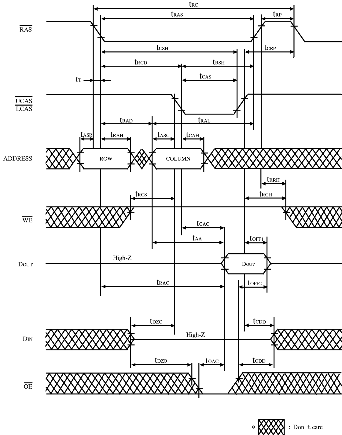
FIGURE 1. READ CYCLE
