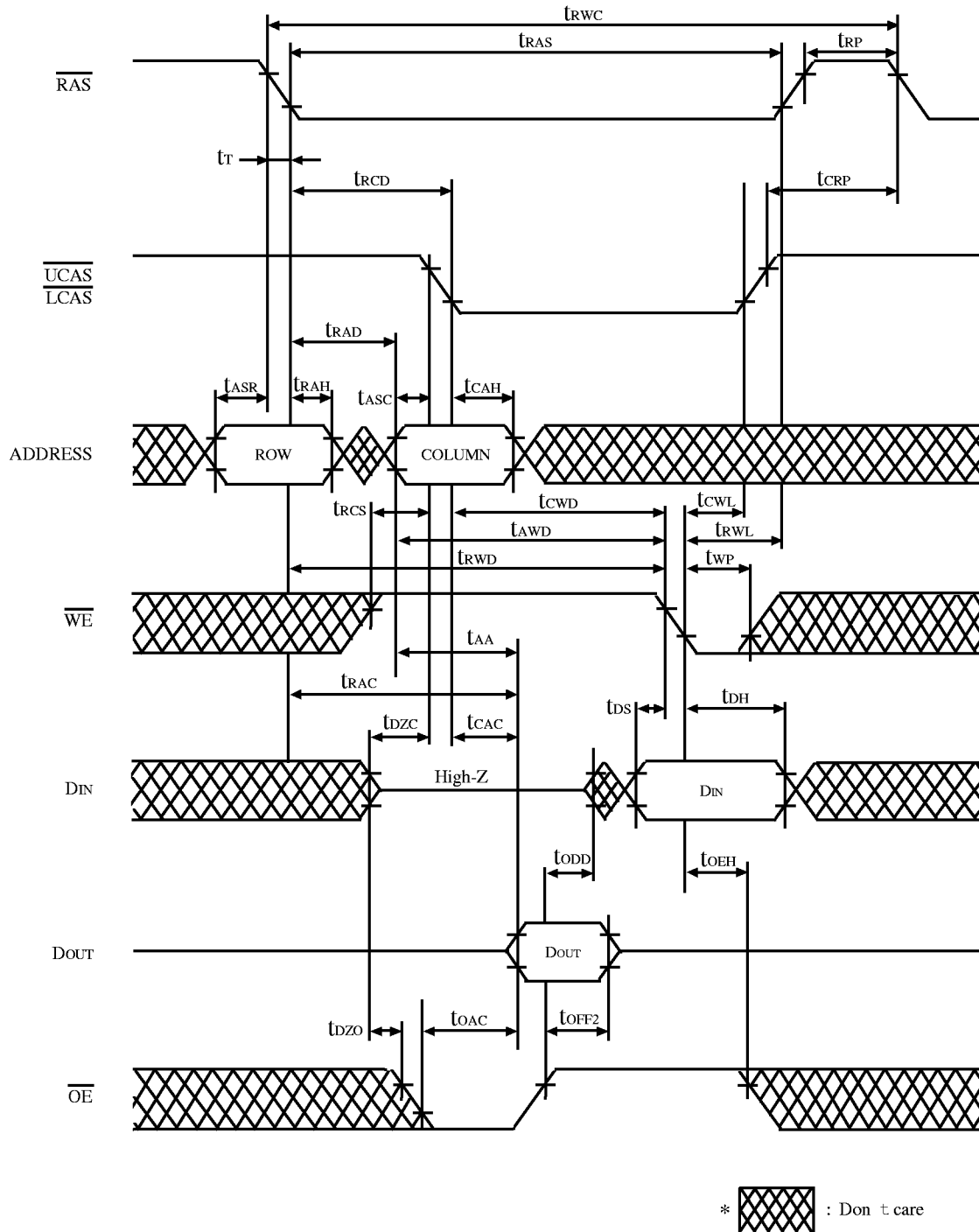
FIGURE 4. READ MODIFY WRITE CYCLE
