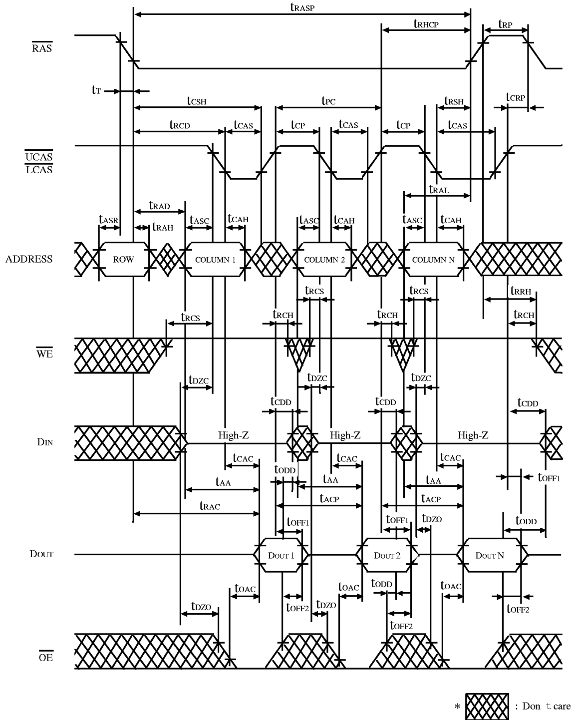
FIGURE 8. FAST PAGE MODE READ CYCLE
