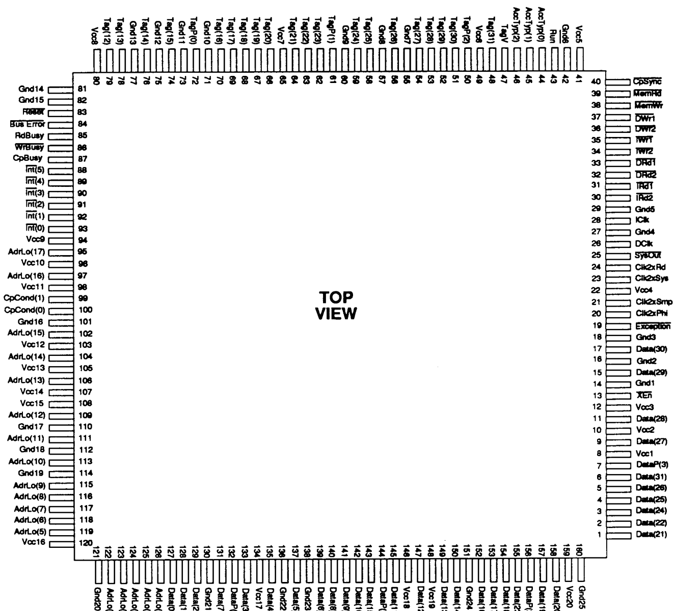
Figure 5.5 PR3000A Pin Diagram—160-Lead Metal Quad Flat Pack, Gull Wing, Cavity Down, EIAJ Standard
