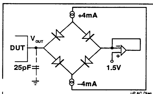
Figure 3.5.1 OUTPUT LOADING FOR AC TESTING
