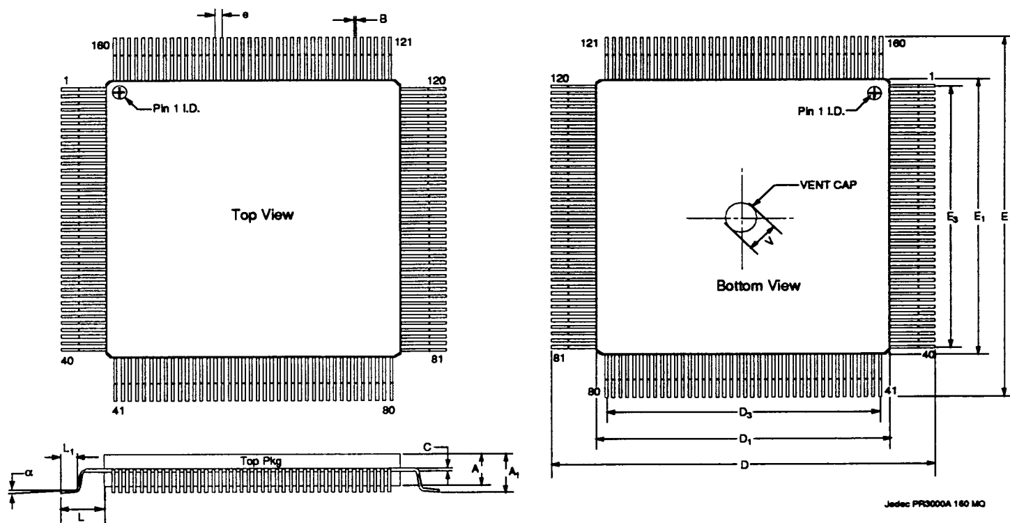
Figure 5.6 PR3000A Package Dimensions--160-Lead Metal Quad Flat Pack, Gull Wing, Cavity Down, EIAJ Standard
