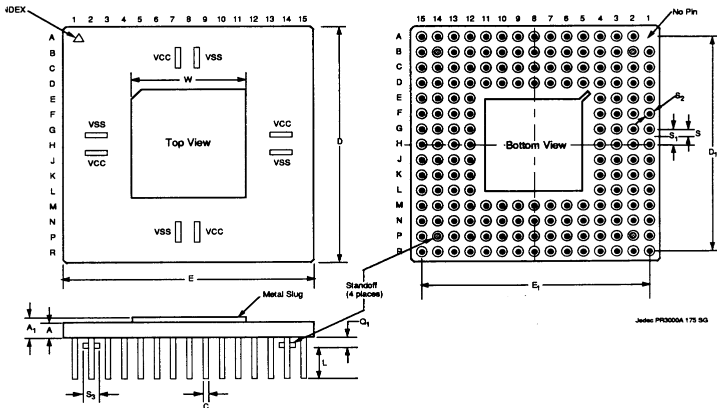
Figure 5.4 PR3000A Package Dimensions — 175-Pin Ceramic Pin Grid Array, Cavity Down
