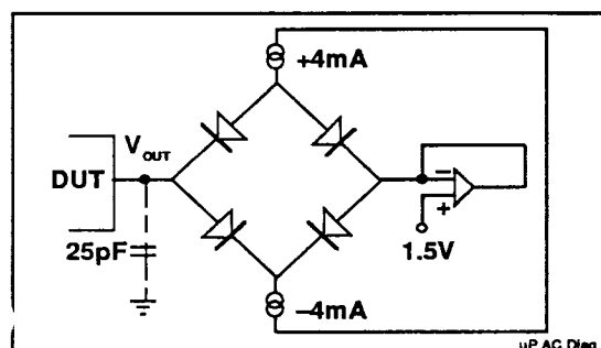
Figure 4.5.1 OUTPUT LOADING FOR AC TESTING
