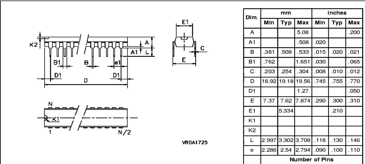
Figure 27.16-Pin Plastic Dual In Line Package (B), 300-mil Width
