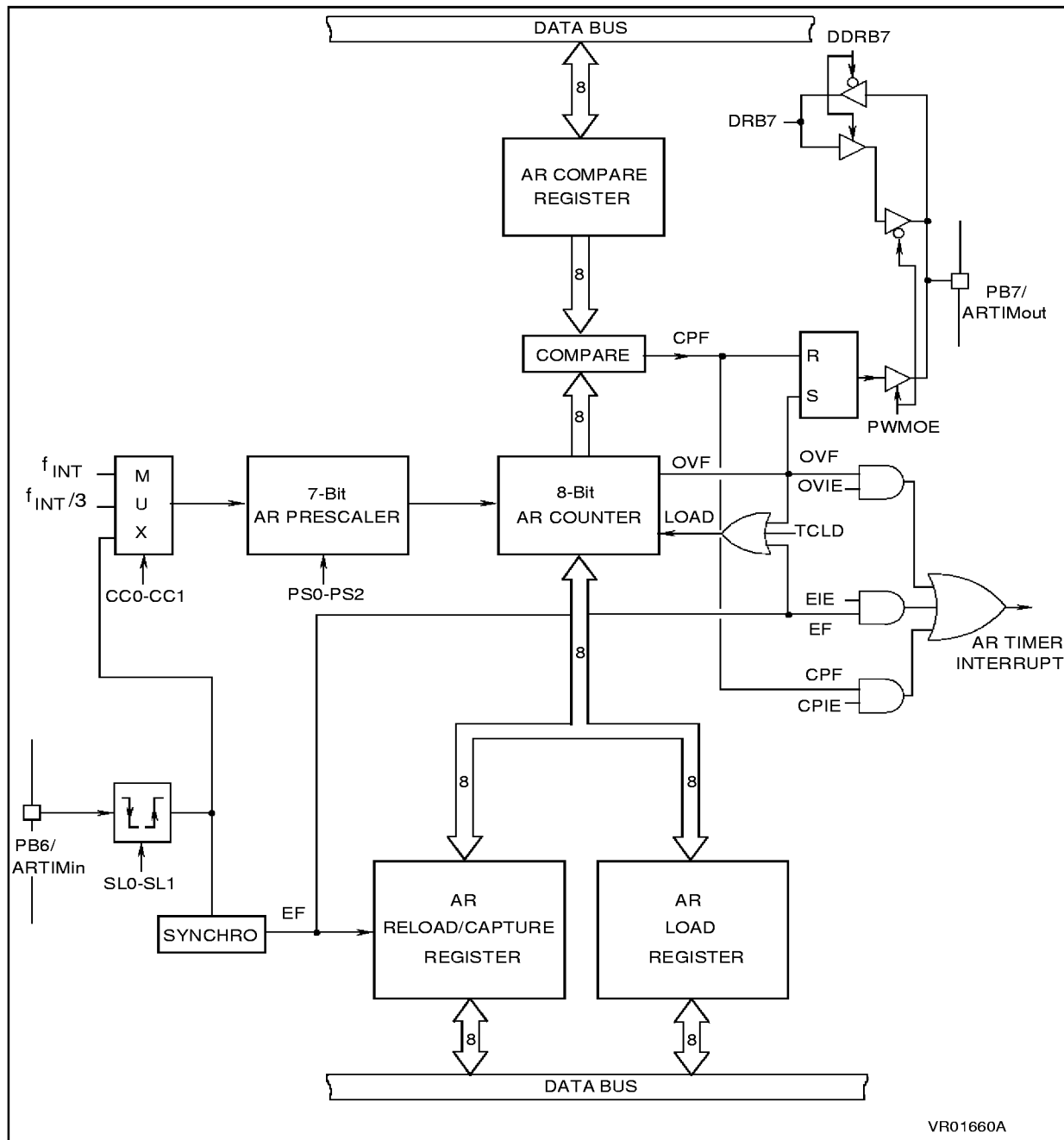
Figure 23. . AR Timer Block Diagram
