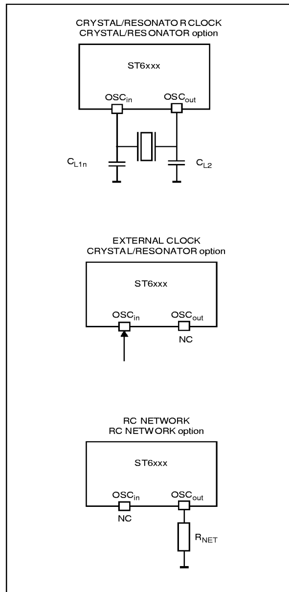
Figure 8. Oscillator Configurations
