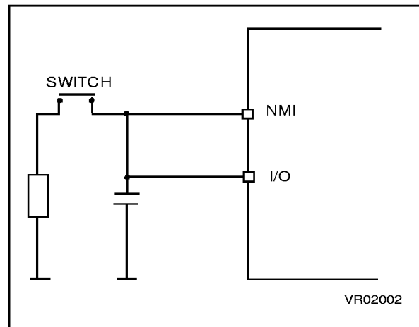
Figure 14. A typical circuit making use of the EXTERNAL STOP MODE CONTROL feature
