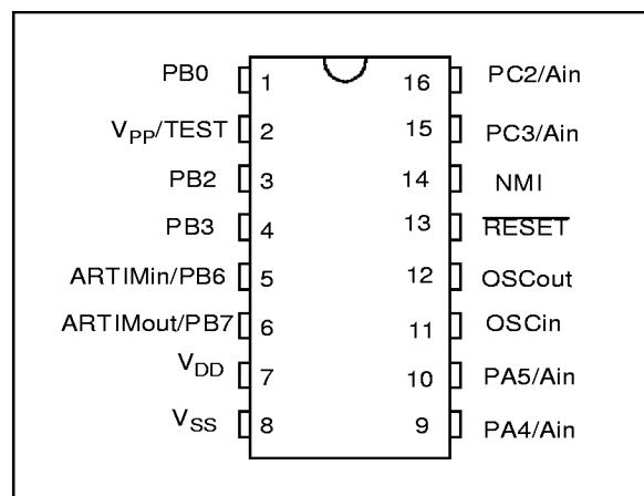
Figure 2. ST62T52B, E62B and T62B Pin Configuration
