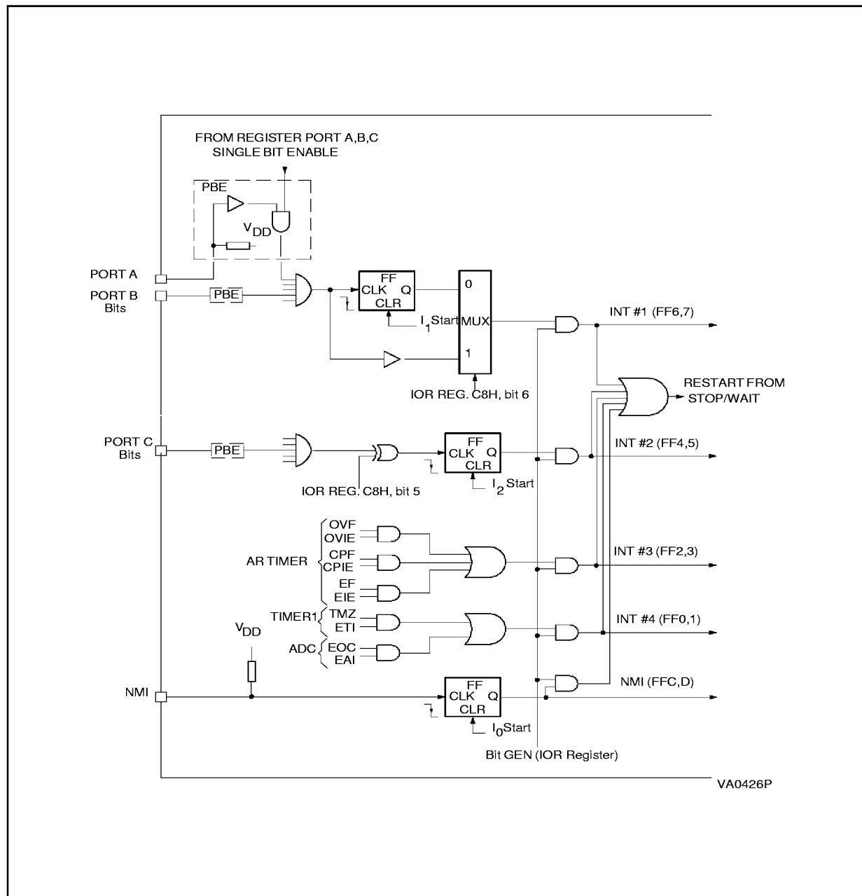
Figure 17. Interrupt Block Diagram
