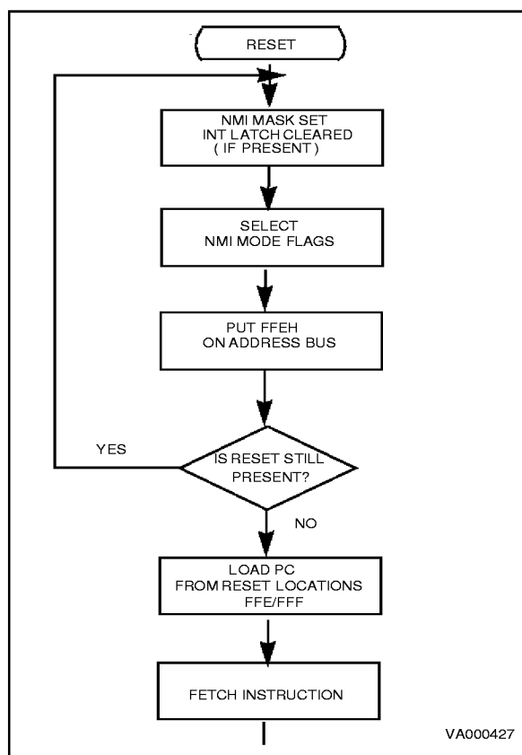
Figure 10. Reset and Interrupt Processing
