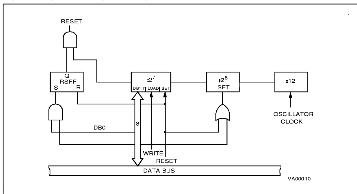
Figure 15. Digital Watchdog Block Diagram
