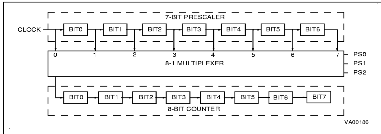
Figure 22. Timer Working Principle
