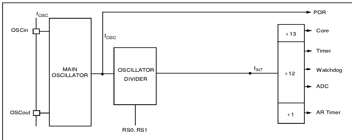
Figure 9. Clock Circuit Block Diagram
