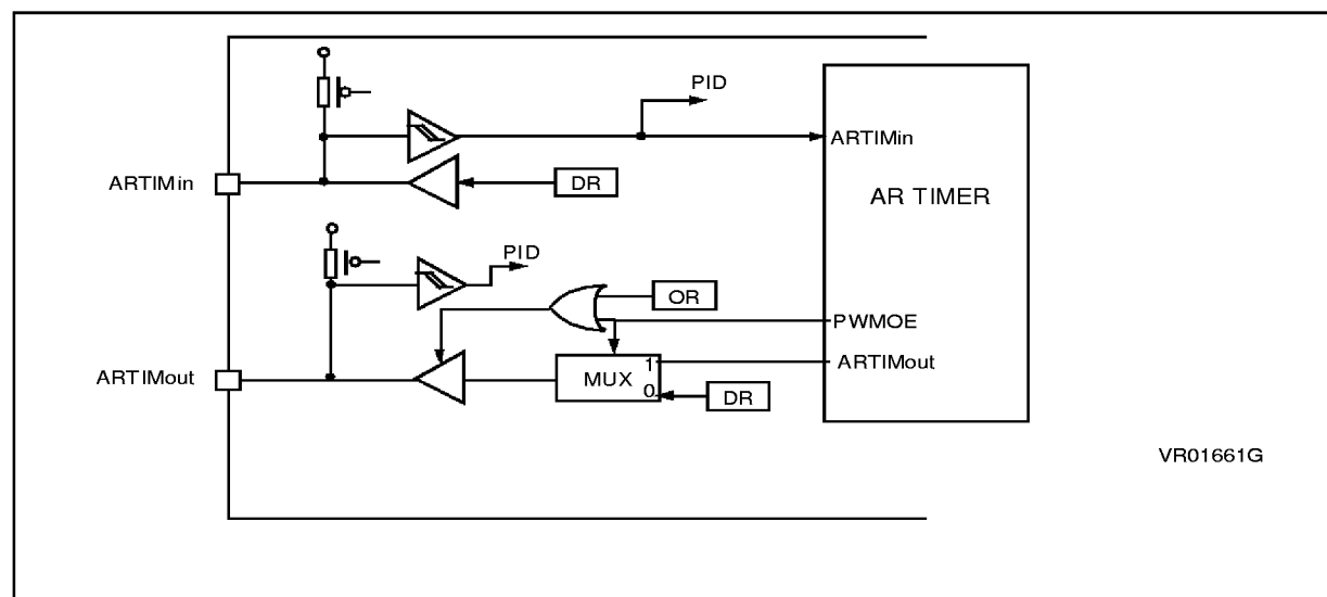
Figure 20. Peripheral Interface Configuration of AR Timer
