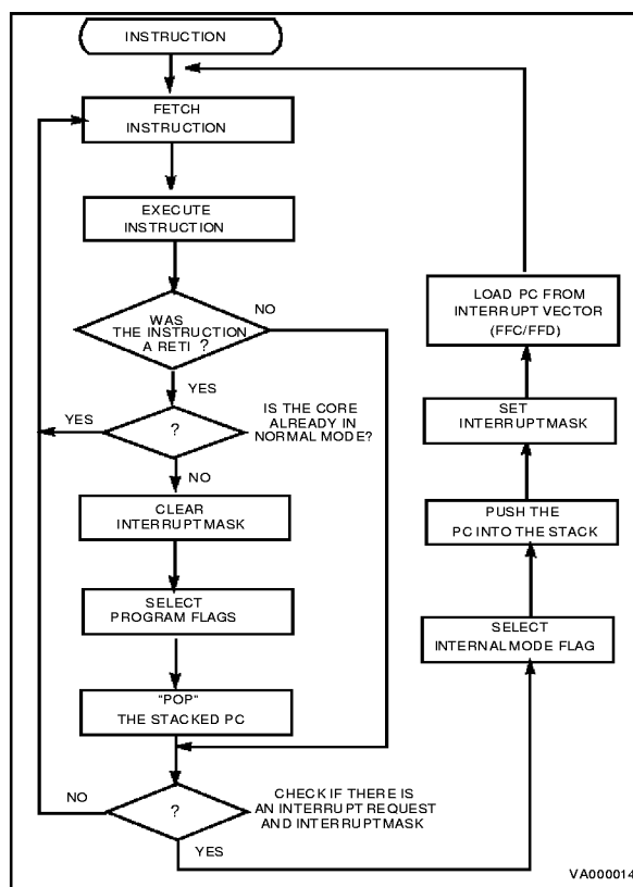
Figure 16. Interrupt Processing Flow Chart
