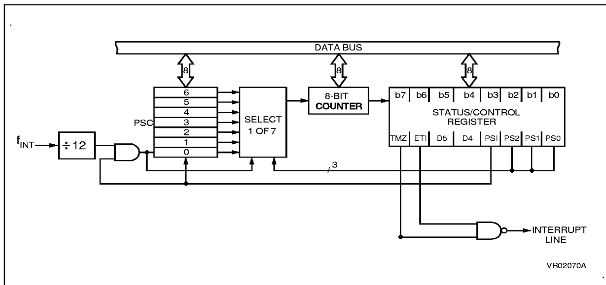
Figure 21. Timer Block Diagram
