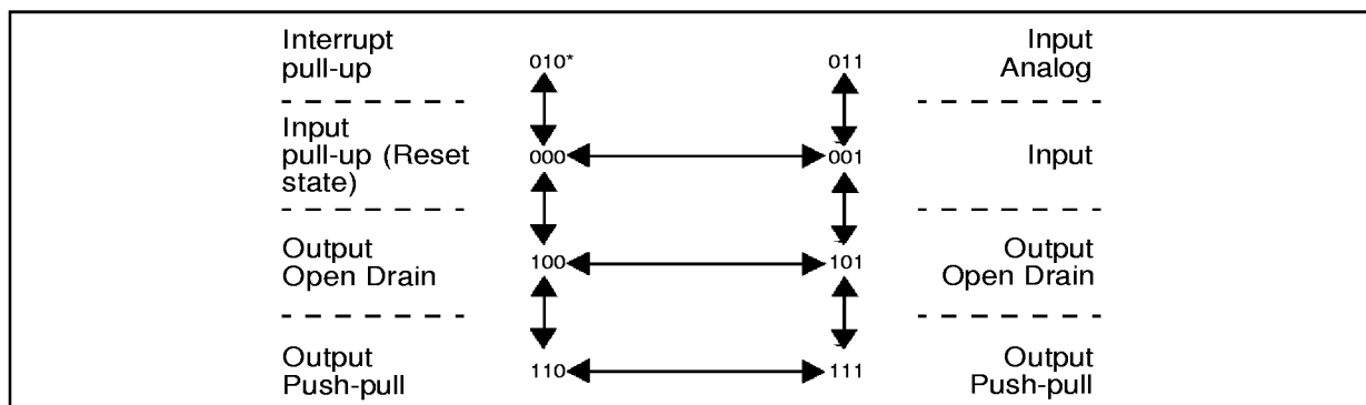
Figure 19. Diagram showing Safe I/O State Transitions
