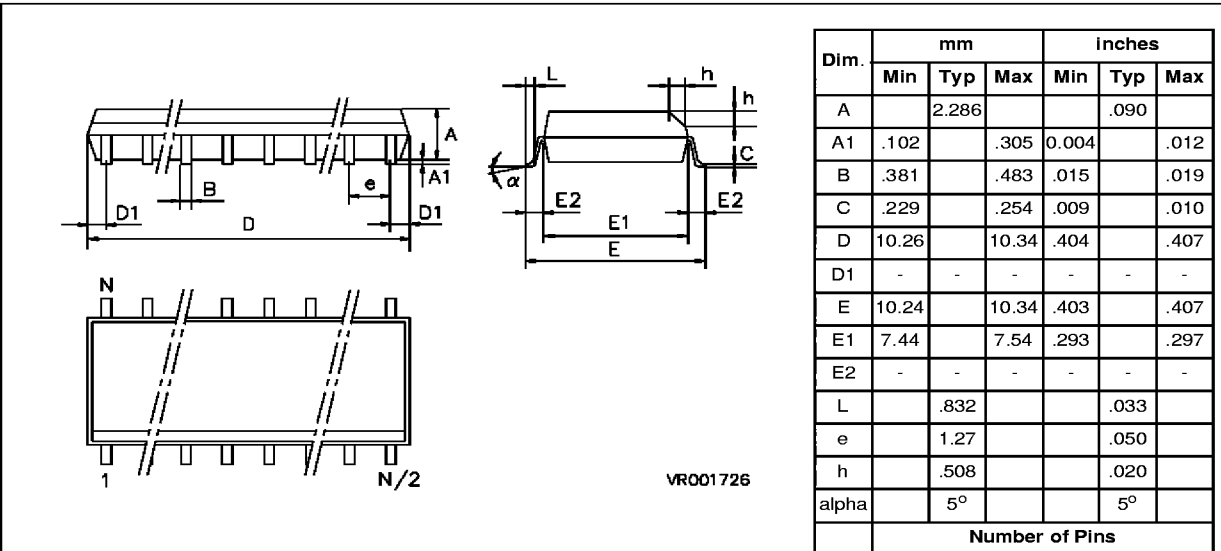
Figure 28. 16-Pin Plastic Small Outline Package (M), 300-mil Width
