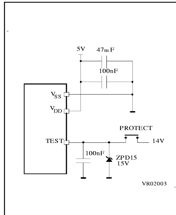
Figure 2. Programming Circuit
