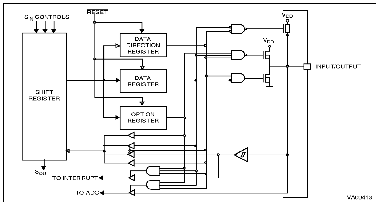
Figure 18. I/O Port Block Diagram
