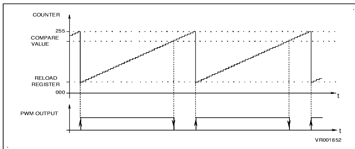
Figure 24. . Auto-reload Timer PWM Function
