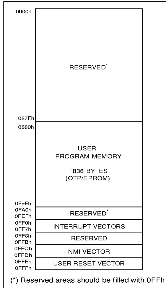
Figure 4. ST62T52B/T62B Program Memory Map
