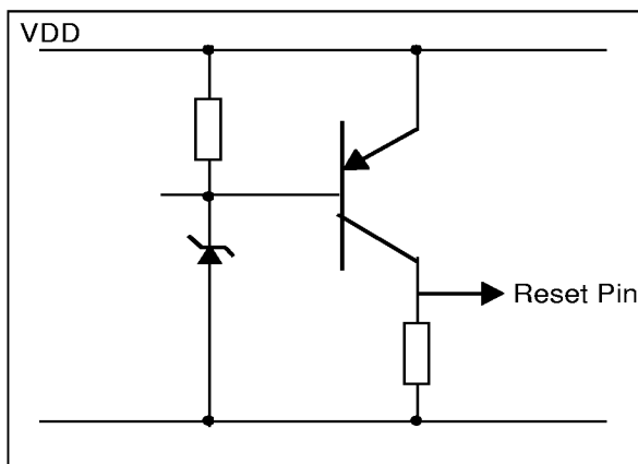
Figure 4. Reset Network
