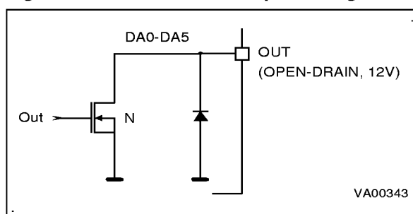
Figure 29. 6-bit PWM D/A Output Configuration
