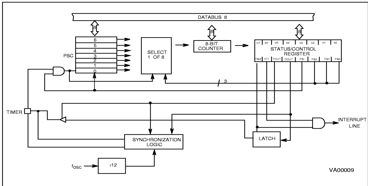
Figure 20. Timer Peripheral Block Diagram
