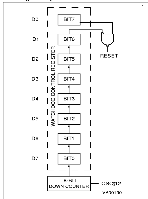
Figure 18. Hardware Activated Watchdog Working Principle
