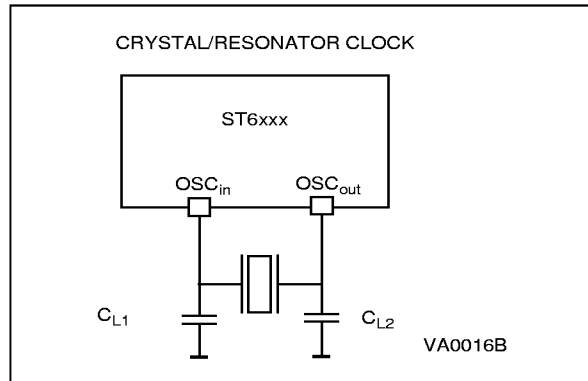
Figure 11. Clock Generator Option 2
