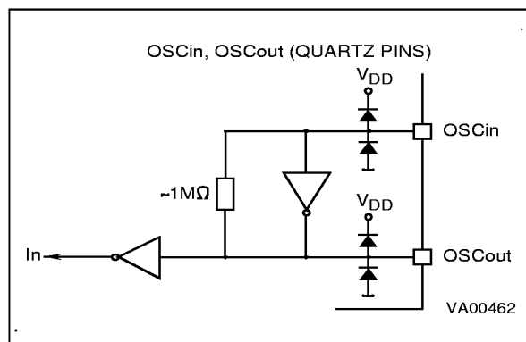
Figure 12. OSCin, OSCout Diagram
