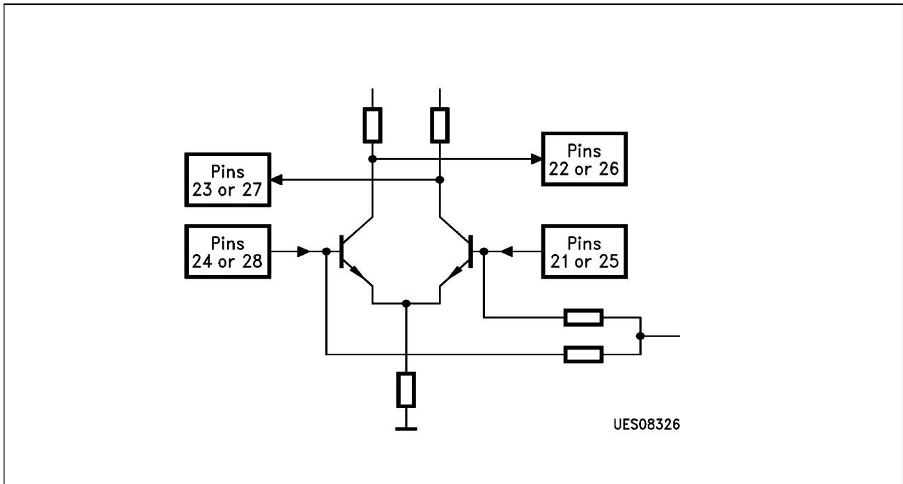
Figure 14 Equivalent I/O-Schematic of UHF- VHF-Oscillator Pins
