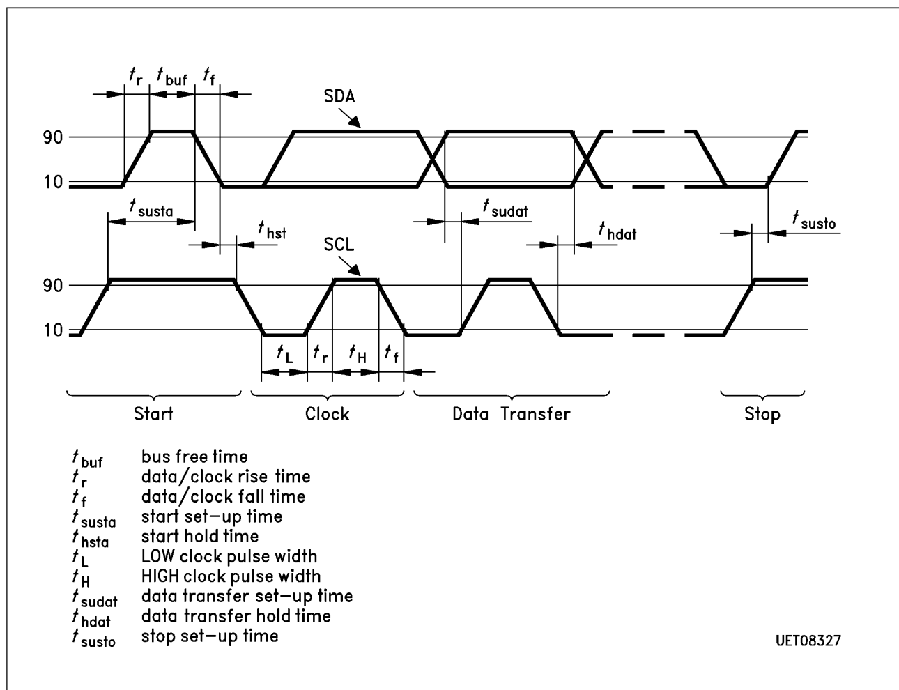
Figure 15 I²C Bus Timing
