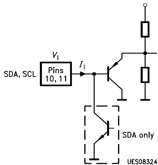
Figure 12 Equivalent I/O-Schematic of SDA/SCL Pins
