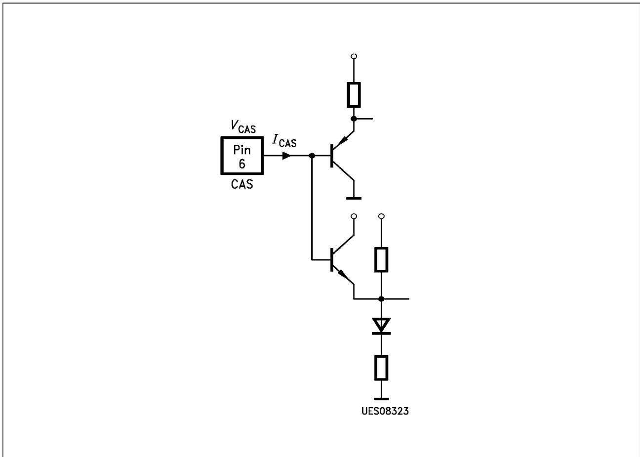
Figure 11 Equivalent I/O-Schematic of CAS Pin
