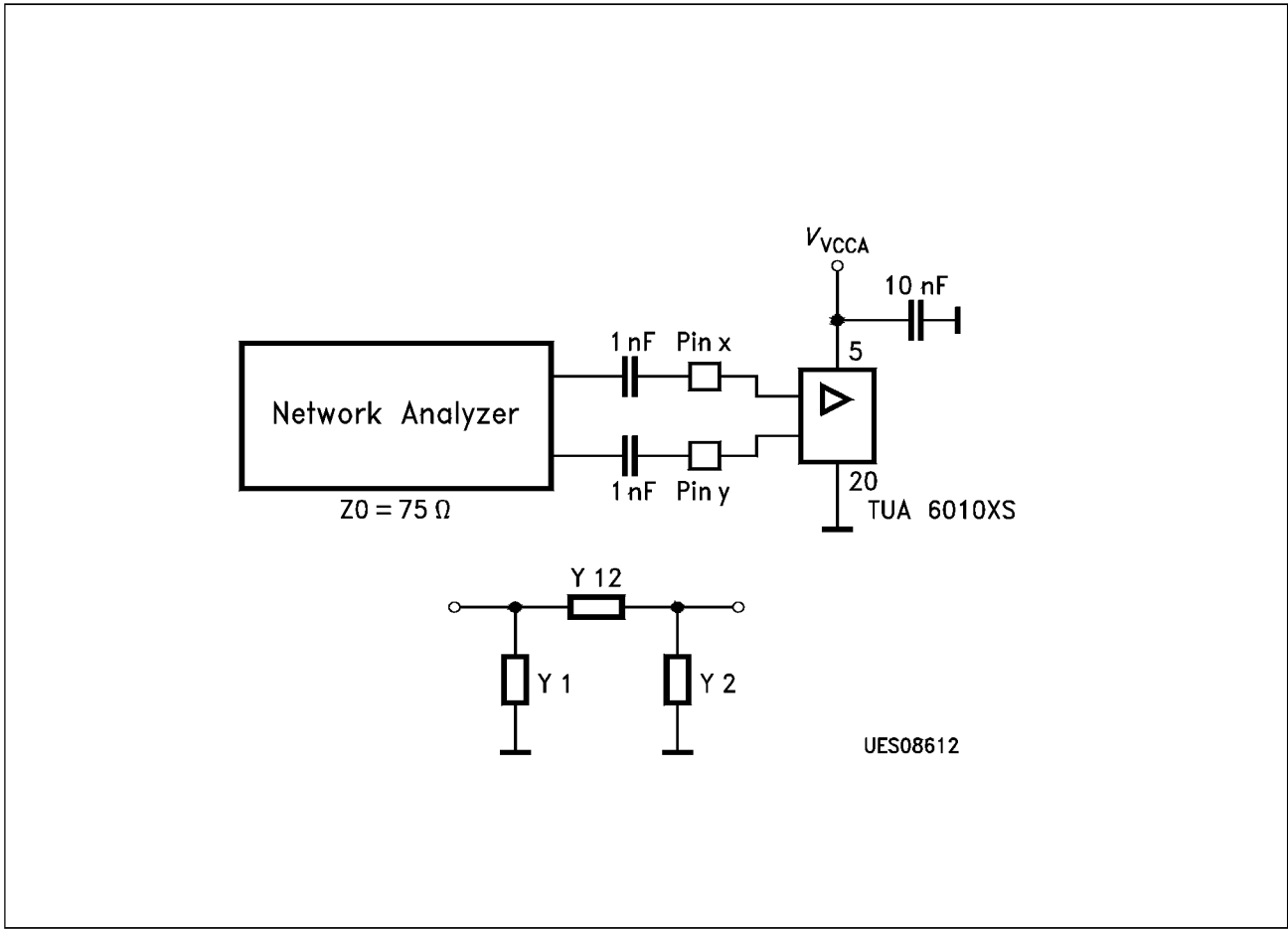
Figure 6 Measurement of S-Parameters S11, S12, S21, S22 and Calculation of \pi -Equivalent Circuit
