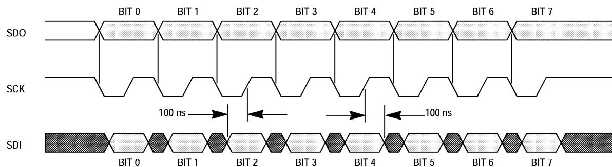
Figure 7-2. SIOF Timing Diagram
