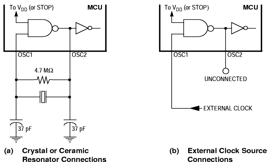
Figure 1-2. Oscillator Connections
