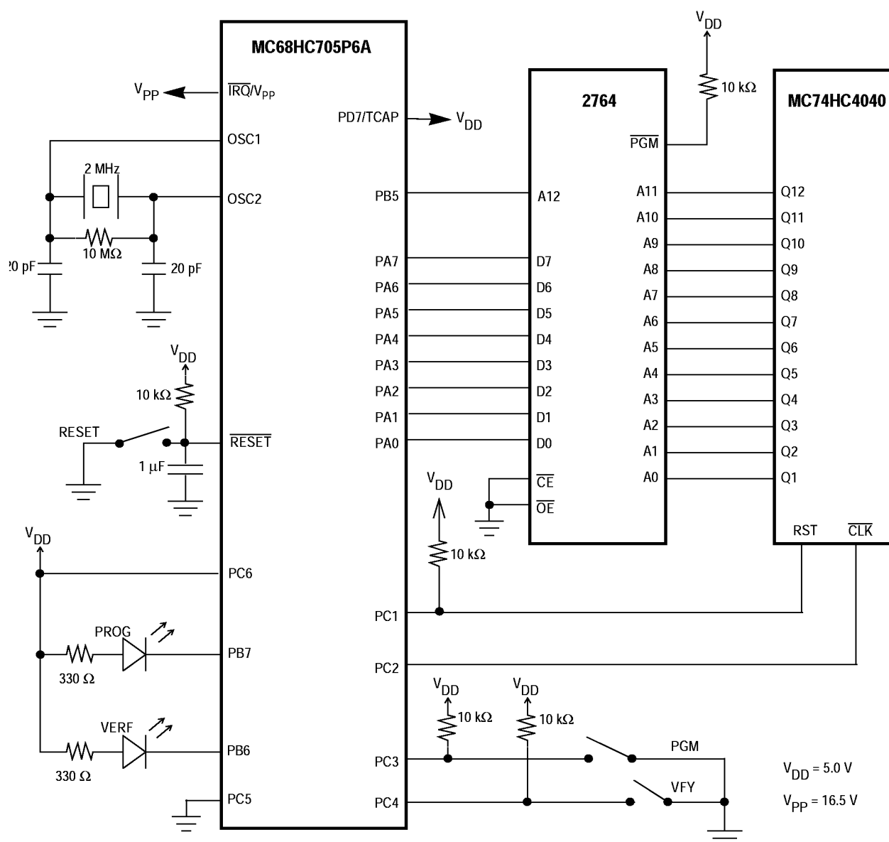
Figure 10-3. MC68HC705P6A EPROM Programming Schematic Diagram
