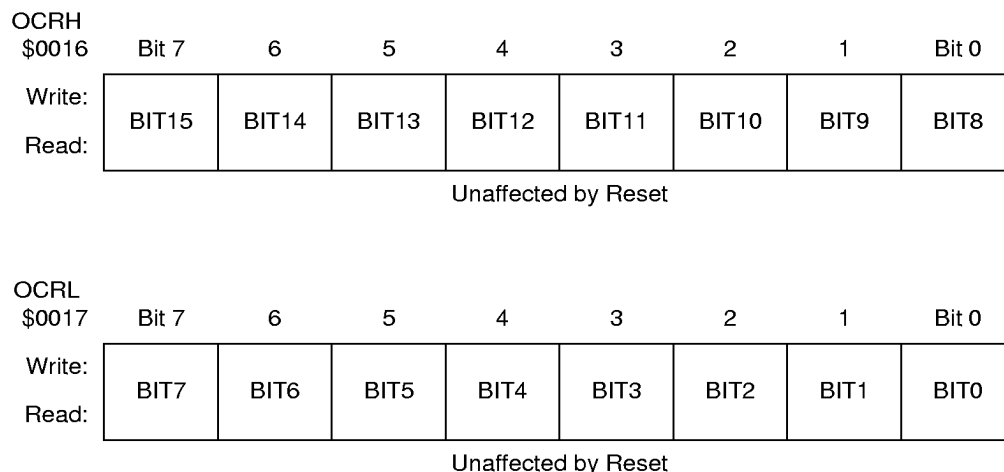
Figure 8-7. Output Compare Registers (OCRH and OCRL)
