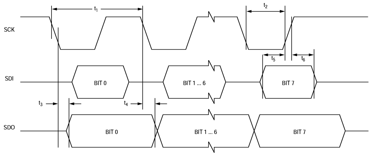
Figure 14-1. SIOPTiming Diagram
