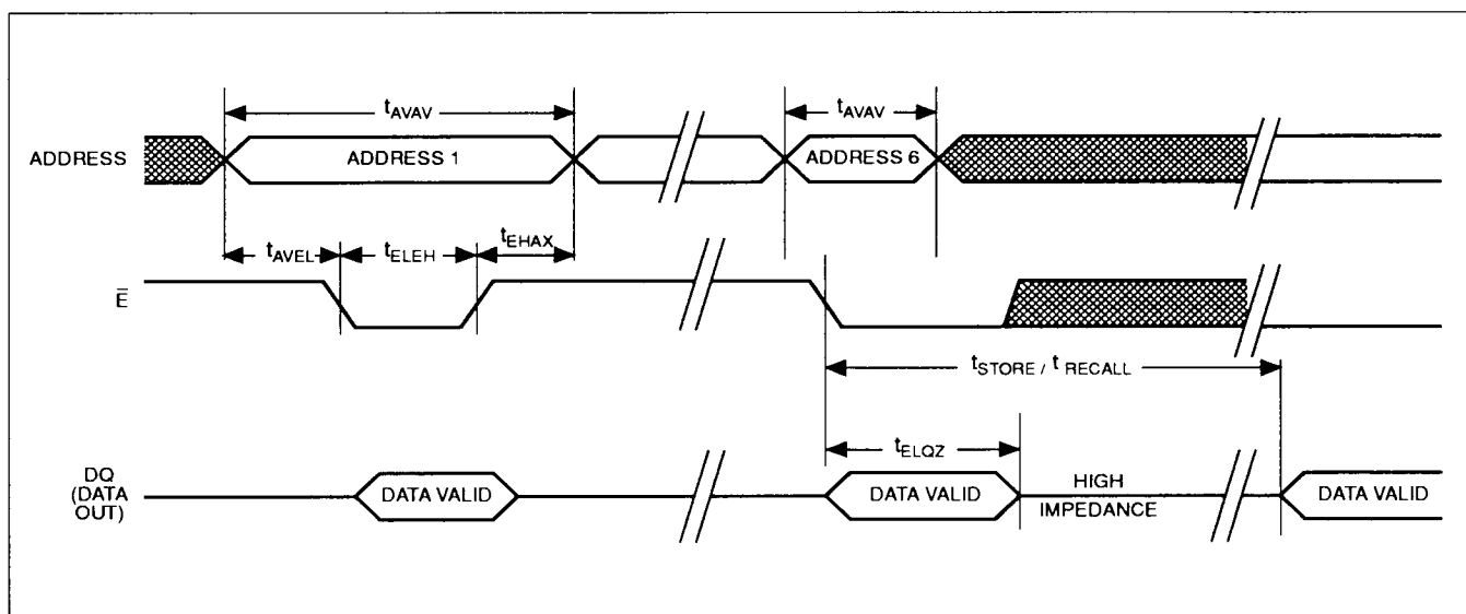
Figure 15. STORE/RECALL cycle 2. E (bar) controlled timing diagram (see notes 23, 26 and 28).
