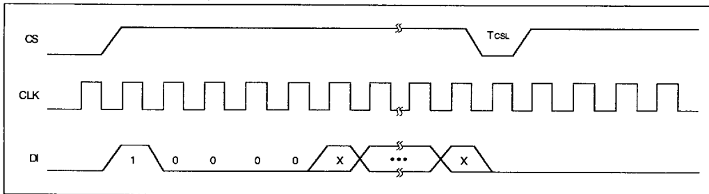
FIGURE 2-5: WRITE TIMING
