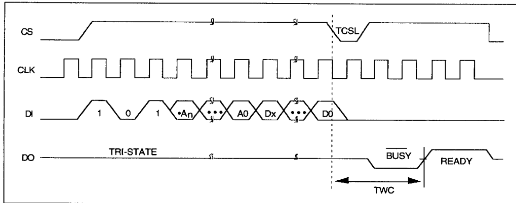
FIGURE 2-5: WRITE TIMING
