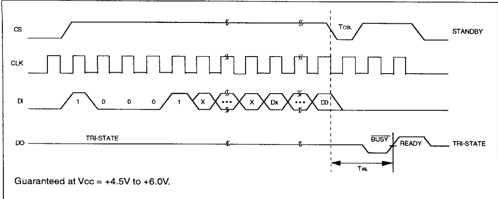
FIGURE 2-7: ERASE TIMING
