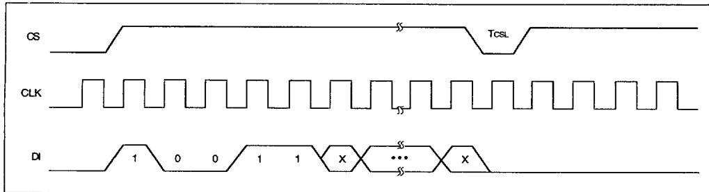
FIGURE 2-4: EWDS TIMING
