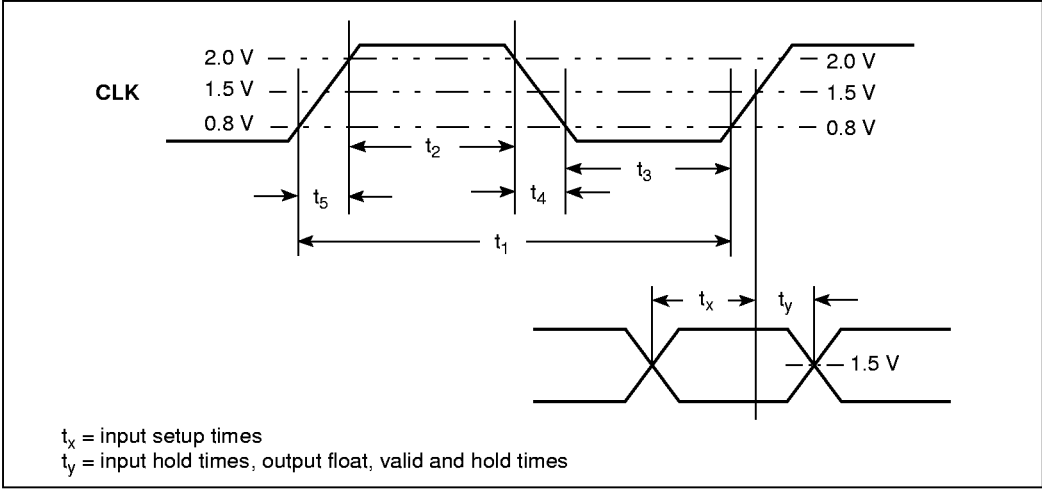
Figure 4. CLK Waveform
