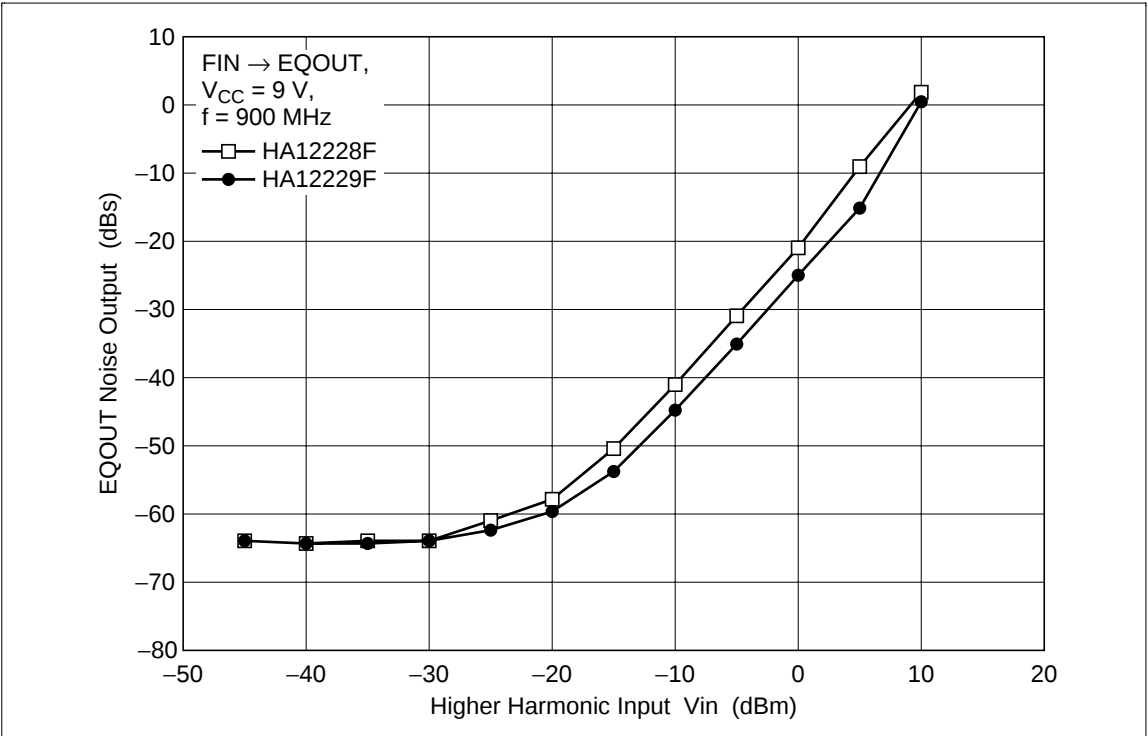
Figure 9 EQOUT Noise Output vs. Transmission Signal Input Level Characteristic
