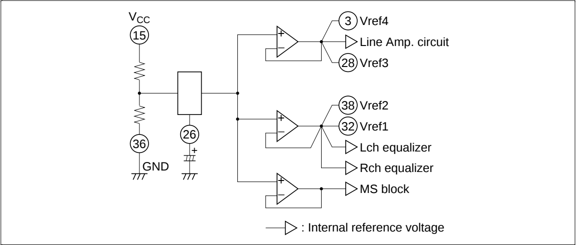
Figure 1b The HA12229F Block Diagram of Reference Supply Voltage
