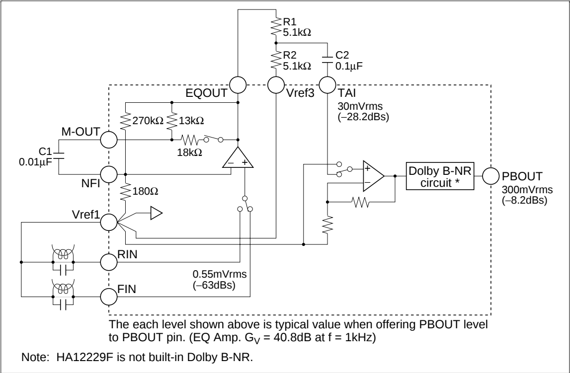
Figure 3 Input Block Diagram
