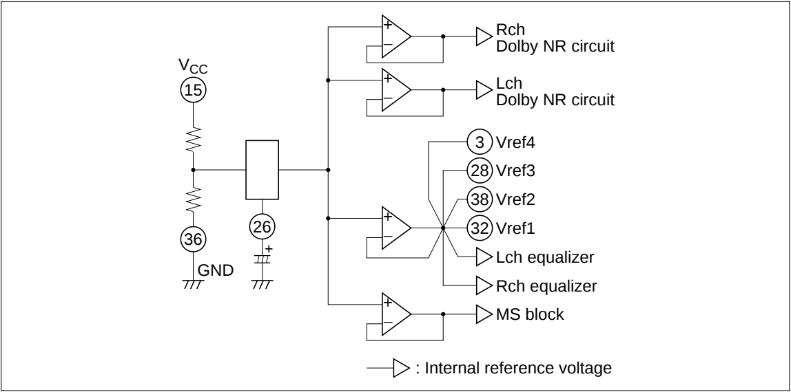
Figure 1a The HA12228F Block Diagram of Reference Supply Voltage
