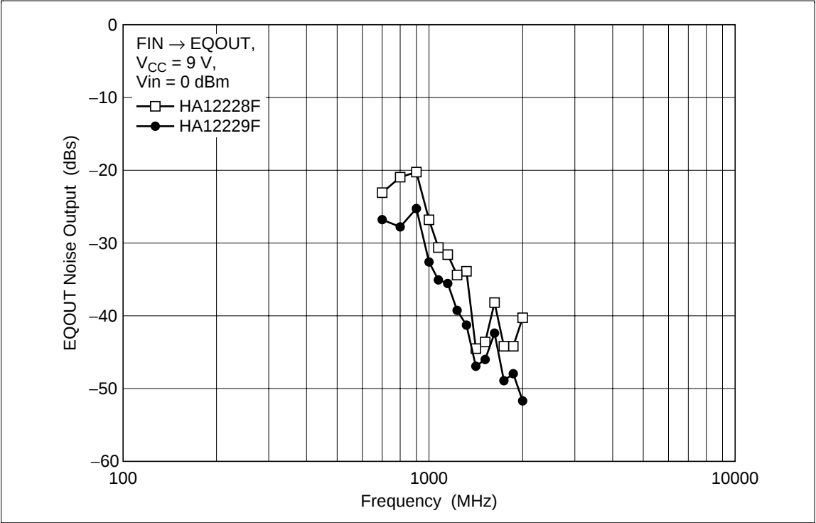
Figure 8 EQOUT Noise Output vs. Transmission Frequency Characteristic
