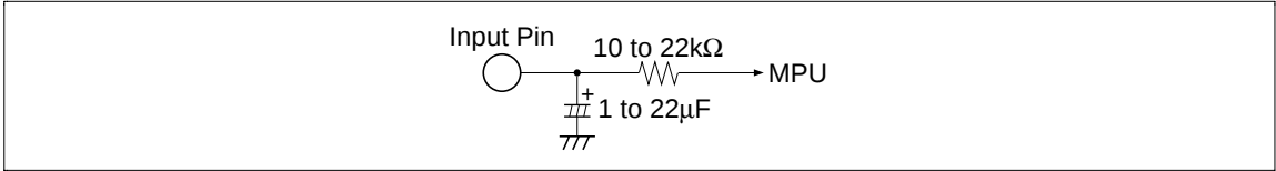
Figure 2 Interface for Reduction of Pop Noise
