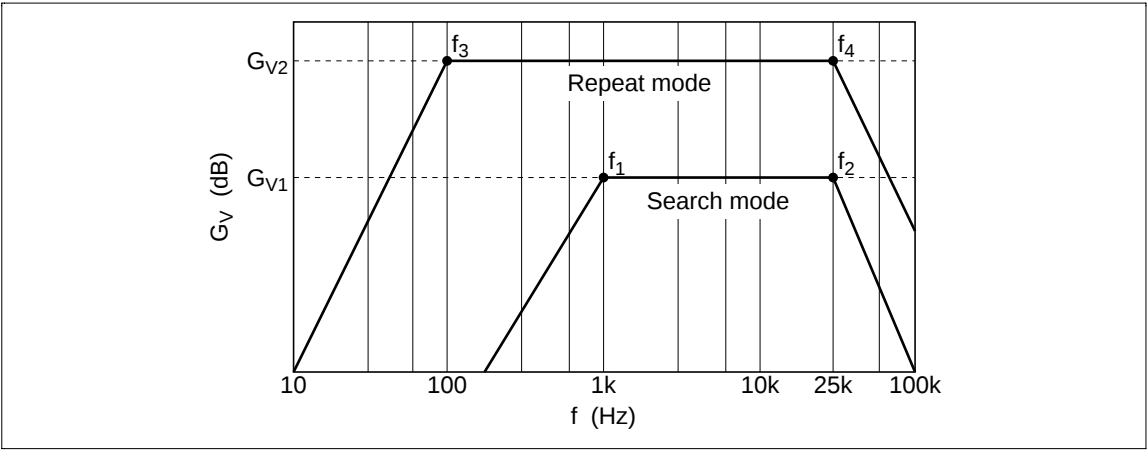
Figure 5 Frequency Response
