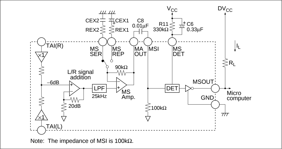
Figure 4 Music Sensor Block Diagram
