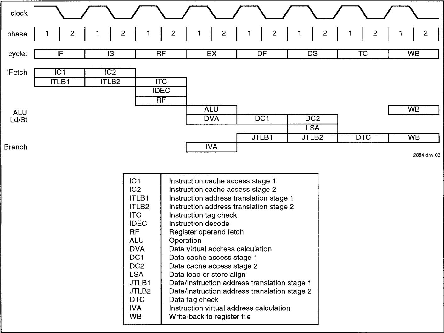
Figure 2. Pipeline Activities
