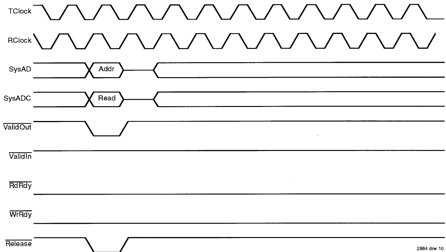
Figure 9. Processor Read Request
