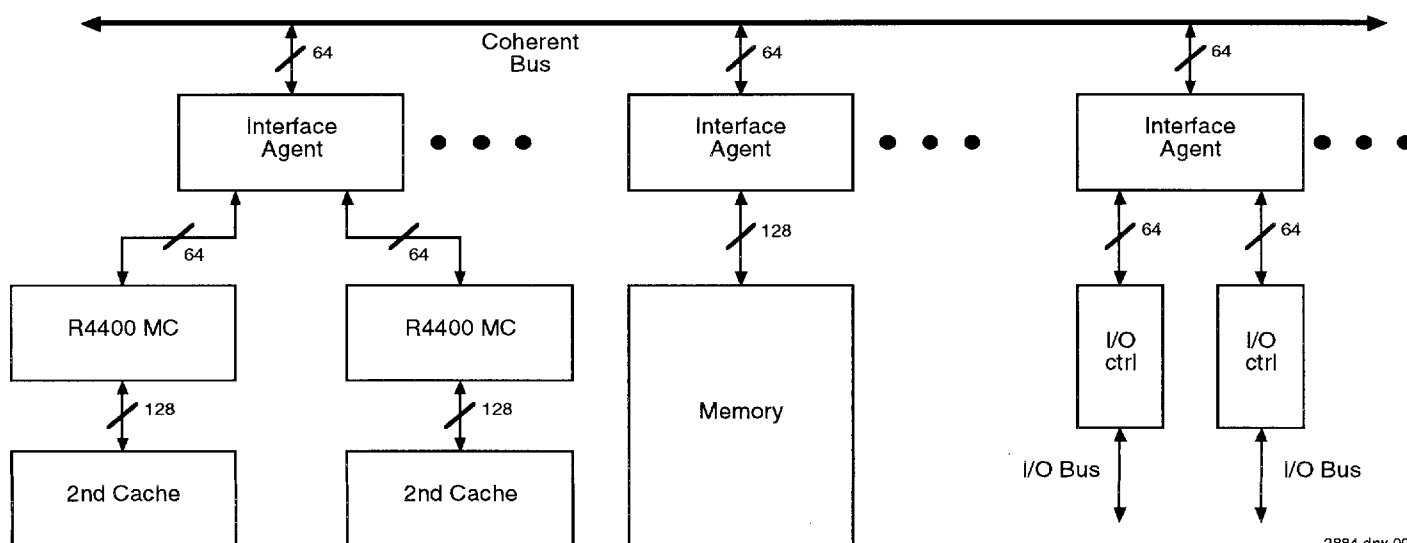
Figure 8. Multiprocessor System Using the R4400 MC
