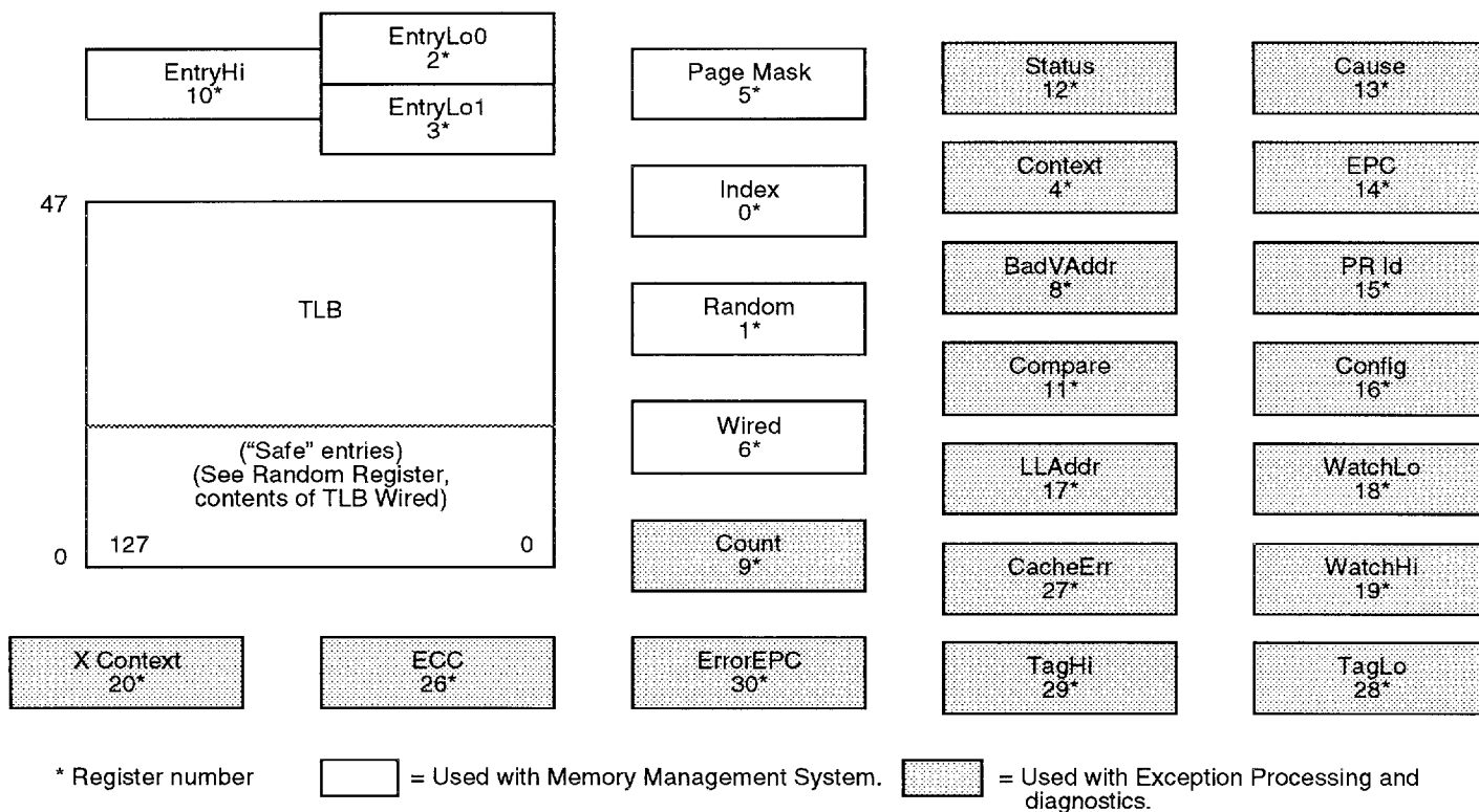
CP0 and the TLB
