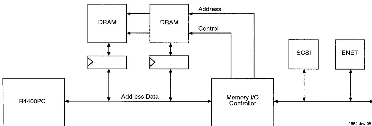
Figure 7. Typical Desktop System Block Diagram
