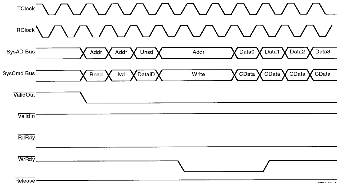
Figure 10. Processor Read, Invalidate, Write Request
