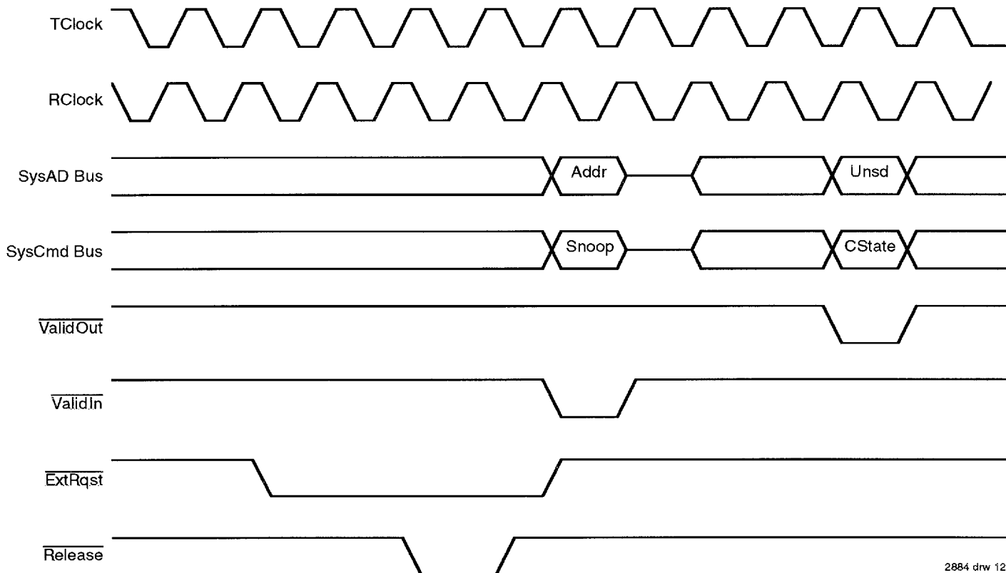
Figure 11. External Snoop Request
