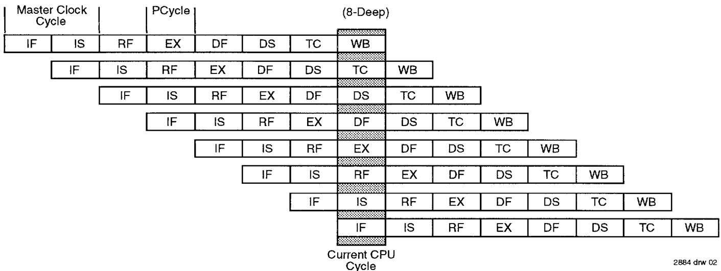
Figure 1. R4400 8-Stage Super-Pipeline
