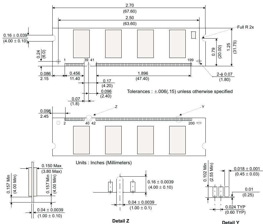
Figure 1: KVR400X64SC3A/256 200-Pin SODIMM
