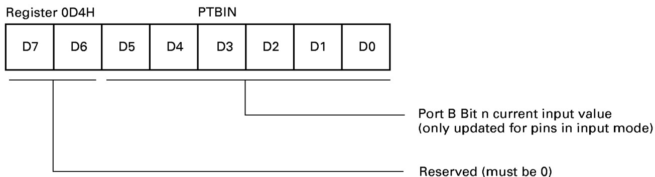
Figure 38. Port B Input Value Register
