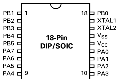
Figure 3. 18-Pin DIP/SOIC Pin Identification
