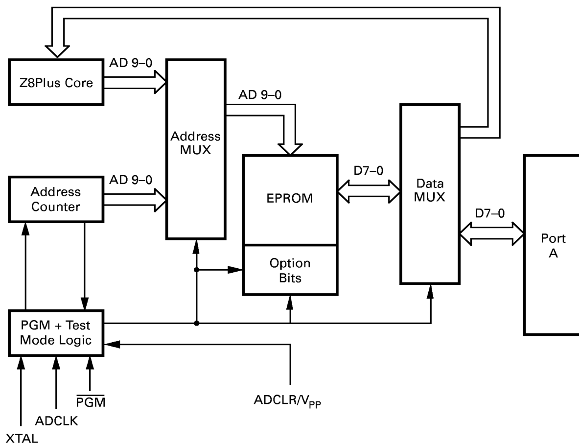
Figure 2. EPROM Programming Mode Block Diagram
