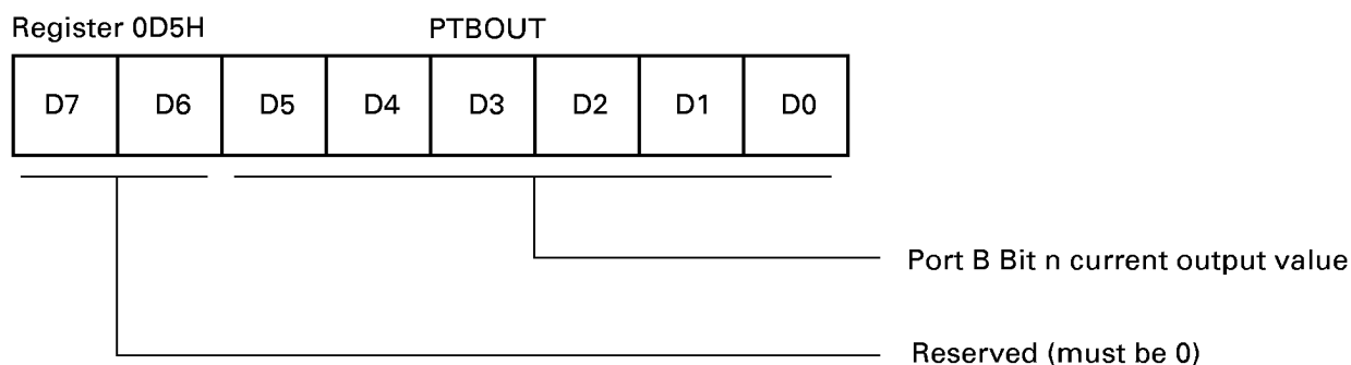
Figure 39. Port B Output Value Register
