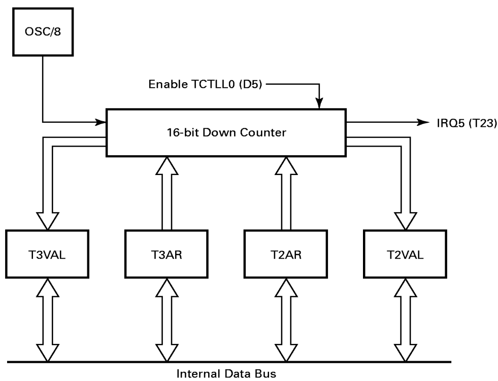
Figure 19. 16-Bit Standard Timer
