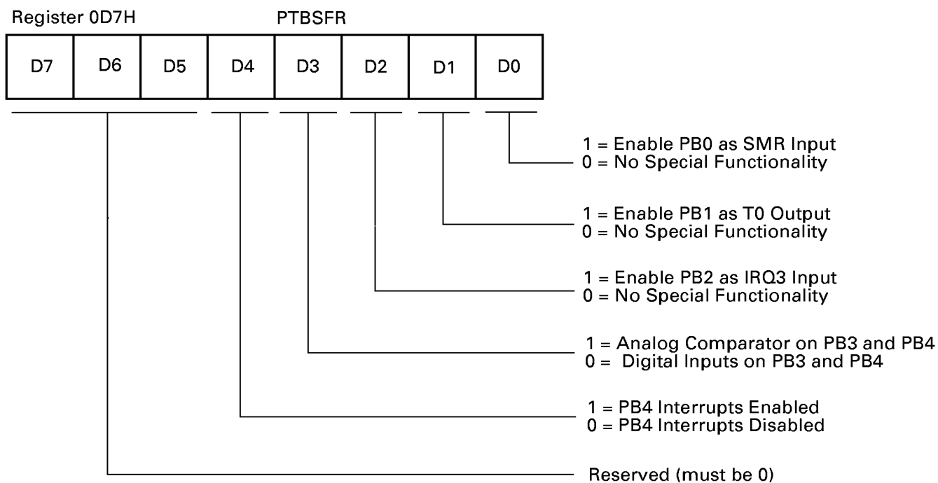
Figure 41. Port B Special Function Register
