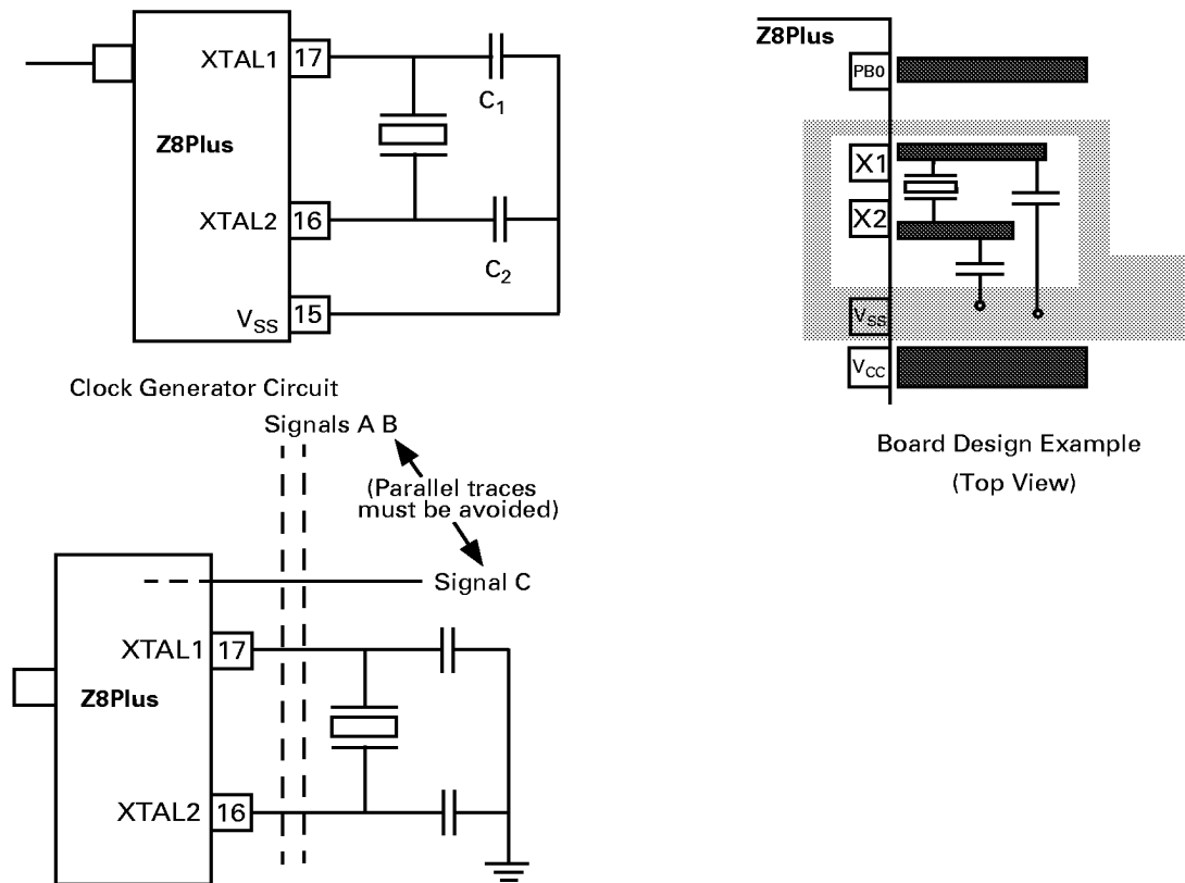
Figure 15. Circuit Board Design Rules
