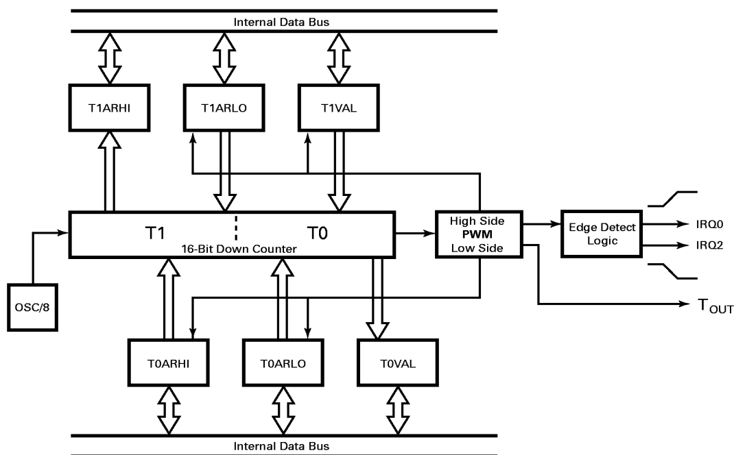
Figure 21. 16-Bit Standard PWM Timer
