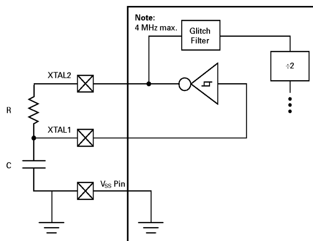
Figure 13. Z8Plus in RC Oscillator Mode
