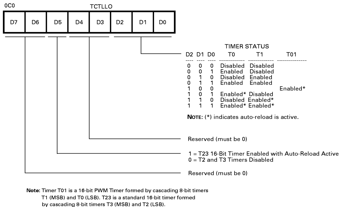
Figure 22. TCTLLO Register
