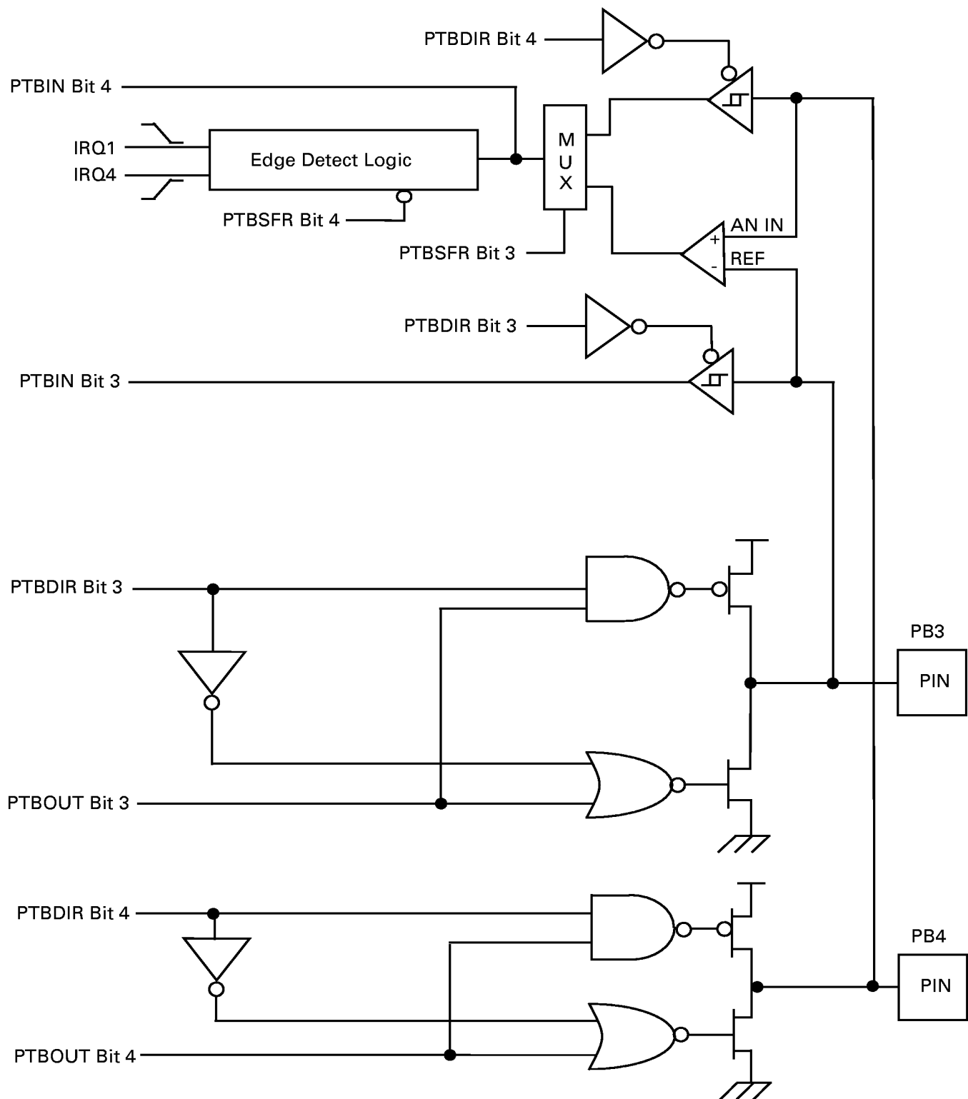
Figure 37. Port B Pins 3 and 4 Diagram
