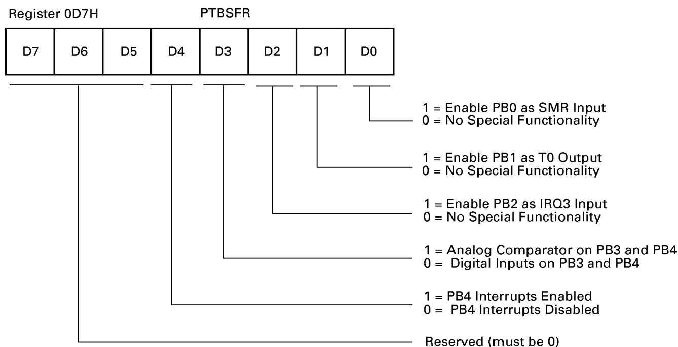
Figure 32. Port B Special Function Register
