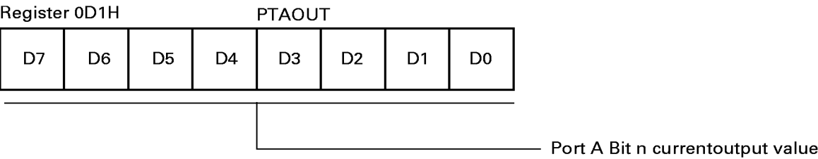
Figure 29. Port A Output Value Register
