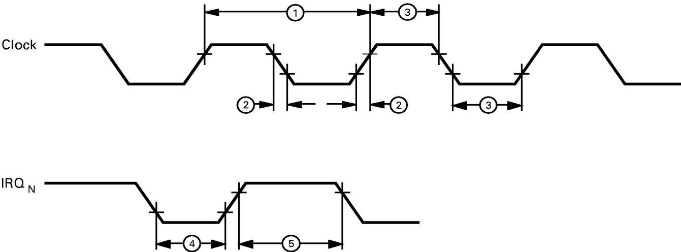
Figure 8. AC Electrical Timing Diagram
