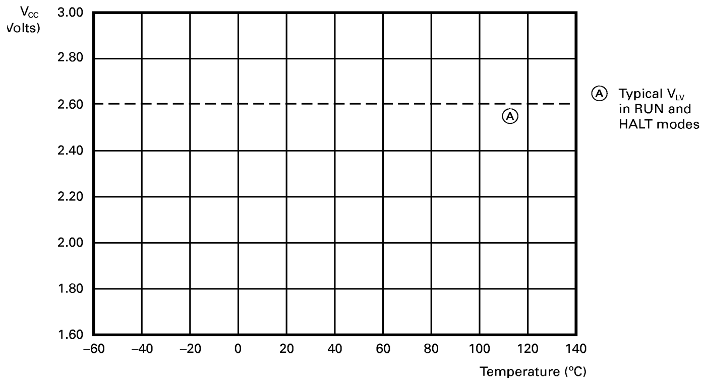
Figure 42. Voltage vs. Temperature
