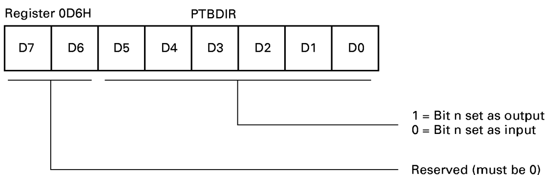
Figure 40. Port B Directional Control Register
