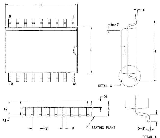
Figure 46. 18-Pin SOIC Package Diagram
