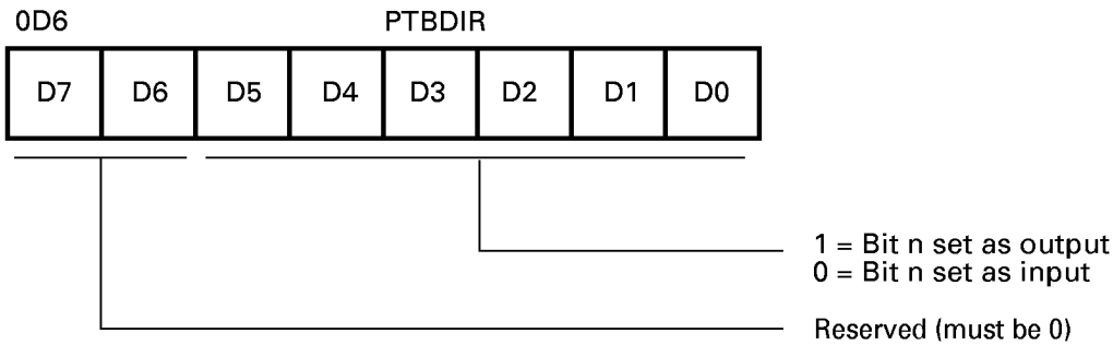
Figure 24. Port B Directional Control Register
