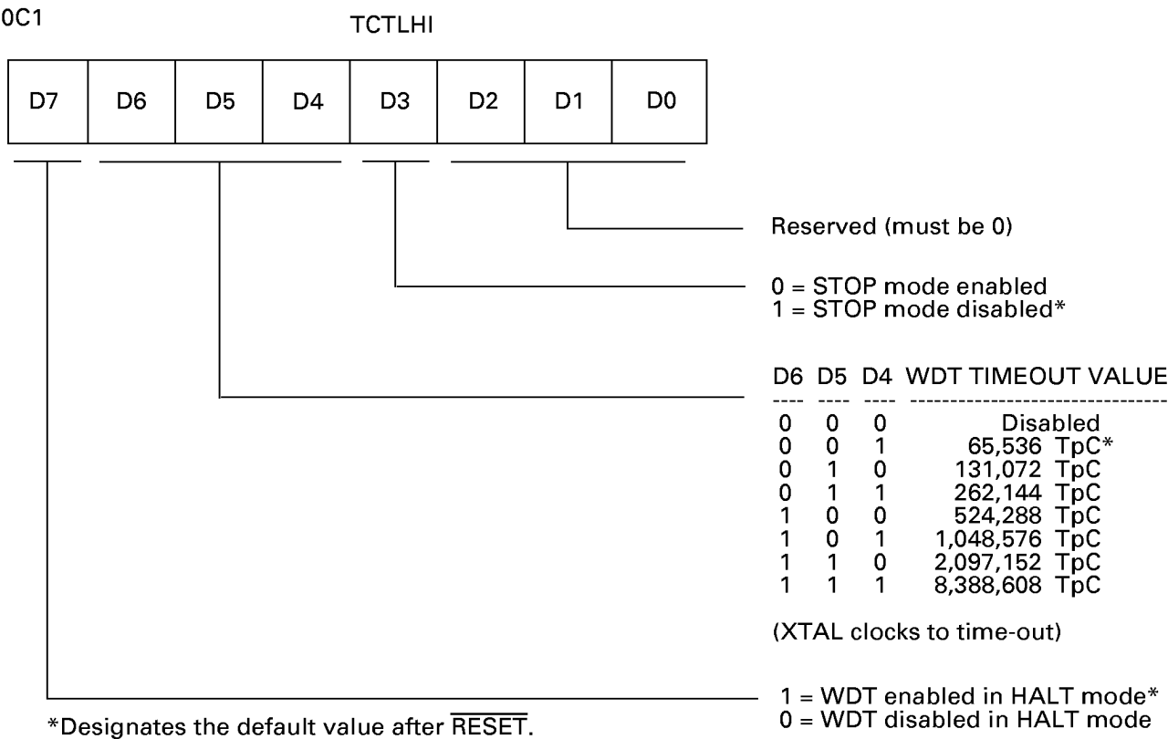
Figure 11. TCTLHI Register for Control of WDT
