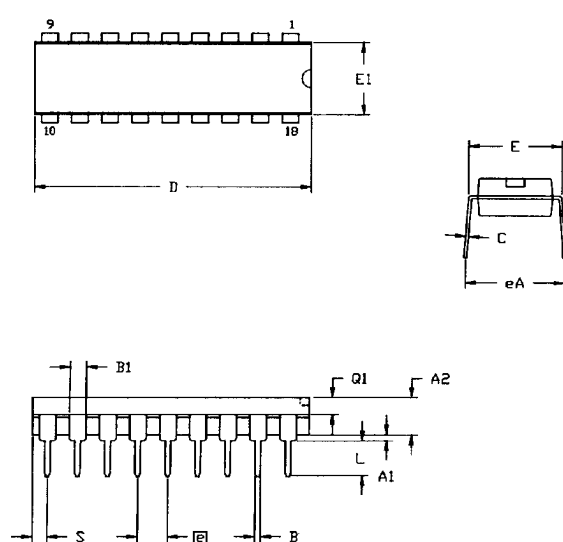
Figure 45. 18-Pin DIP Package Diagram
