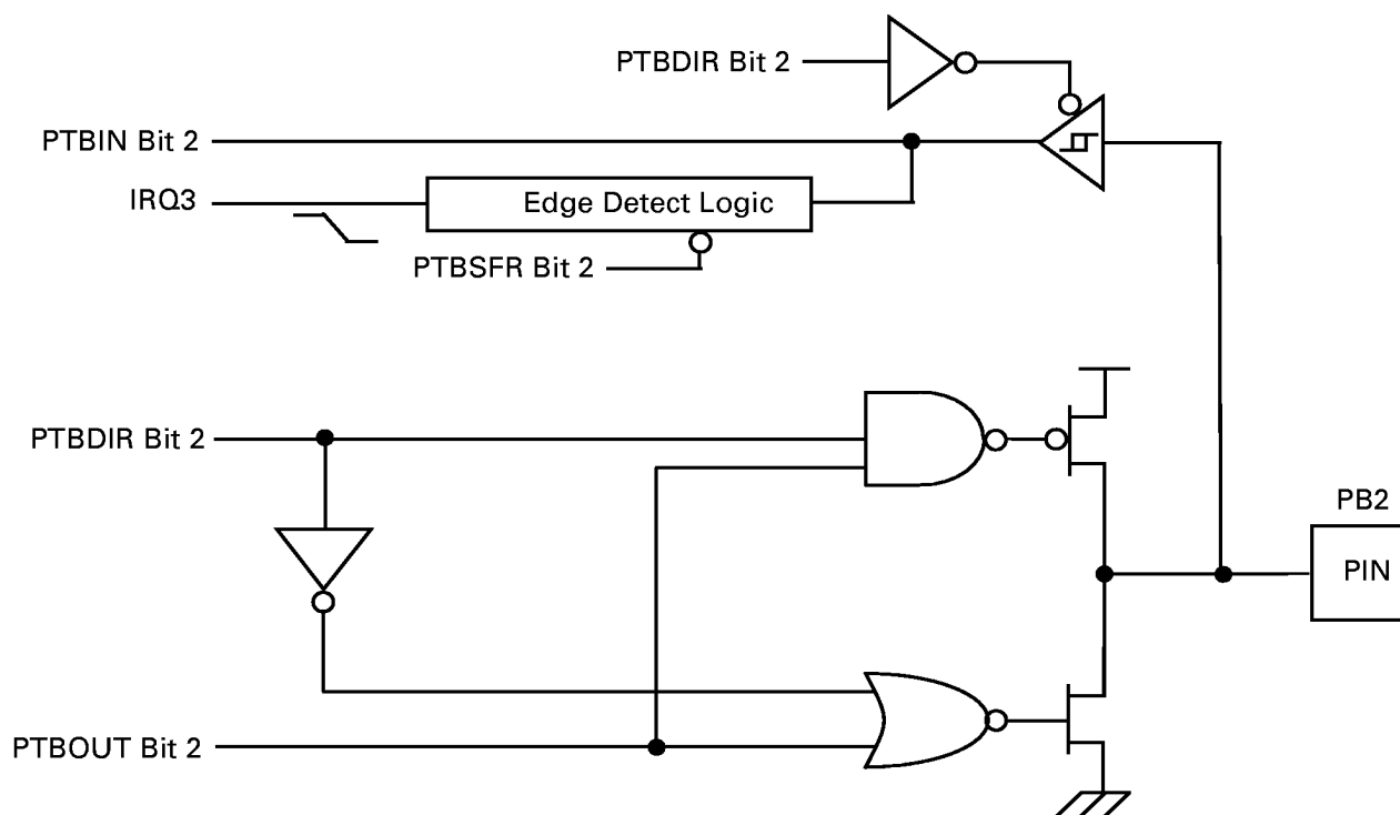
Figure 36. Port B Pin 2 Diagram
