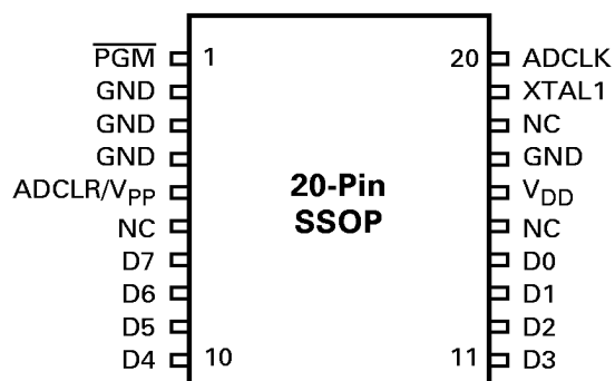
Figure 6. 20-Pin SSOP Pin Identification/EPROM Programming Mode
