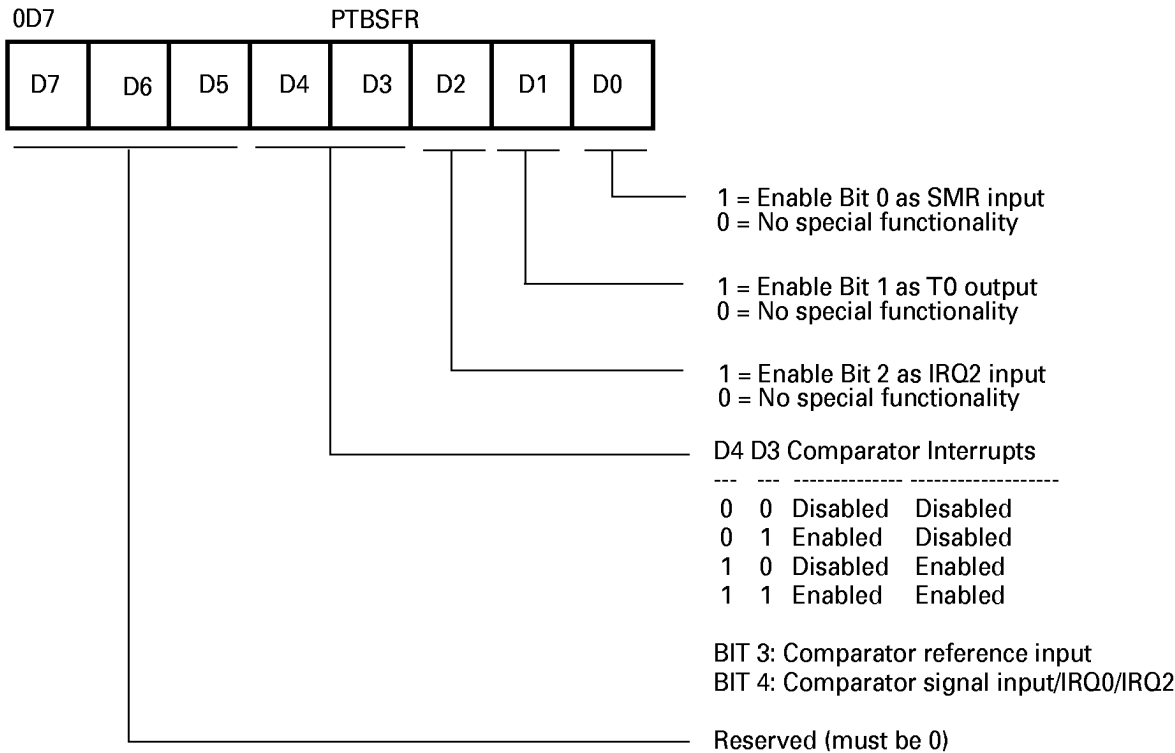
Figure 23. PortB Special Function Register
