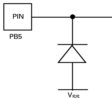
Figure 44. PB5 Pin Input Protection
