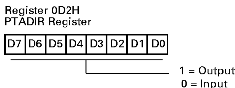
Figure 27. Port A Directional Control Register
