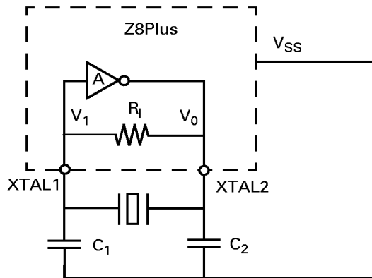
Figure 14. Pierce Oscillator with Internal Feedback Circuit
