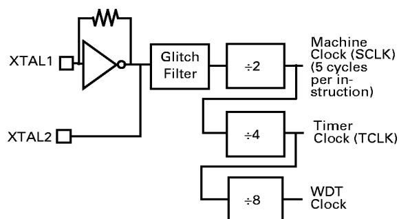
Figure 12. Clock Circuit
