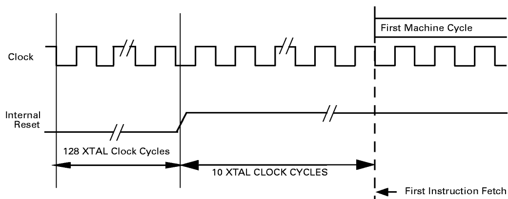
Figure 9. Reset Timing
