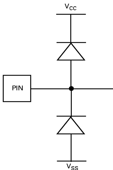
Figure 43. I/O Pin Diode Input Protection
