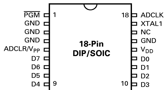
Figure 4. 18-Pin DIP/SOIC Pin Identification
