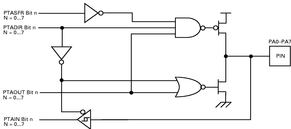
Figure 26. Port A Configuration with Open-Drain Capability and Schmitt-Trigger
