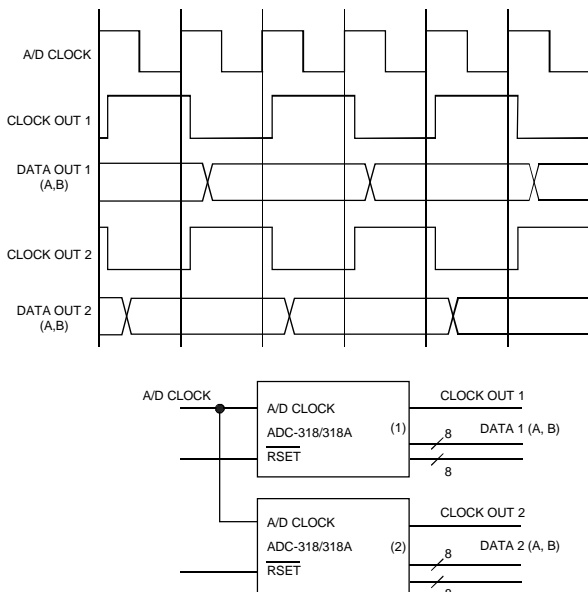
Figure 3-3: Parallel Operation without RSET Pulse
