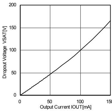
Fig. 10 Dropout Voltage vs Output Current (BH28RB1WGUT)
