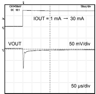
Fig. 20 Load Response (Co = 1.0 µF) (BH33RB1WGUT)
