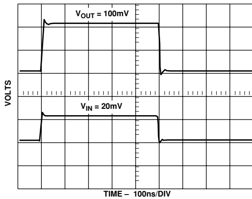
Figure 4. 100 mV Step Response; G = +5 , V_S = \pm 6 V, R_L = 25 \Omega , Single-Ended
