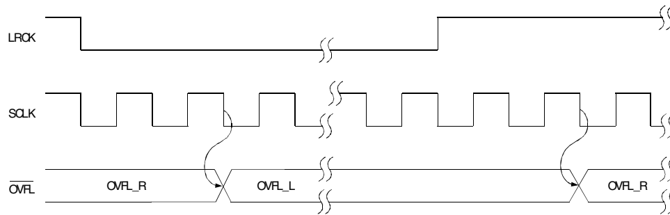
Figure 20. \overline{\text{OVFL}} Output Timing, I 2 S Format
