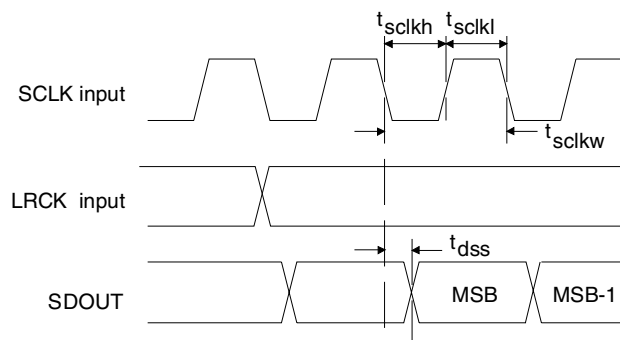
Figure 16. Slave Mode, I 2 S SAI
