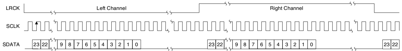
Figure 19. I 2 S Serial Audio Interface
