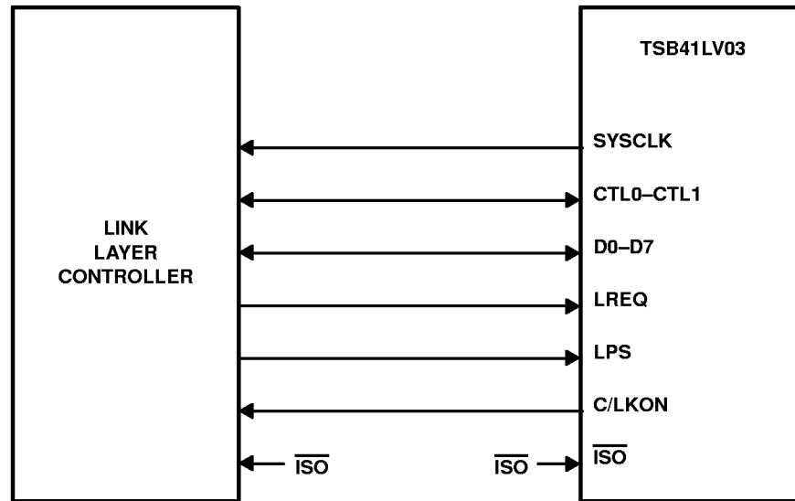
Figure 10. PHY-LLC Interface
