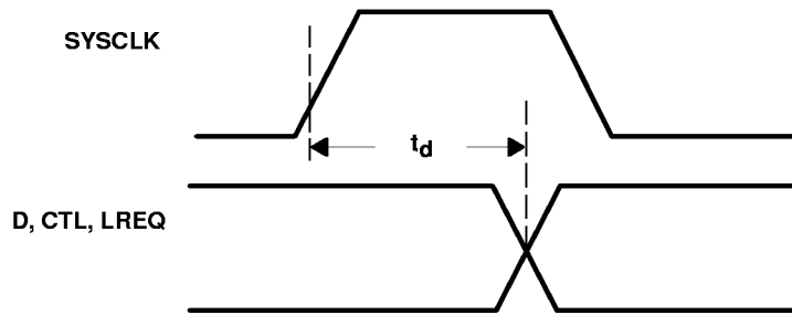
Figure 3. D and CTL Output Delay Relative to SYSCLK Waveforms
