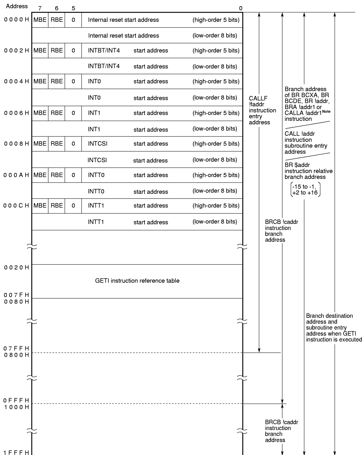
Fig. 5-3 Program Memory Map (in μPD750008)
