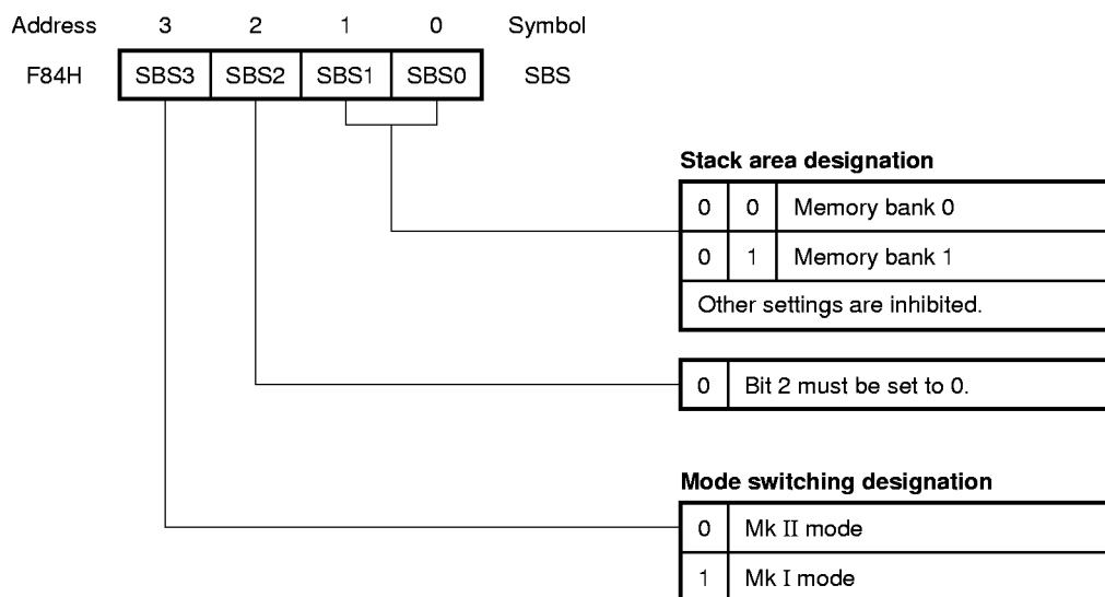
Fig. 4-1 Stack Bank Selection Register Format
