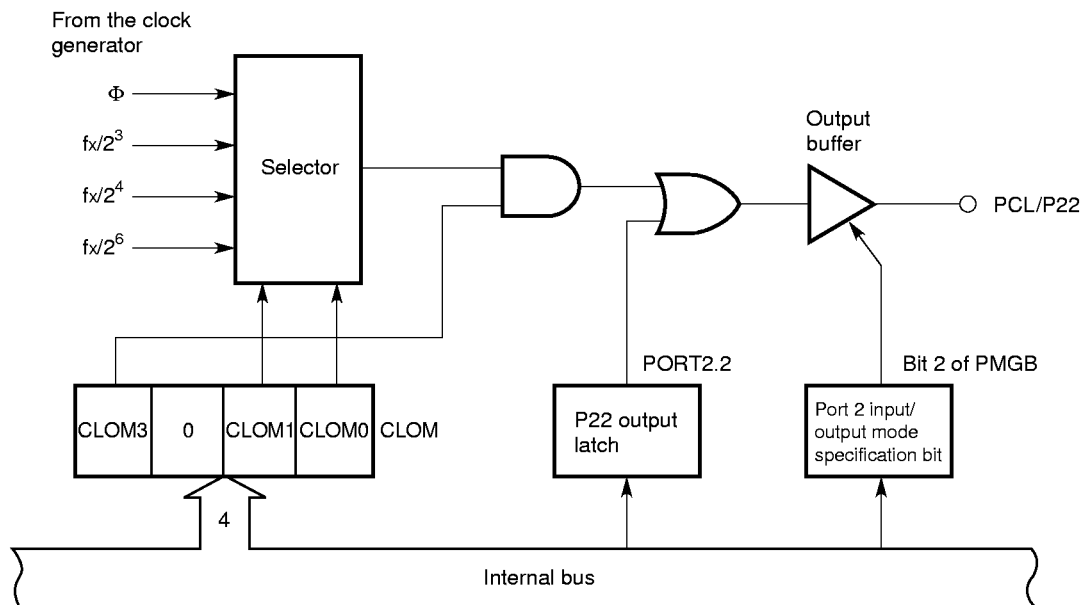
Fig. 6-3 Clock Output Circuit Configuration
