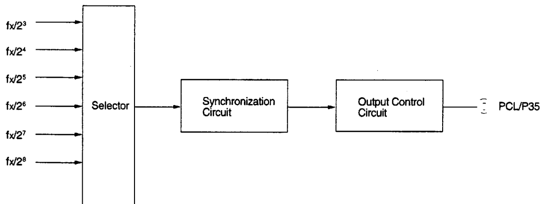
Figure 5-4. Clock Output Control Circuit Block Diagram
