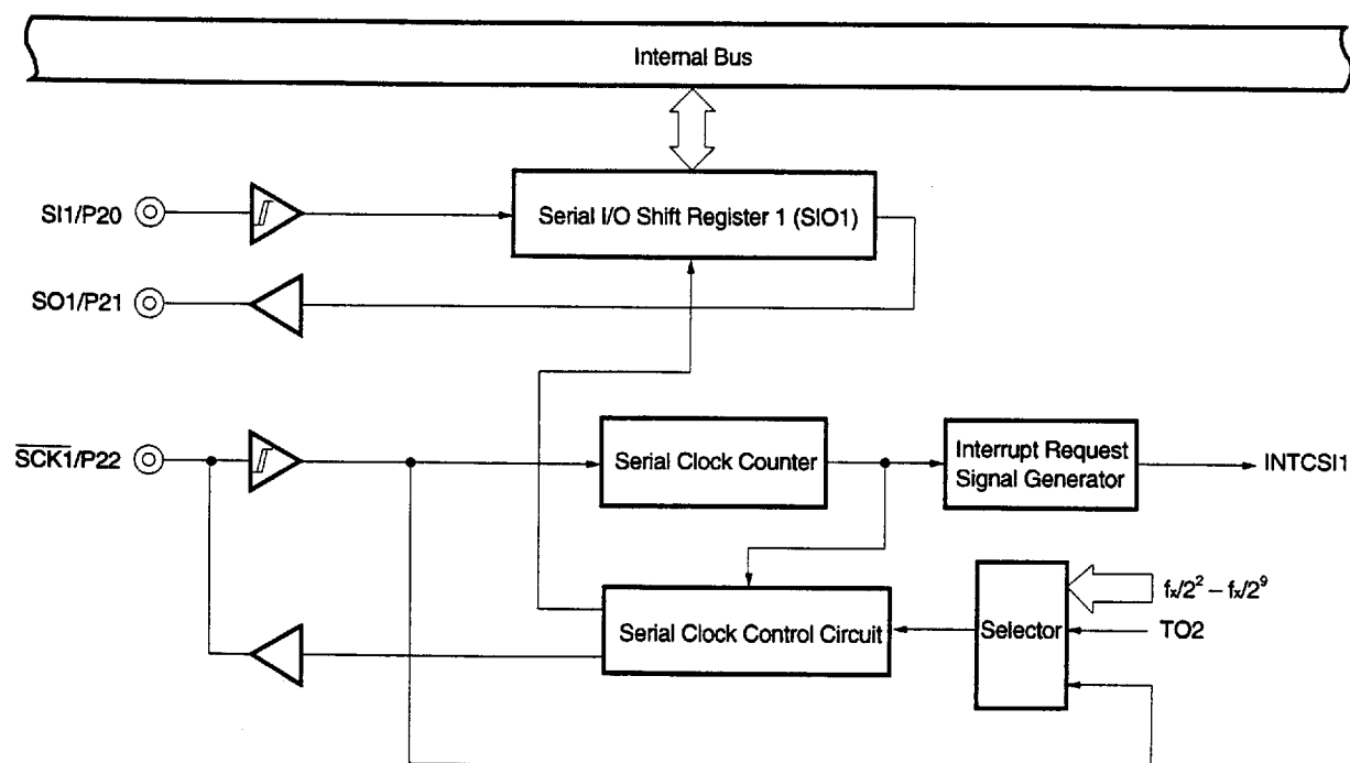
Figure 5-7. Serial Interface Channel 1 Block Diagram
