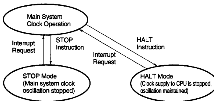
Figure 7-1. Standby Functions
