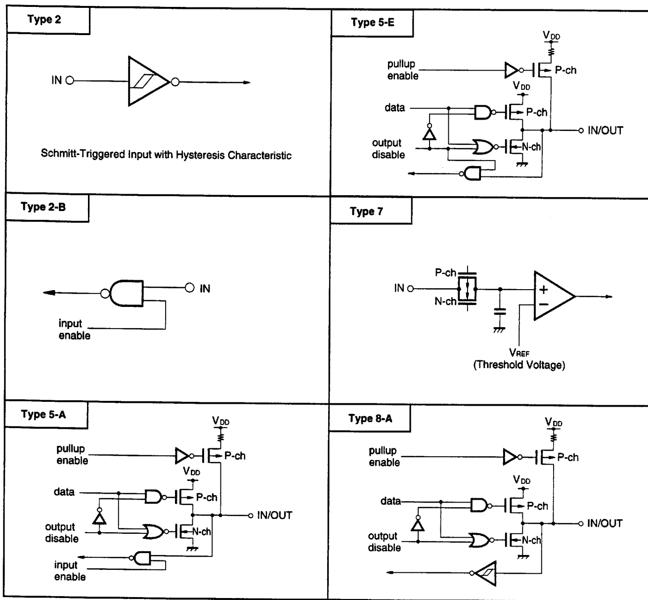
Figure 3-1. Pin Input/Output Circuits
