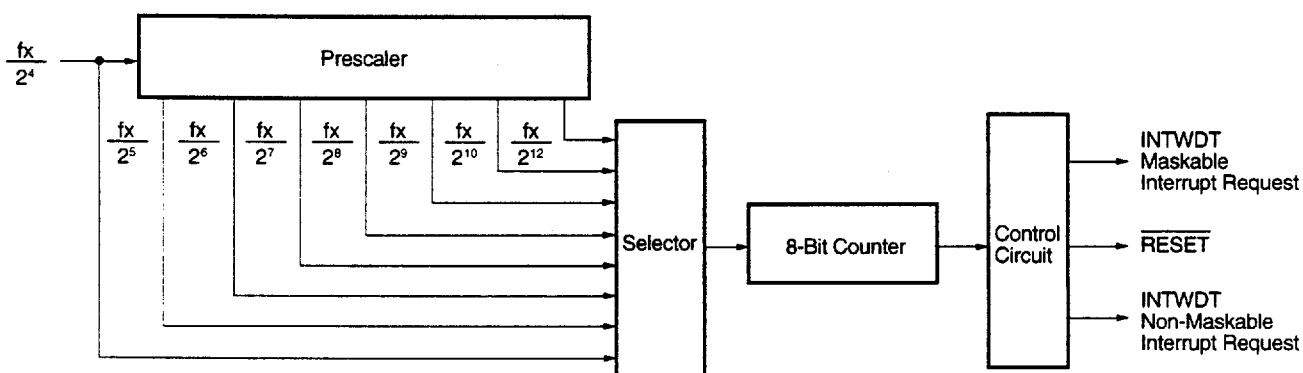
Figure 5-3. Watchdog Timer Block Diagram
