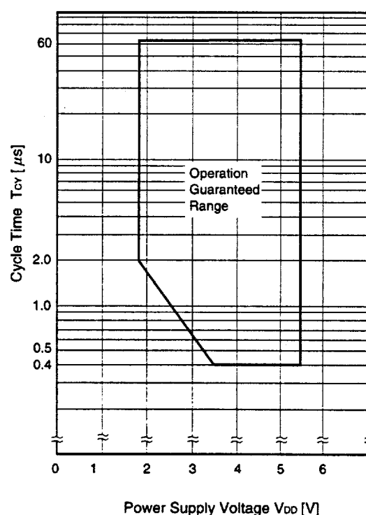
T_{CY} vs V_{DD} (Main System Clock Operation)
