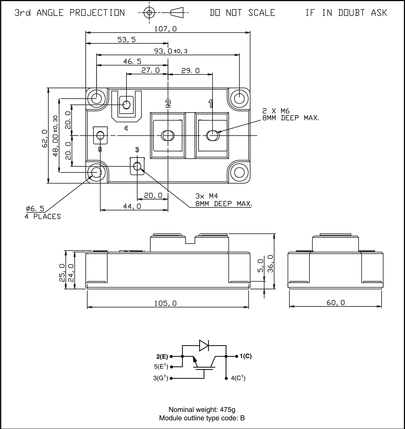
Fig. 11 Package details
