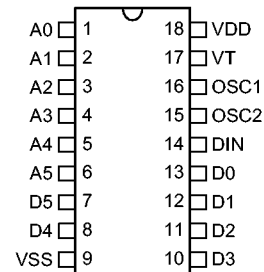
HT6072 - 18 DIP-6M
