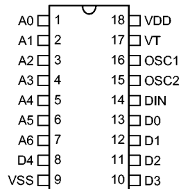
HT6072 - 18 DIP-5M
