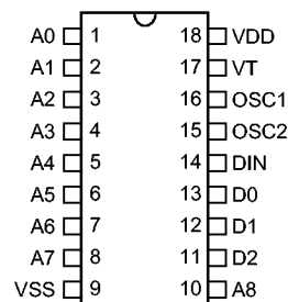
HT6072 - 18 DIP/SOP-3L
