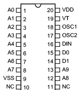
HT6072 - 20 DIP-2M
