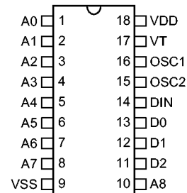
HT6072 - 18 DIP/SOP-3M
