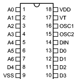
HT6072 - 18 DIP-5L
