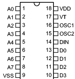
HT6072 - 18 DIP-4M
