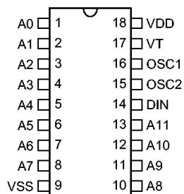
HT6072 - 18 DIP-0
