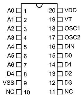
HT6072 - 20 DIP-5L
