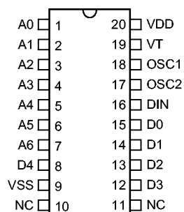
HT6072 - 20 DIP-5M
