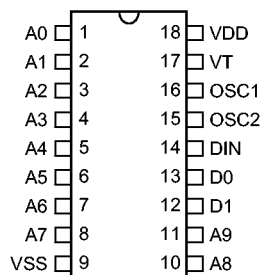
HT6072 - 18 DIP-2L
