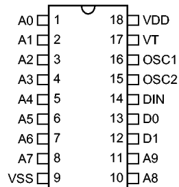
HT6072 - 18 DIP-2M
