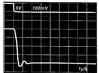
NEGATIVE SETTLING TIME ( V_{SS} = -5\text{V} )
