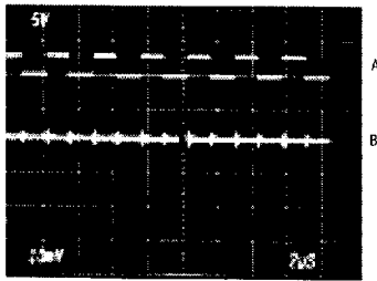
CLOCK FEEDTHROUGH
