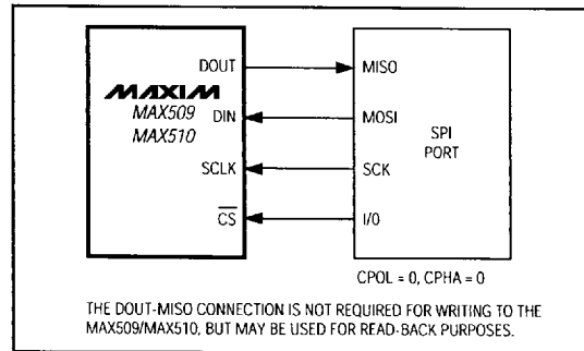
Figure 5. Connections for SPI
