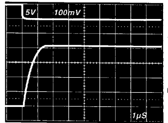
POSITIVE SETTLING TIME ( V_{SS} = \text{AGND OR } -5\text{V} )
