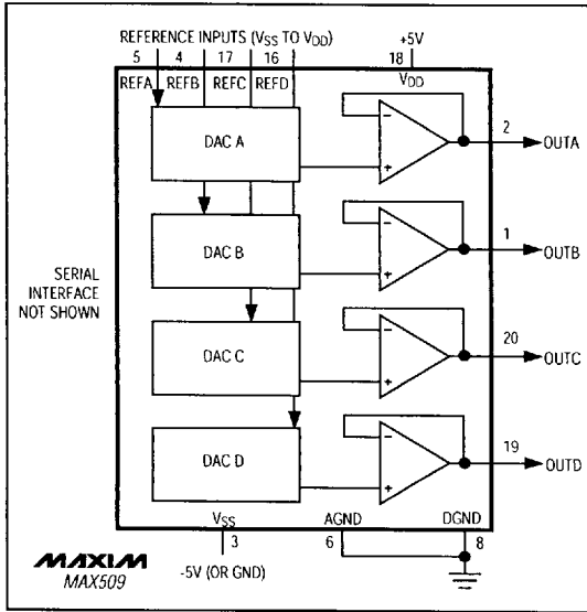
Figure 11. MAX509 Unipolar Output Circuit
