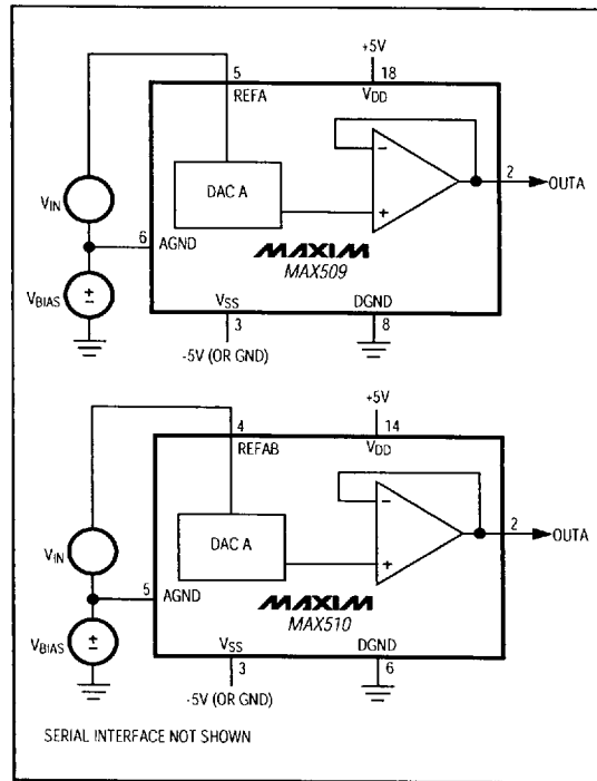
Figure 13. MAX509/MAX510 AGND Bias Circuits (Positive Offset)
