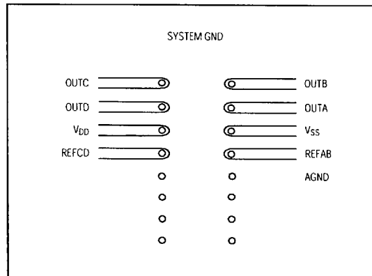
Figure 10. Suggested MAX510 PC Board Layout for Minimizing Crosstalk (Bottom View)
