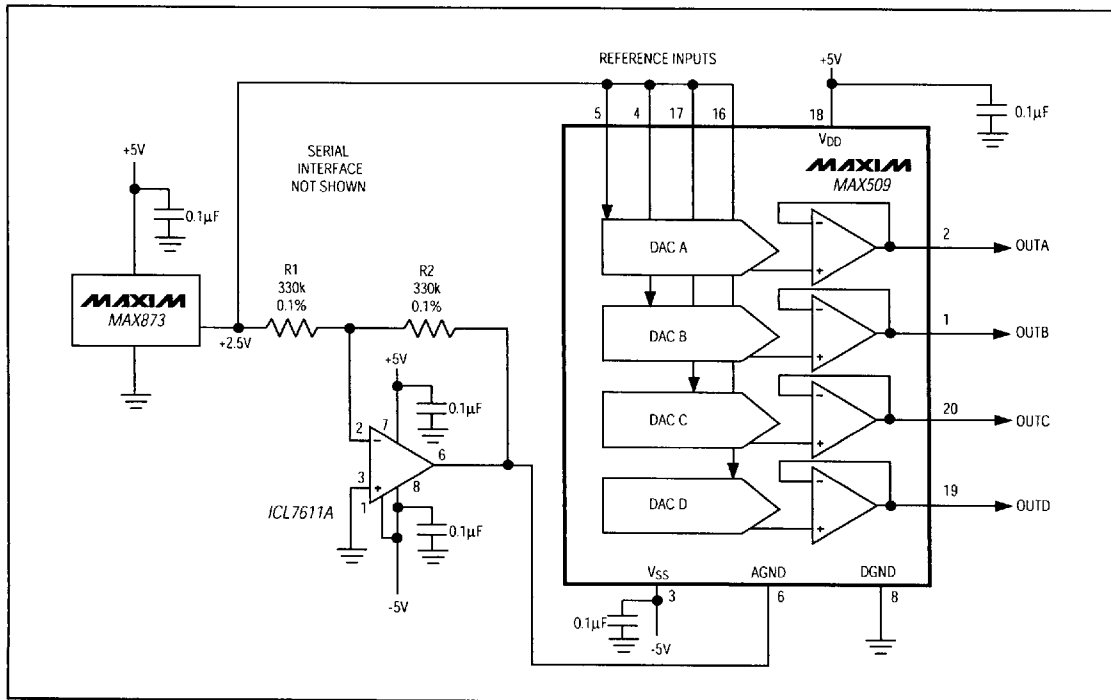
Figure 14. MAX509 AGND Bias Circuit (Negative Offset)
