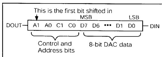
Figure 3. Serial Input Format
