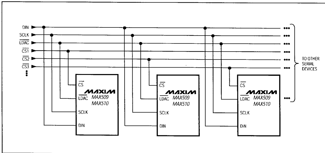
Figure 7. Multiple MAX509/MAX510 DACs sharing one DIN line. Simultaneously update by strobing \overline{LDAC} , or specifically update by enabling individual \overline{CS} .
