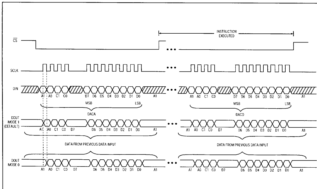
Figure 1. MAX509/MAX510 3-Wire Interface Timing
