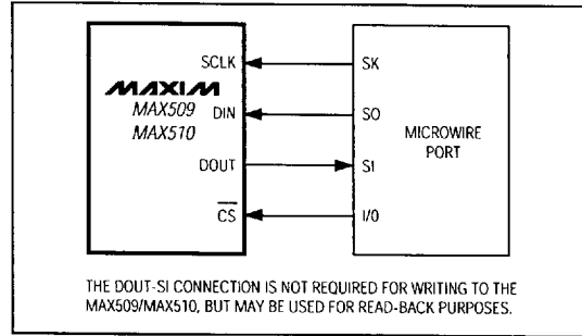
Figure 4. Connections for Microwire
