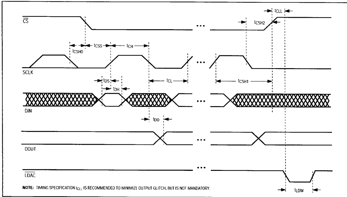
Figure 2. Detailed Serial Interface Timing (Mode 0 Shown)
