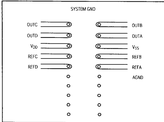
Figure 9. Suggested MAX509 PC Board Layout for Minimizing Crosstalk (Bottom View)
