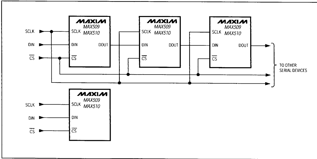
Figure 6. Daisy-chained or individual MAX509/MAX510s are simultaneously updated by bringing \overline{CS} high. Only three wires are required.
