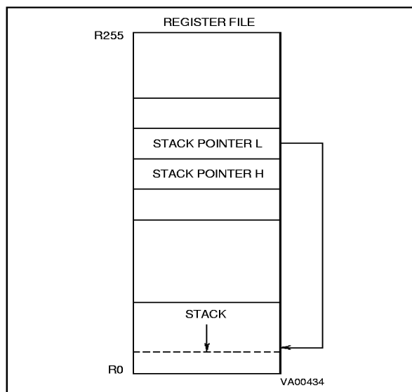
Figure 2-8. System and/or User Stack in Register Stack Mode
