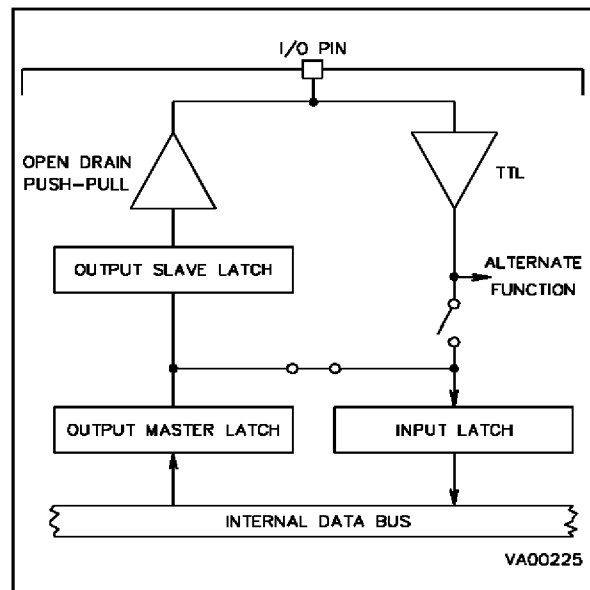
Figure 9-5. Output Configuration
