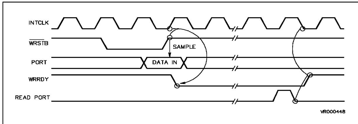
Figure 10-3. Two Line Input Handshake Timing
