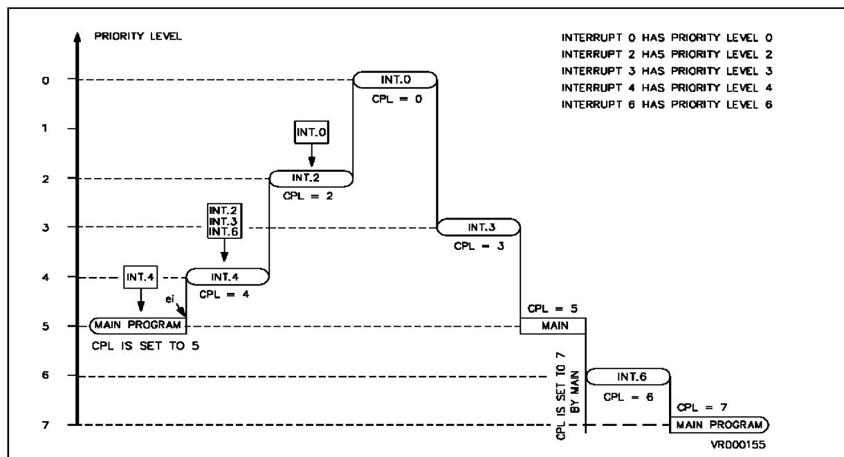
Figure 4-9. Example of a Sequence of Interrupt Requests with : - Nested mode - IEN unchanged by the interrupt routiness
