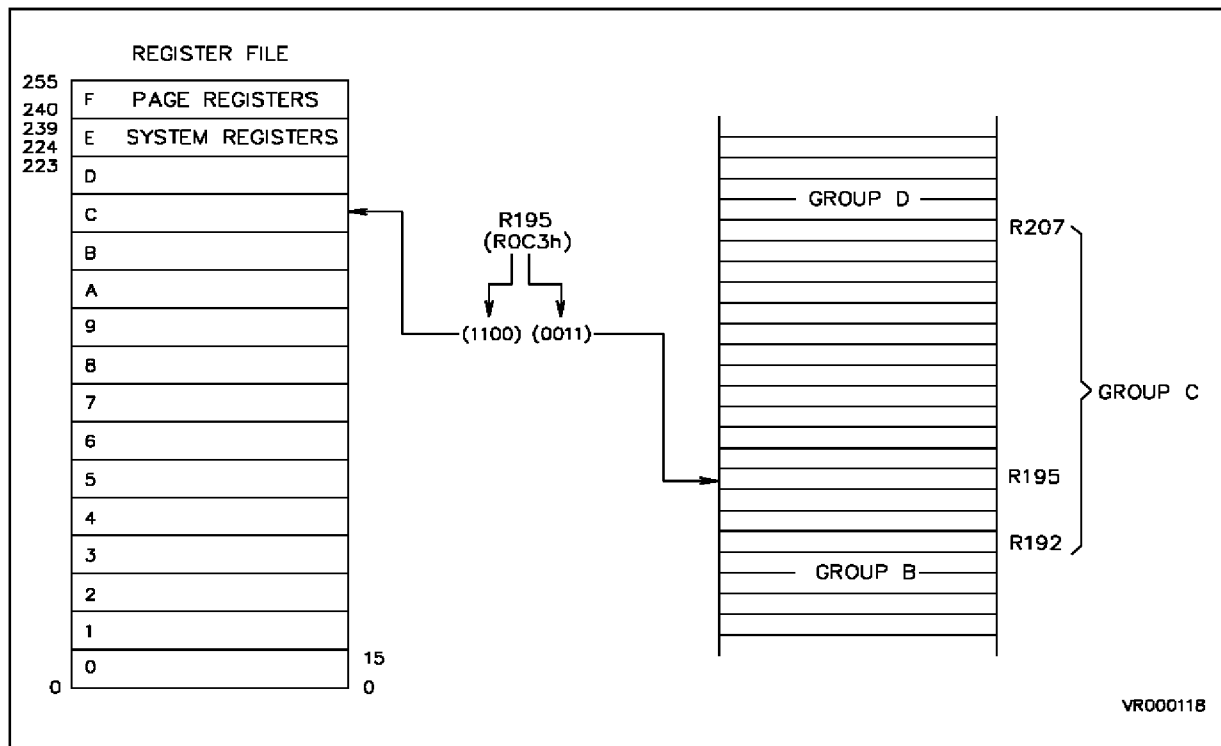
Figure 2-4. Addressing the Register File
