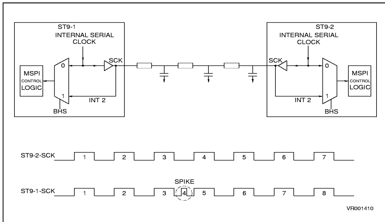
Figure 11-7. SPI Arbitration
