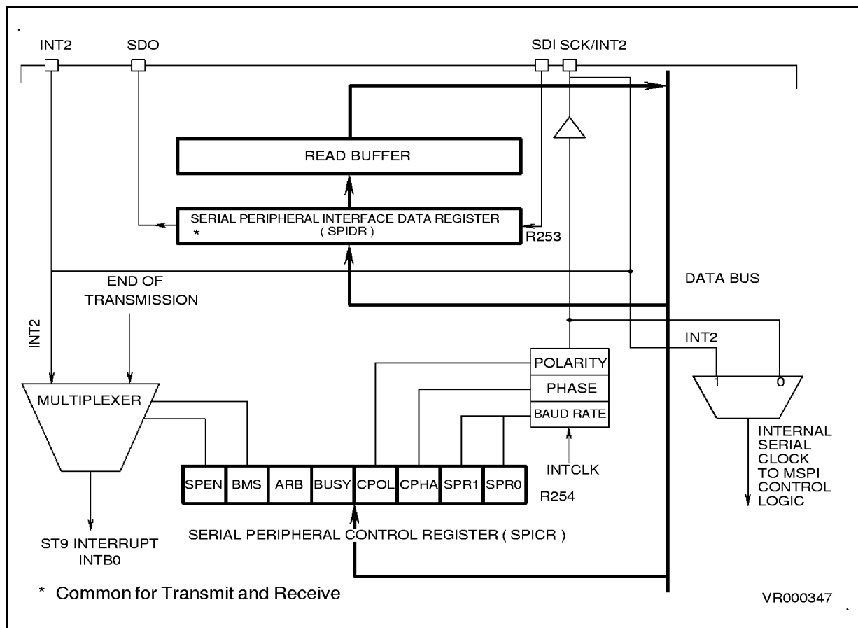
Figure 11-1. Block Diagram
