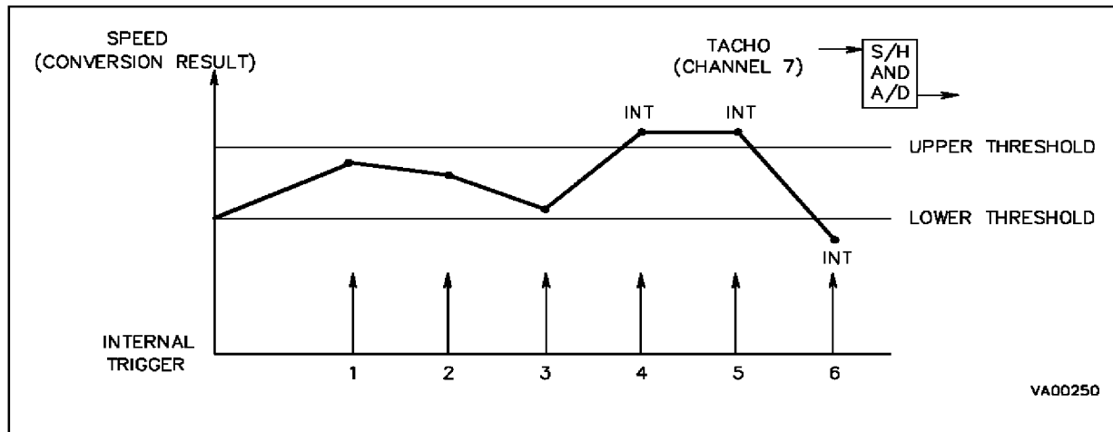
Figure 15-5. Analog Watchdog used in Motorspeed Control
