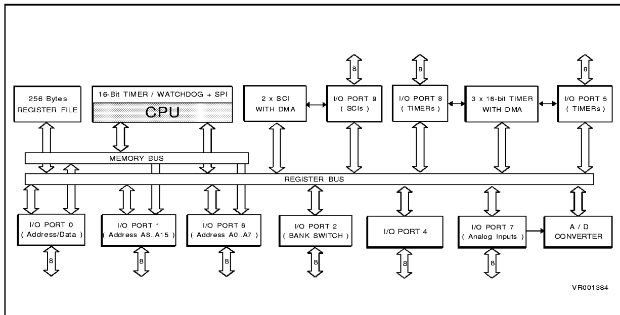
Figure 1-3. ST90R50 Block Diagram
