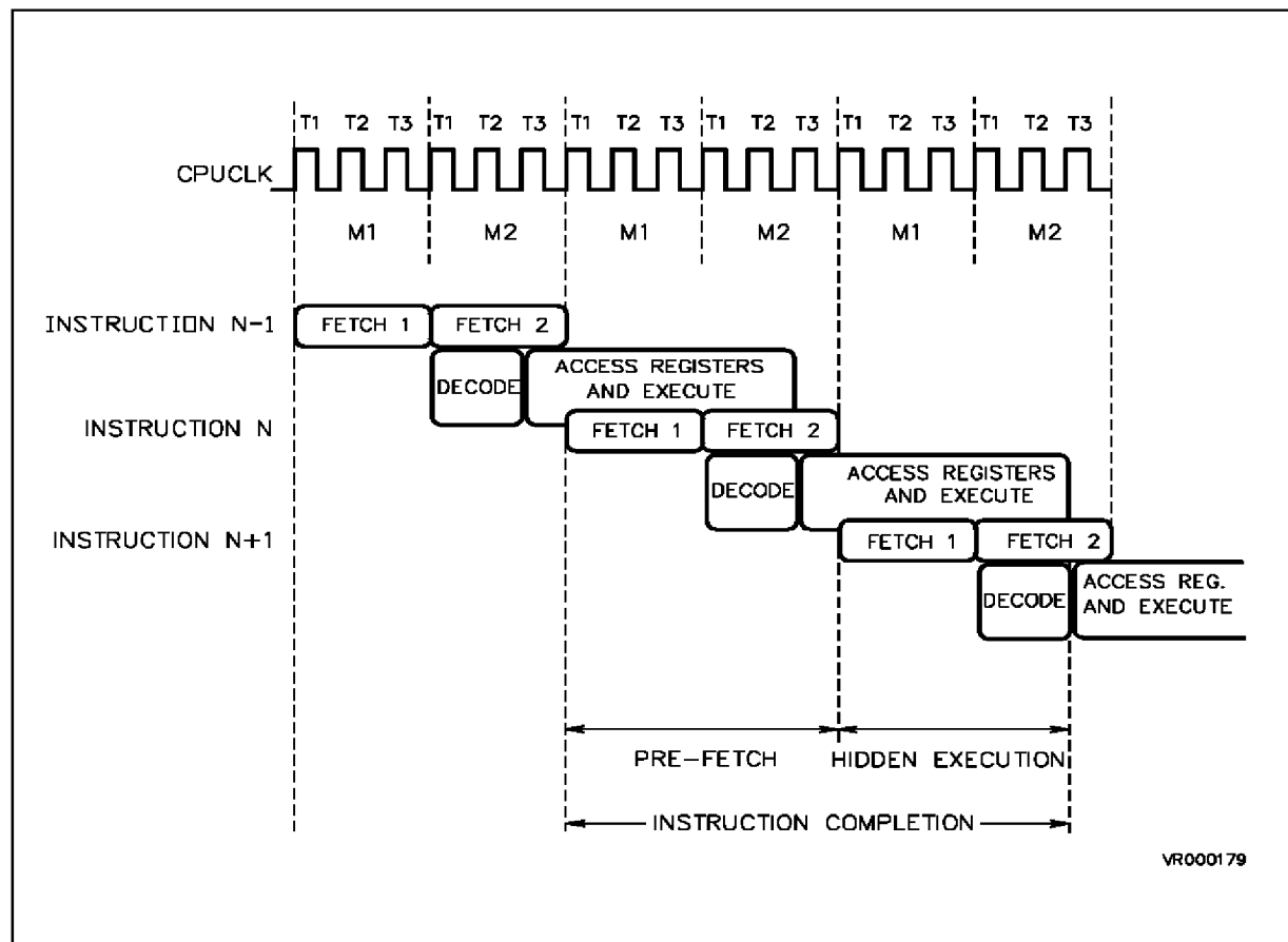
Figure 8-7. Instruction Pipe-line Stages
