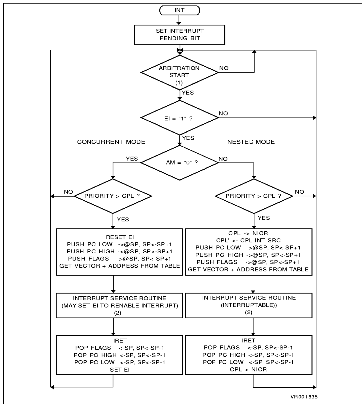
Figure 4-7. Interrupt Mode Flow-Chart
