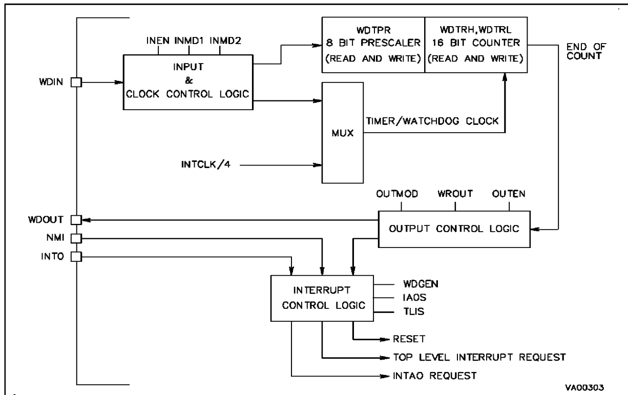
Figure 12-1. Block Diagram
