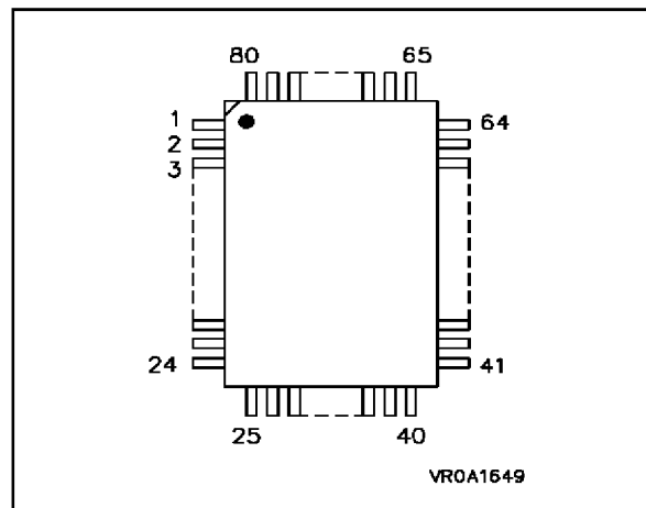
Figure 1-2. 80 Pin PQFP Package
