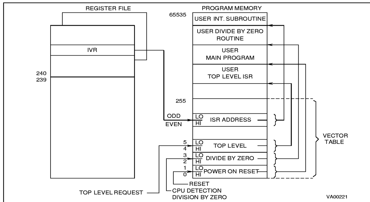
Figure 4-3. Interrupt Architecture, Example of priority Allocations
