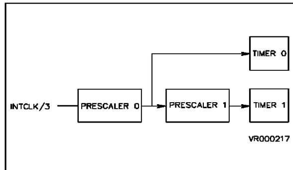
Figure 13-3. Parallel Mode Description
