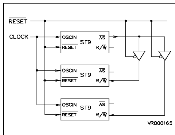
Figure 7-9. Synchronization Under Reset
