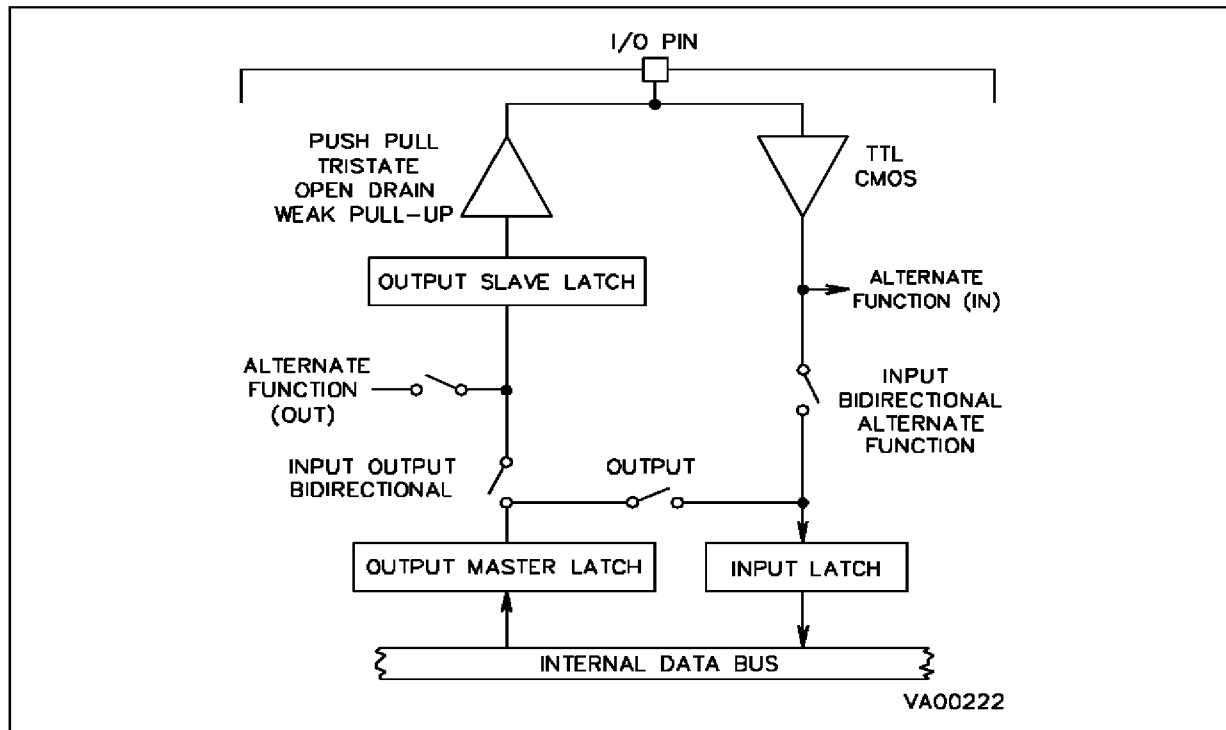
Figure 9-3. Basic Structure of an I/O Port Pin
