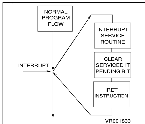
Figure 4-1. Interrupt Flow
