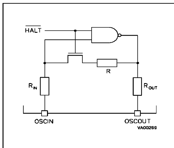
Figure 6-4. Internal Oscillator Schematic
