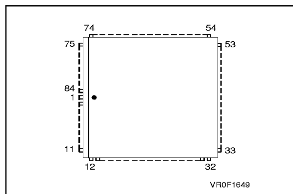
Figure 1-1. 84 Pin PLCC Package
