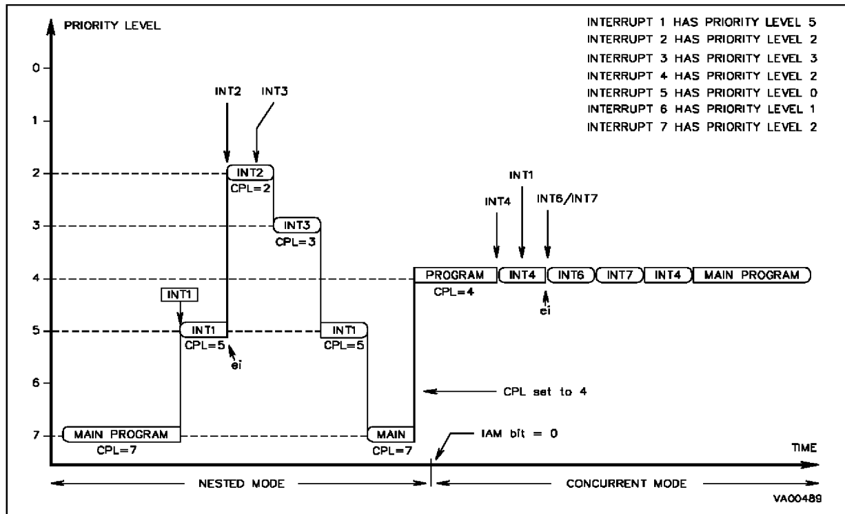
Figure 4-10. Example of a Nested and Concurrent Mode Sequence
