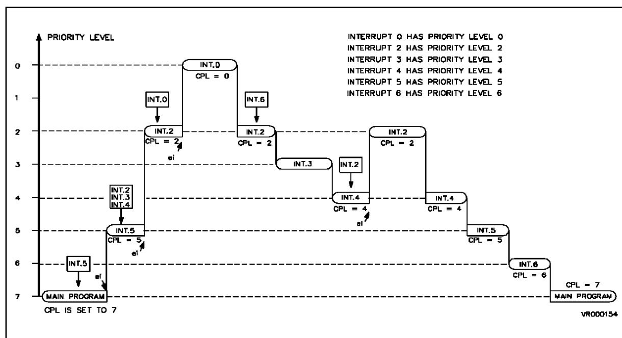
Figure 4-8. Example of a Sequence of Interrupt Requests with : - Nested mode - IEN set to 1 during the interrupt routine execution
