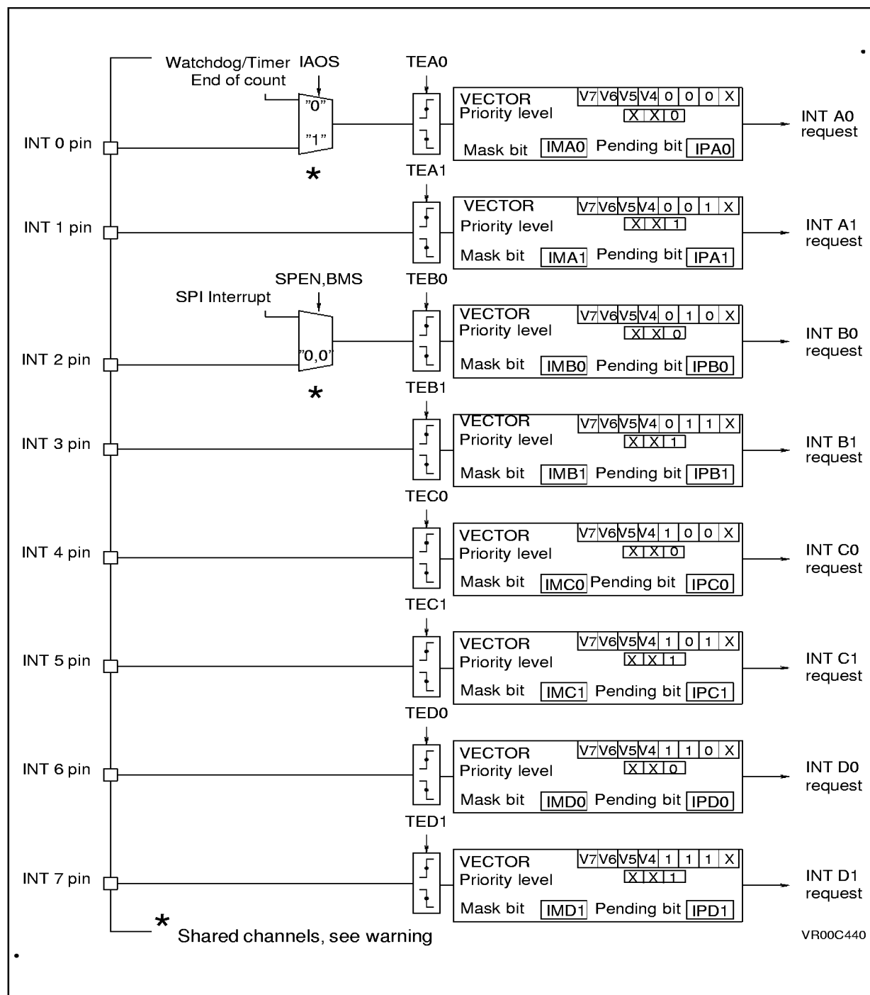
Figure 4-12. External Interrupts Control Bits and Vectors
