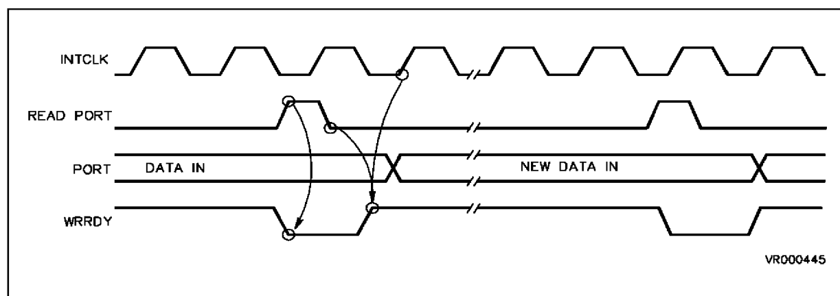
Figure 10-5. One Line Input Handshake Timing
