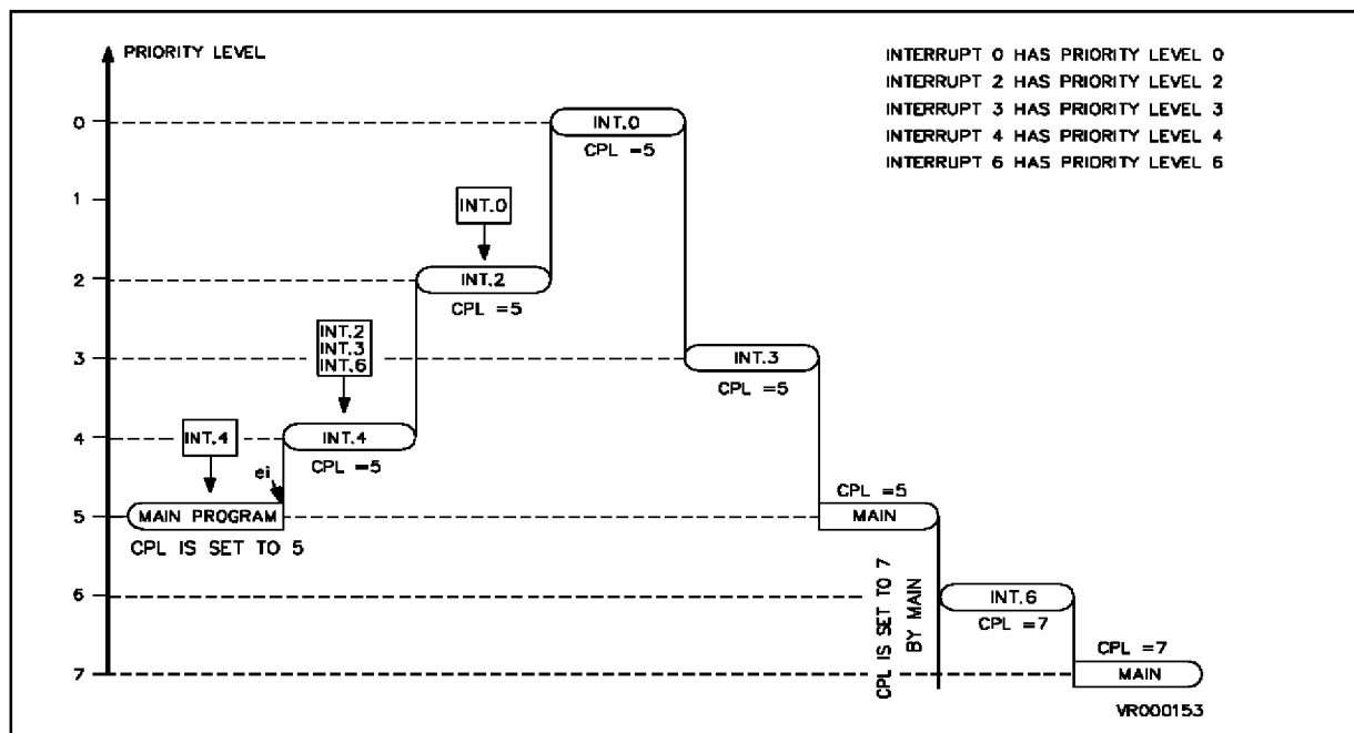
Figure 4-6. Example of a Sequence of Interrupt Requests with :
