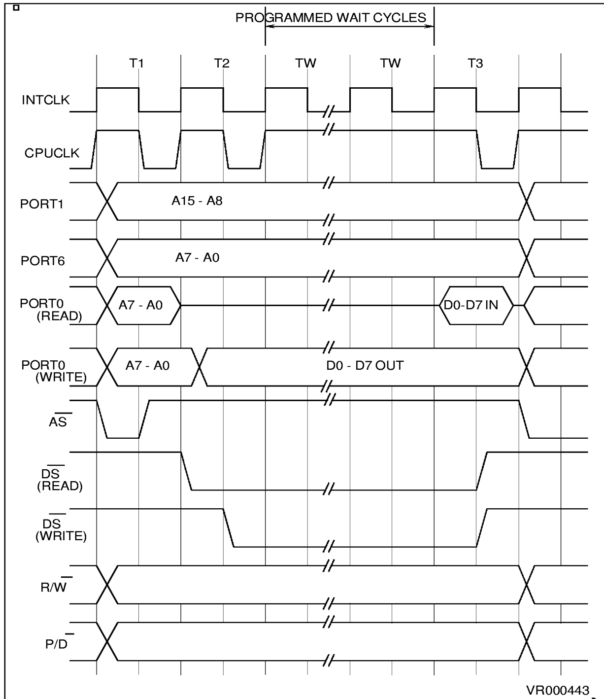
Figure 8-4. External Memory Read/Write Sequence with Programmable Wait.
