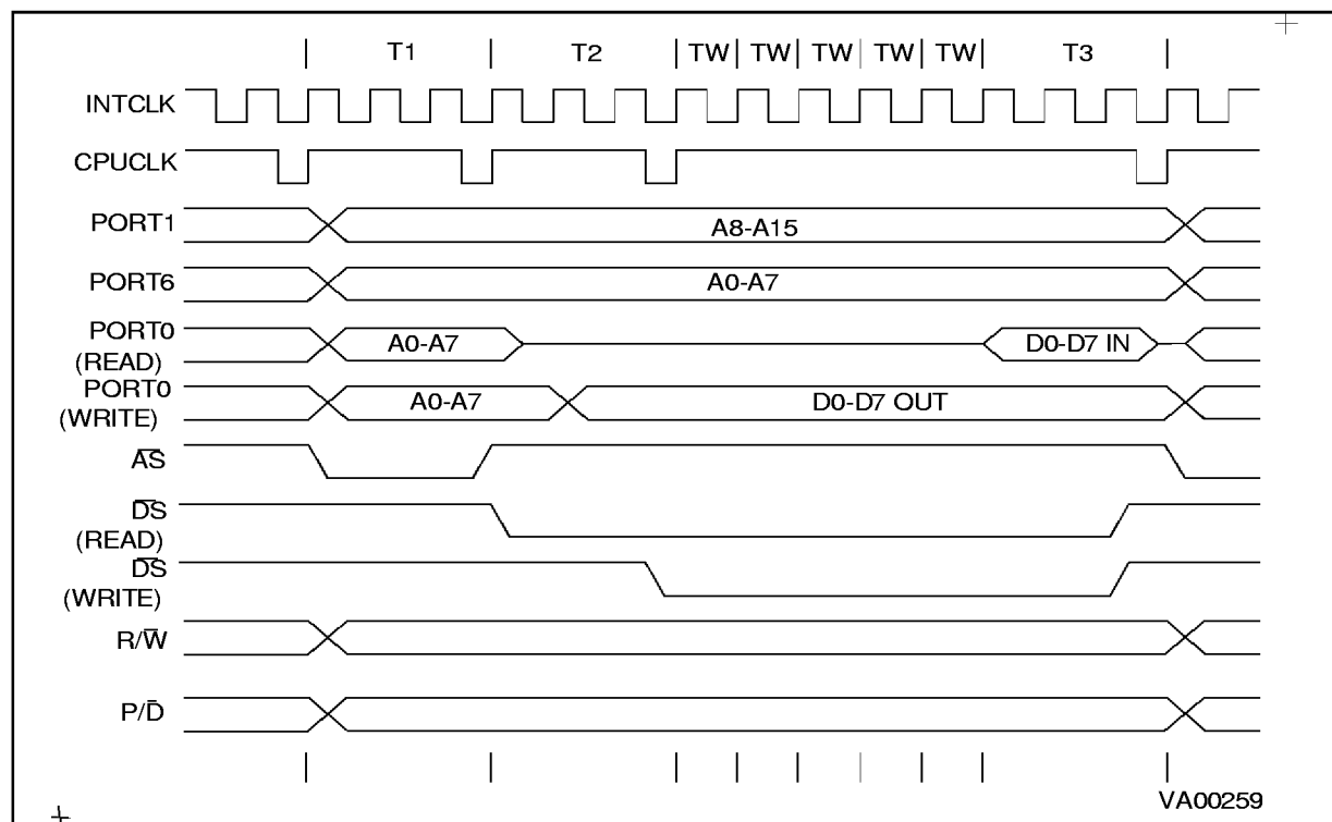
Figure 6-3. Memory Access with a Clock Prescaler by 2 and 5 Wait Cycle
