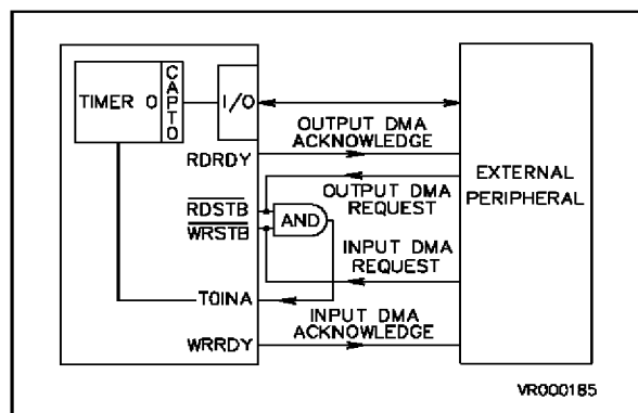
Figure 10-17. DMA input/output transfers with bidirectional handshake
