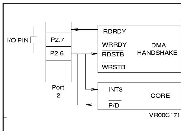
Figure 9-10. Example of One I/O Pin Configuration
