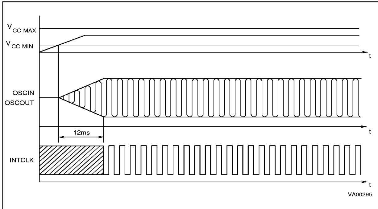
Figure 6-7. Oscillator Start-up Sequence
