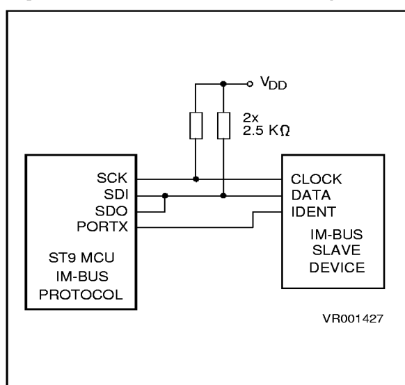
Figure 11-10. ST9 and InterMetal Peripheral
