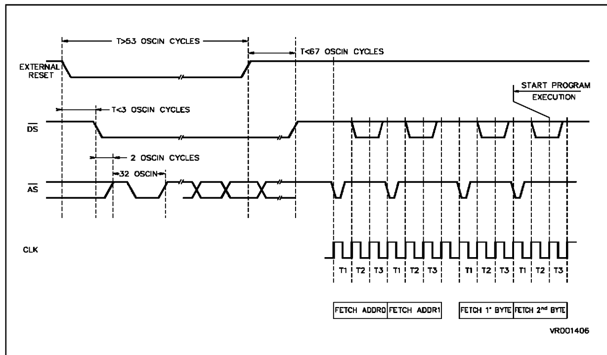
Figure 7-10. Exit From Reset Timing
