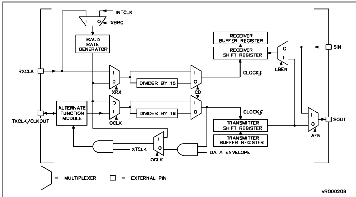
Figure 14-11. SCI Functional Scheme
