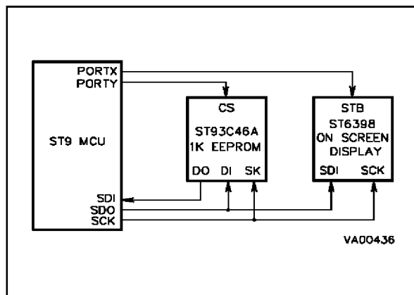
Figure 11-2. A Typical SPI Network
