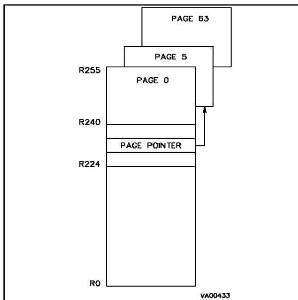
Figure 2-3. Page Pointer Configuration
