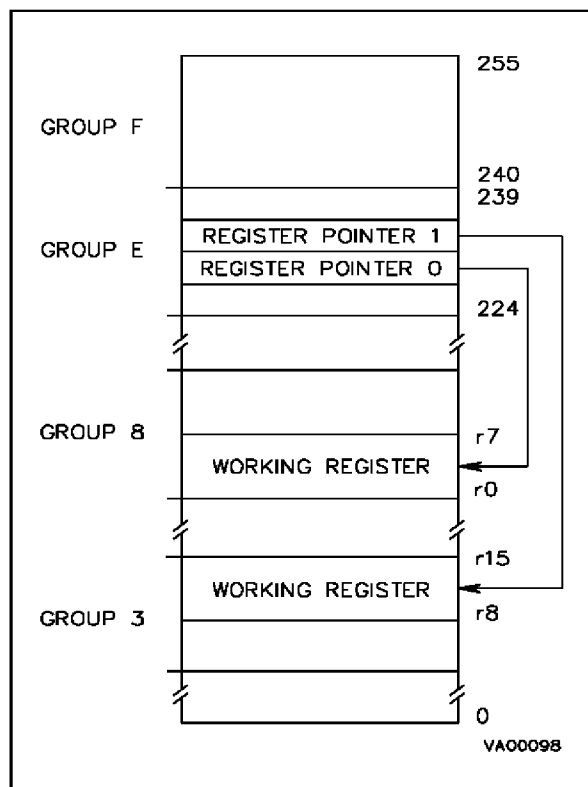
Figure 2-7. Double Register pointing Mode
