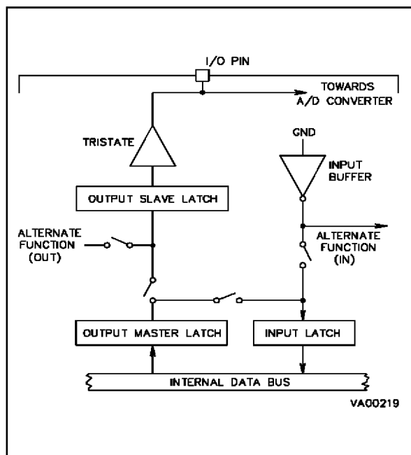
Figure 15-2. A/D Input Configuration Status
