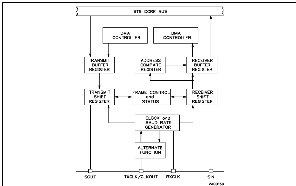
Figure 14-1. SCI Block Diagram
