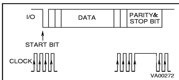
Figure 14-4. Synchronous Mode
