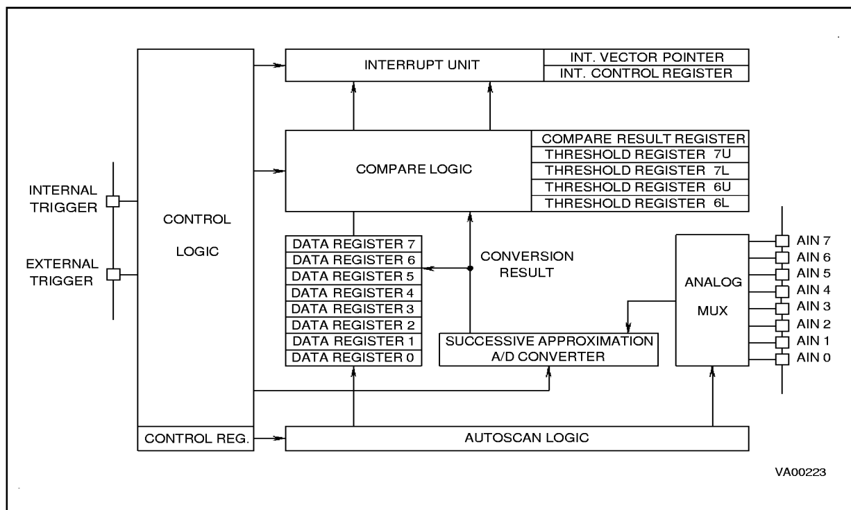
Figure 15-1. Block Diagram
