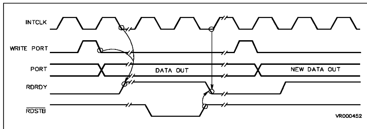
Figure 10-7. Two Line Output Handshake Timing
