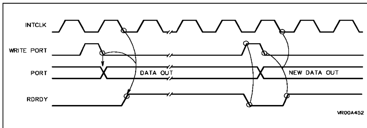
Figure 10-9. One Line Output Handshake Timing
