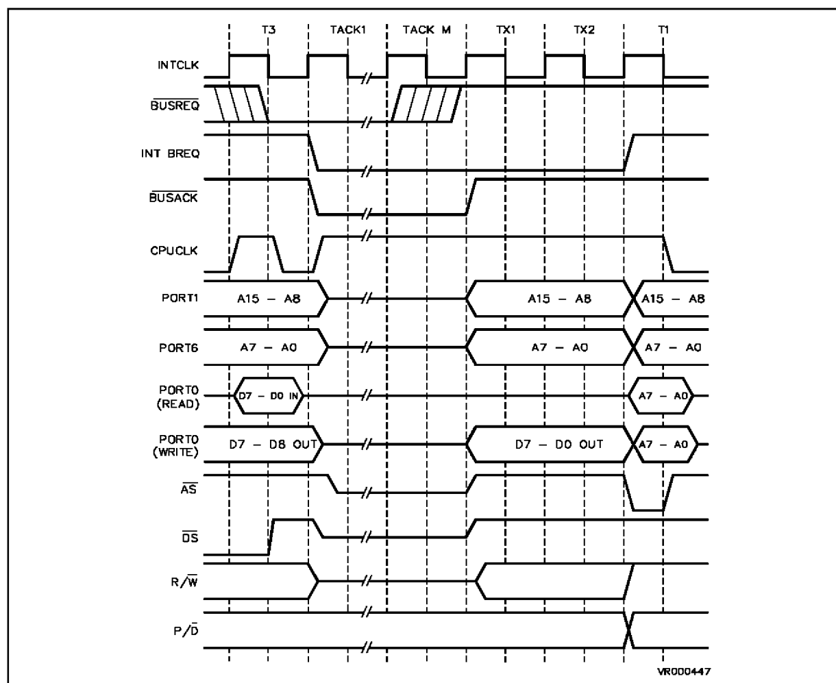
Figure 8-5. Bus Request/Acknowledge Timing.
