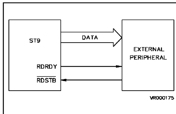
Figure 10-6. Two Line Output Handshake
