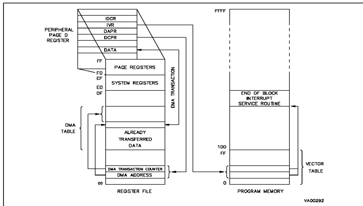
Figure 5-3. DMA Between Memory and peripherals
