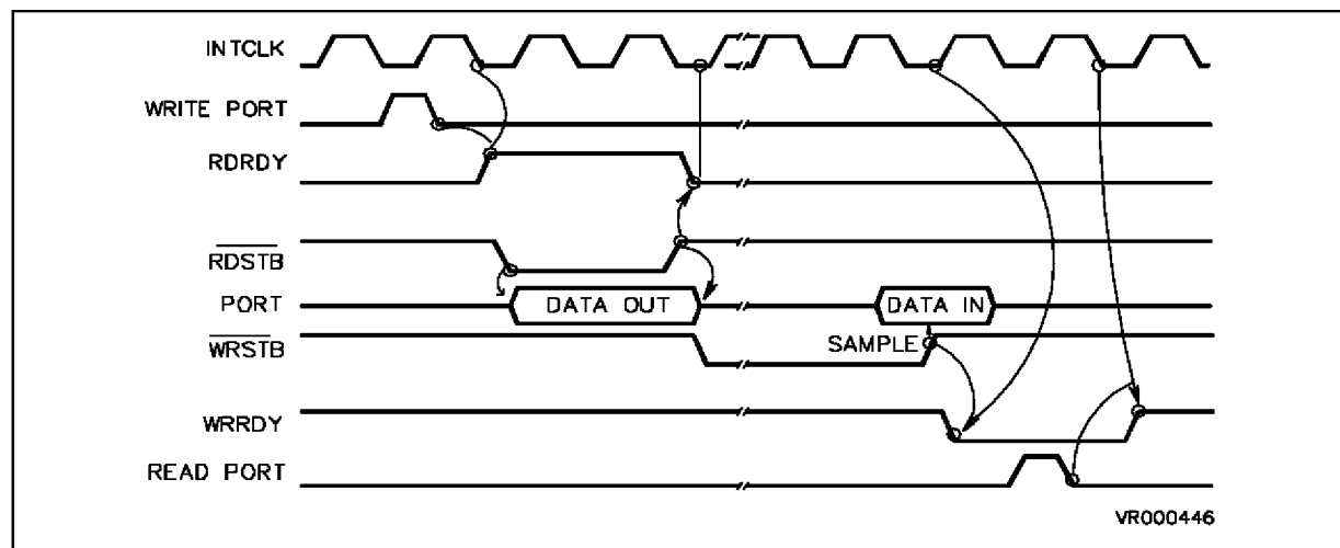
Figure 10-11. Bidirectional Handshake Timing
