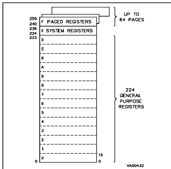
Figure 2-2. Register Grouping
