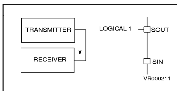
Figure 14-8. Loop Back Configuration
