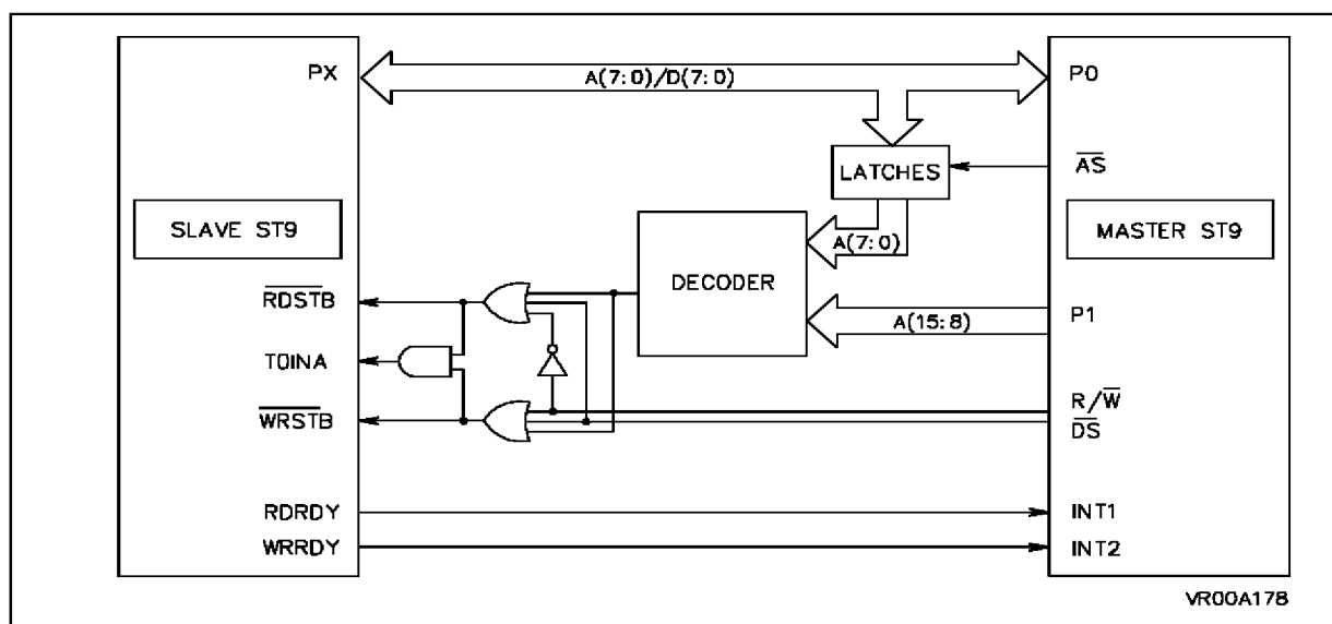
Figure 10-18. Bidirectional Application Example With DMA Transfer
