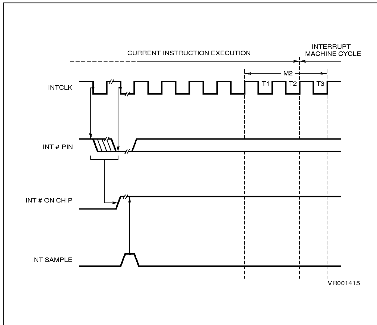
Figure 4-16. External Interrupt Response Time
