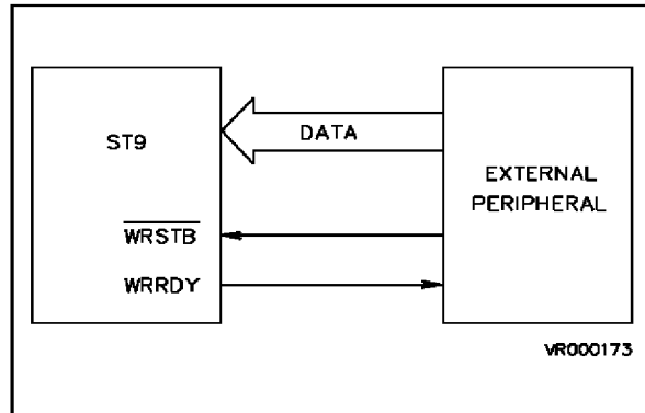
Figure 10-2. Two Line Input Handshake
