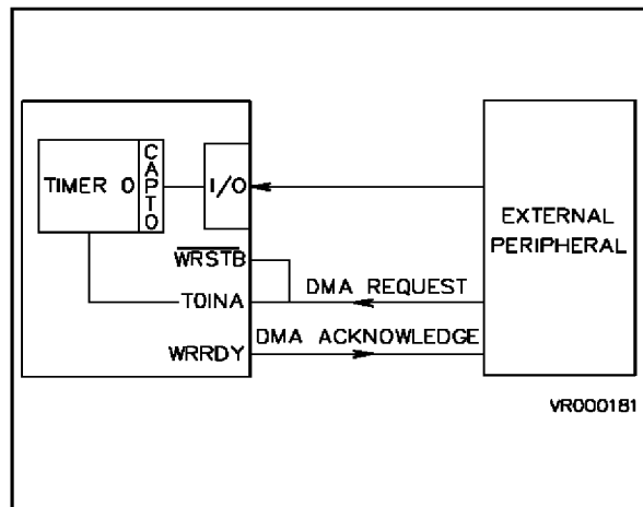
Figure 10-13. DMA with 2 Line Input Handshake Mode
