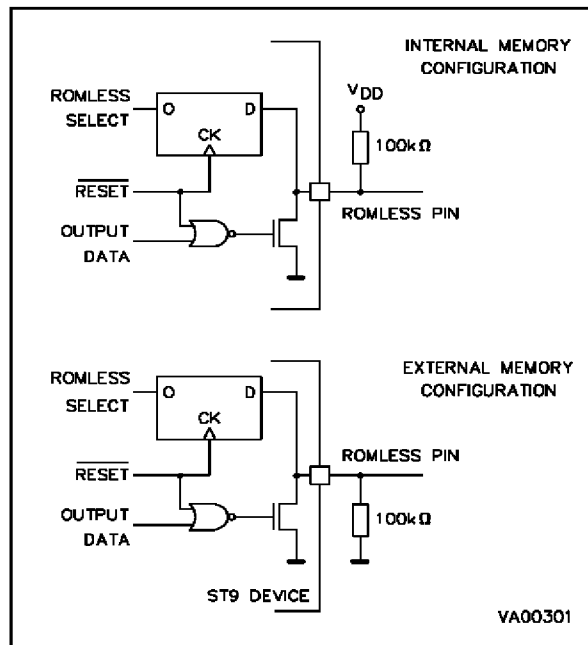
Figure 8-6. ROMless Selection
