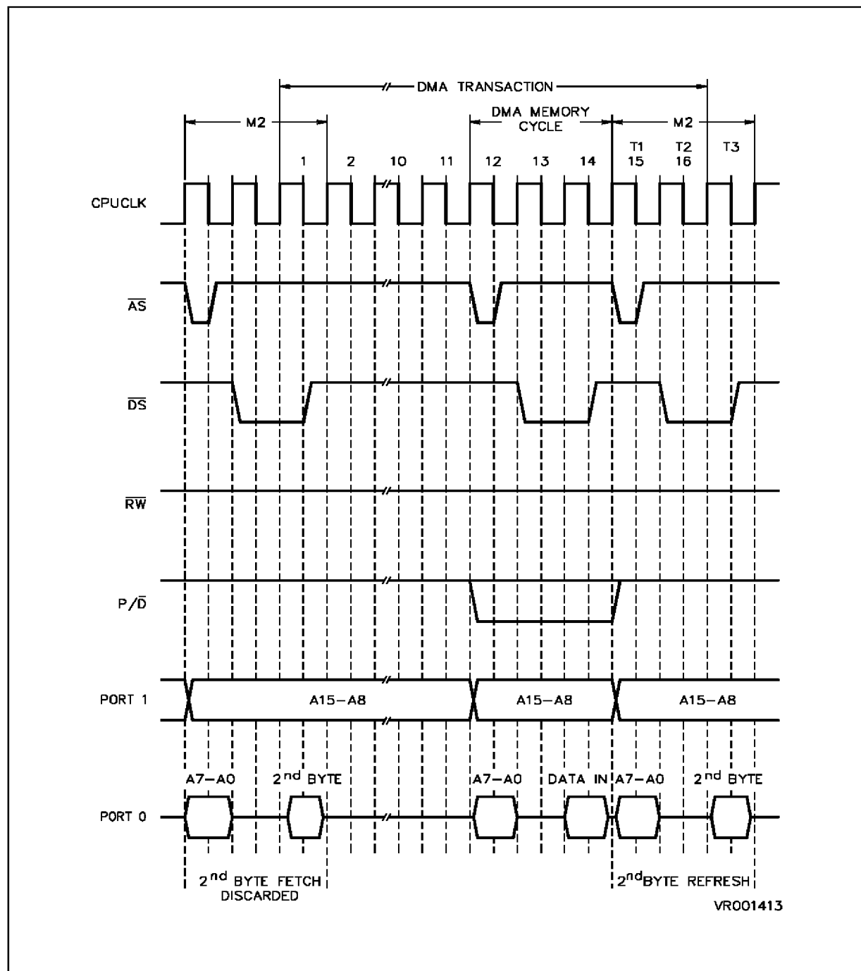
Figure 5-5. DMA Transaction from Memory
