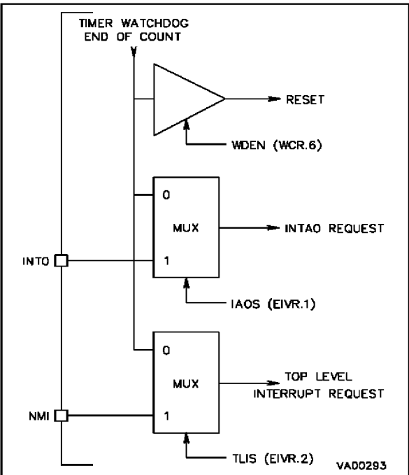
Figure 12-3. Interrupt Sources
