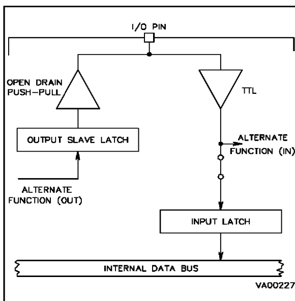
Figure 9-7. Alternate Function Configuration
