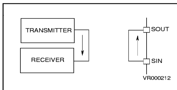
Figure 14-9. Auto Echo and Loop Back Config.
