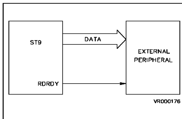
Figure 10-8. One Line Output Handshake
