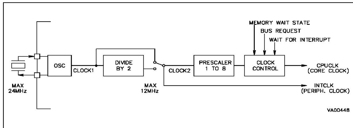
Figure 6-1. Peripheral and Core Clocks
