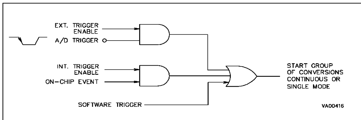
Figure 15-3. A/D Trigger Source
