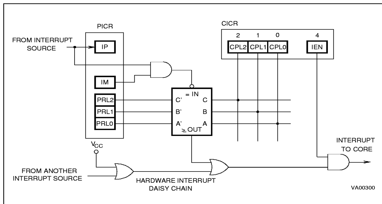
Figure 4-4. Interrupt Logic
