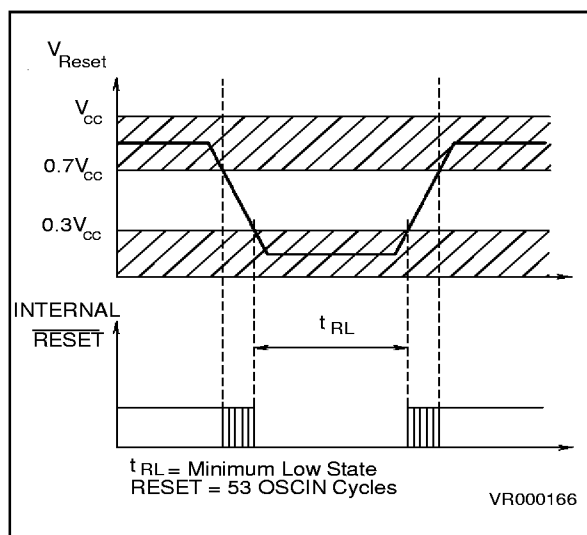
Figure 7-8. Signal to be applied on Reset Pin
