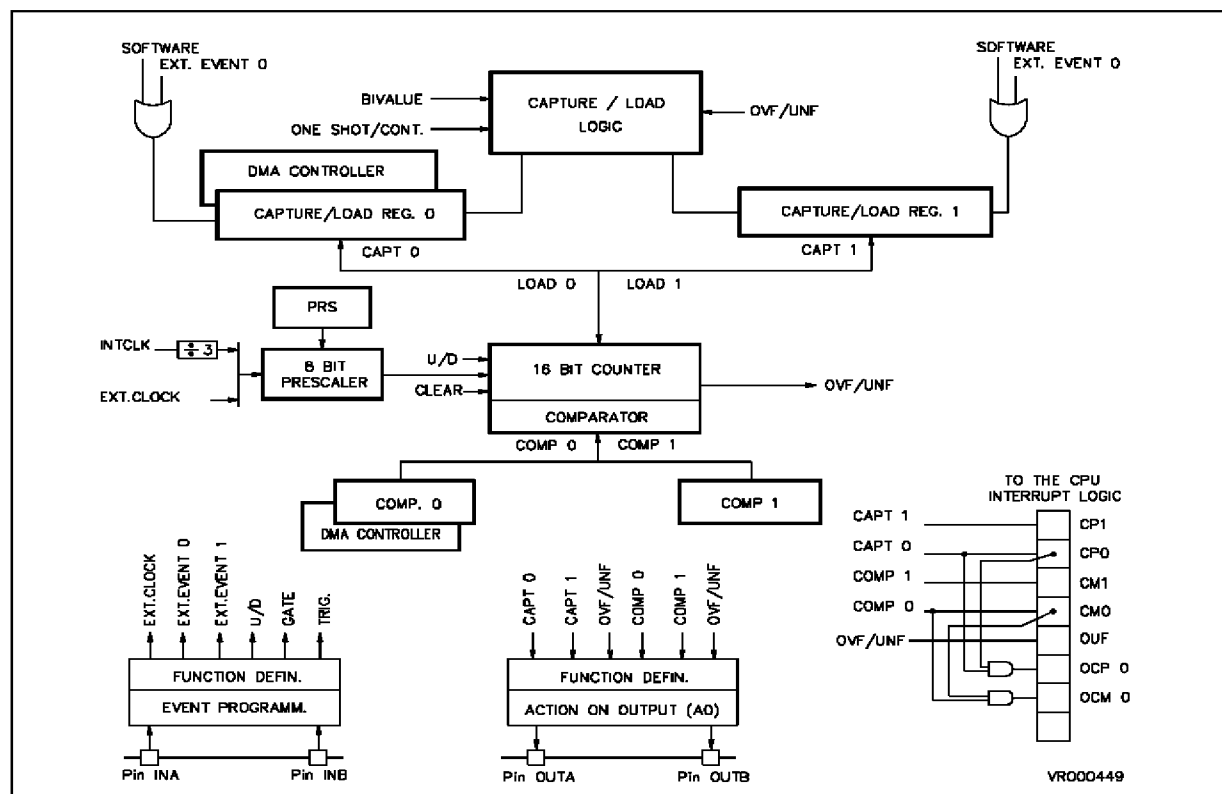
Figure 13-2. Detailed Block Diagram
