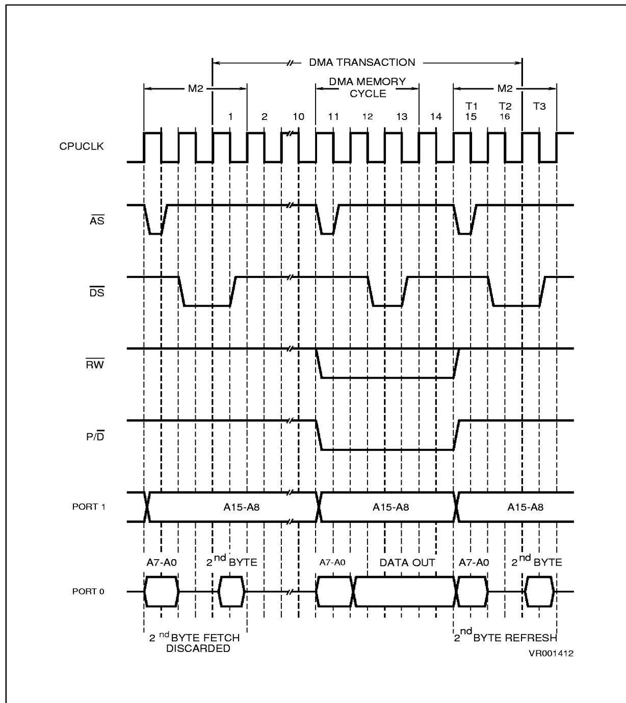
Figure 5-4. DMA Transaction to Memory
