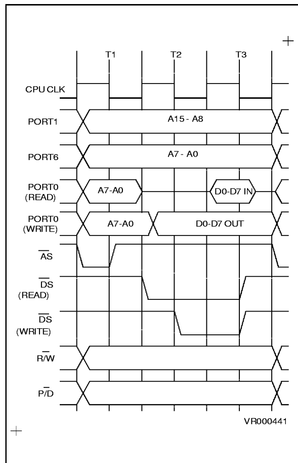
Figure 8-2. External Memory Read/Write.
