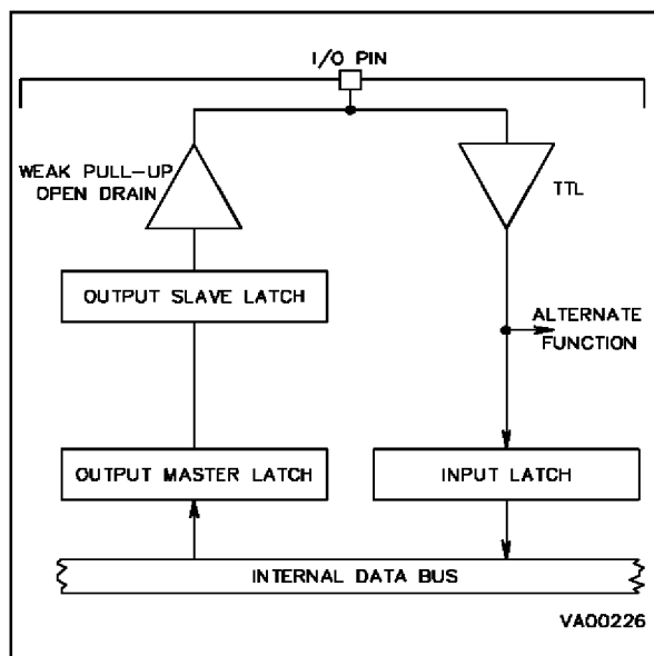
Figure 9-6. Bidirectional Configuration
