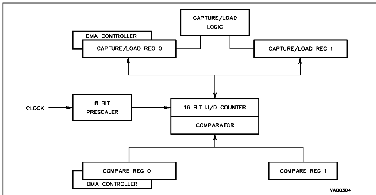
Figure 13-1. MFT Simplified Block Diagram
