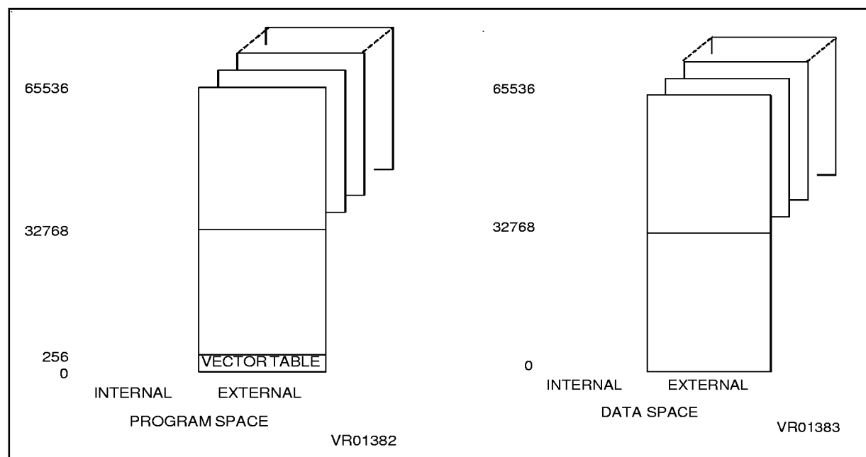
Figure 3-1. Program and Data Spaces
