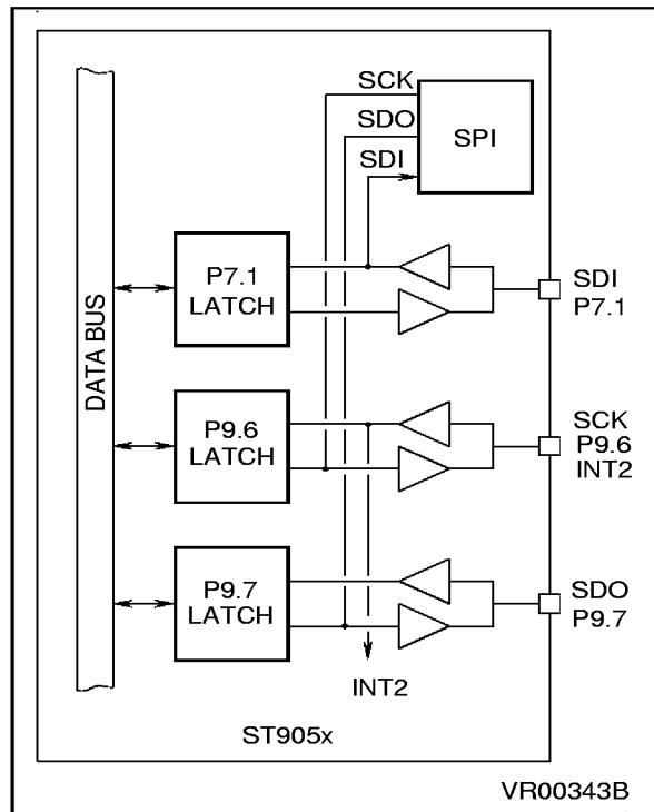
Figure 11-3. SPI I/O Pins
