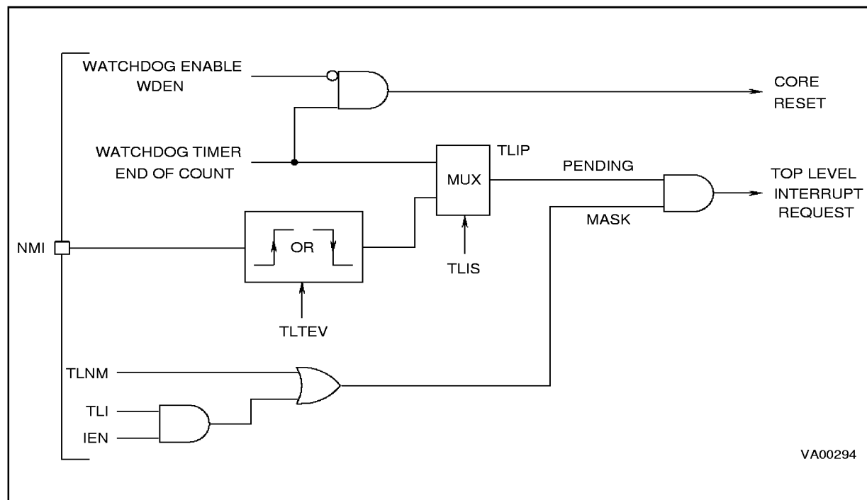
Figure 4-13. Top Level Interrupt Structure
