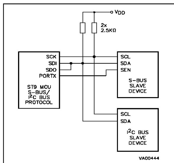
Figure 11-9. S-bus Configuration
