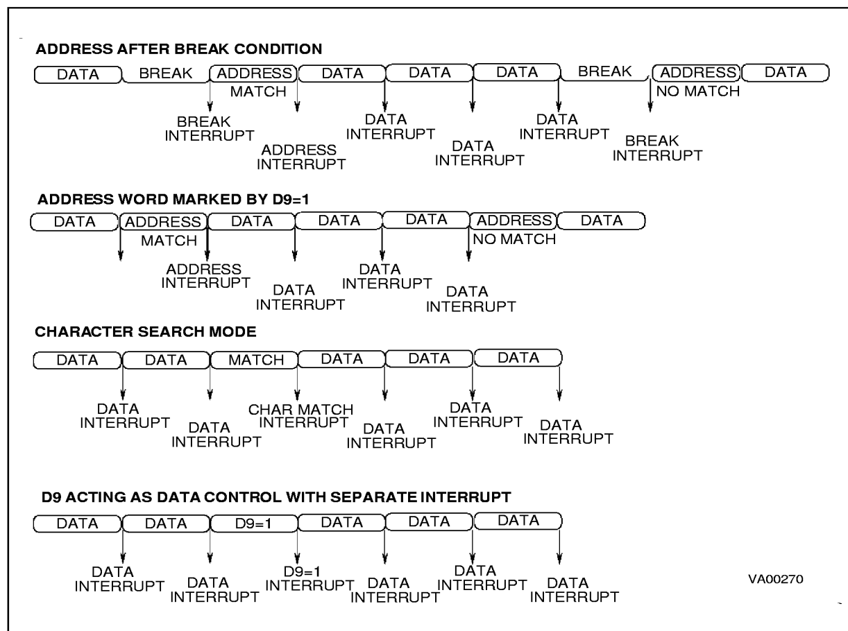
Figure 14-10. SCI Interrupt Typical Usage
