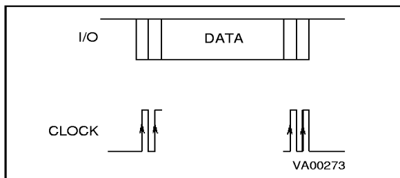
Figure 14-5. Serial Expansion Mode
