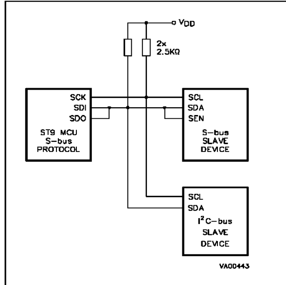
Figure 11-4. S-Bus/I 2 C-bus Peripheral Compatibility without S-Bus Chip Select
