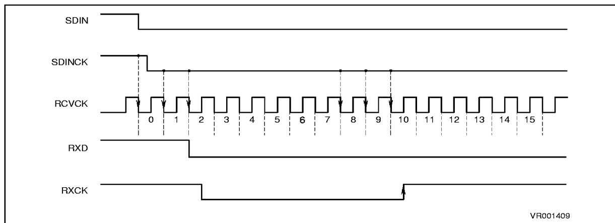
Figure 14-2. Sampling Times in Asynchronous Format
