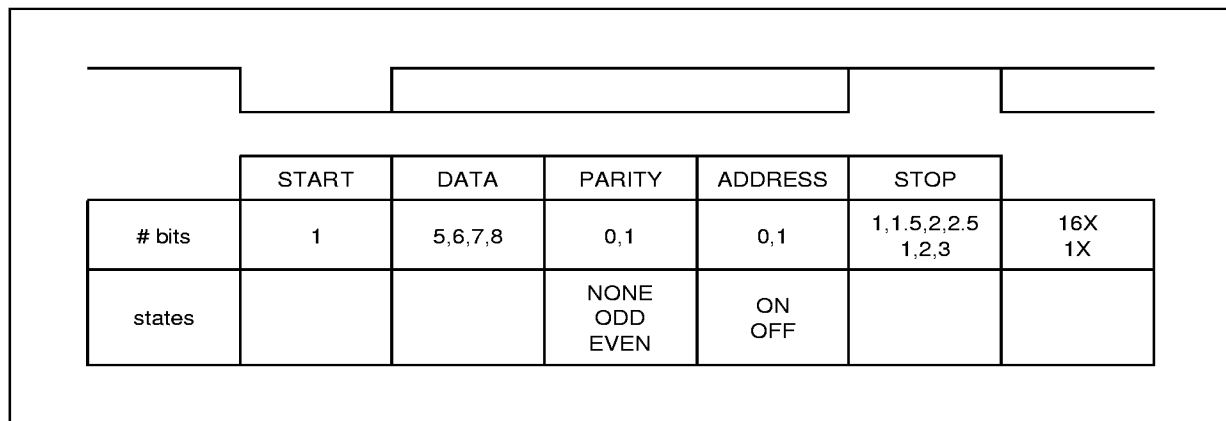
Figure 14-6. SCI Character Format
