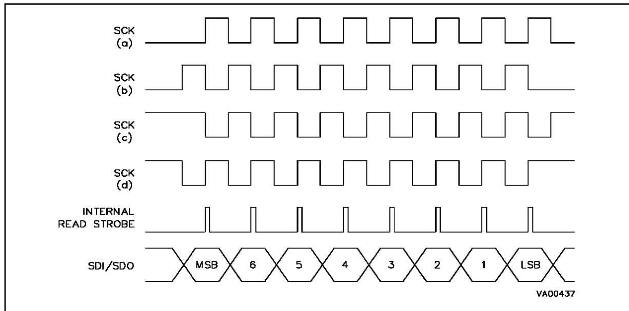
Figure 11-5. SPI Data and Clock Timing
