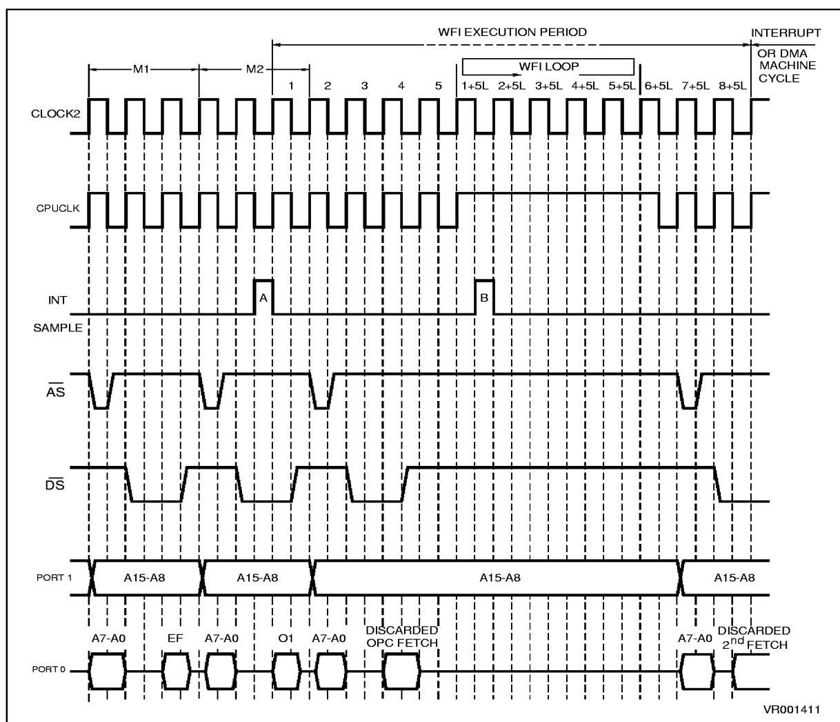
Figure 4-14. Wait For Interrupt Timing
