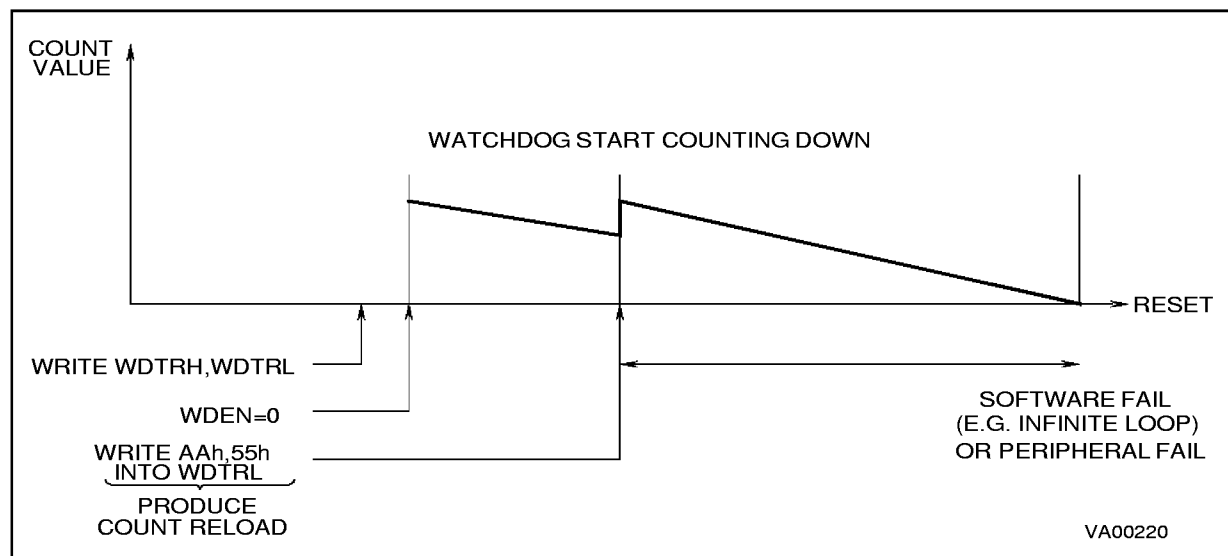
Figure 12-2. Timer /Watchdog in Watchdog Mode
