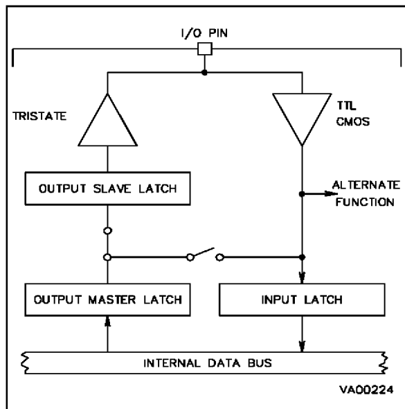
Figure 9-4. Input Configuration
