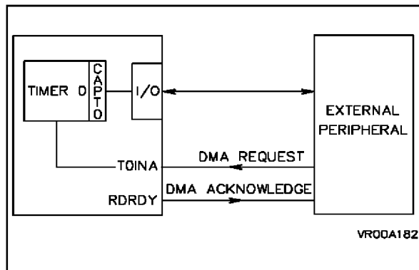
Figure 10-16. DMA output transfers with one line output handshake
