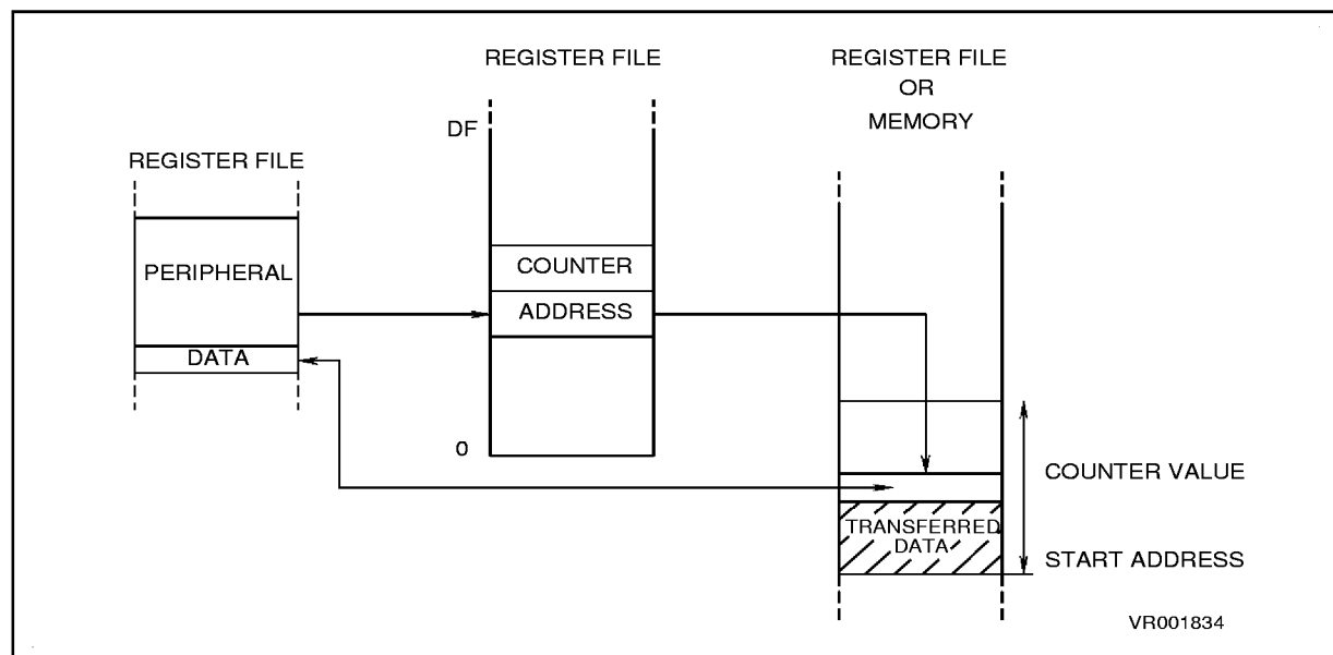
Figure 5-1. DMA Overview
