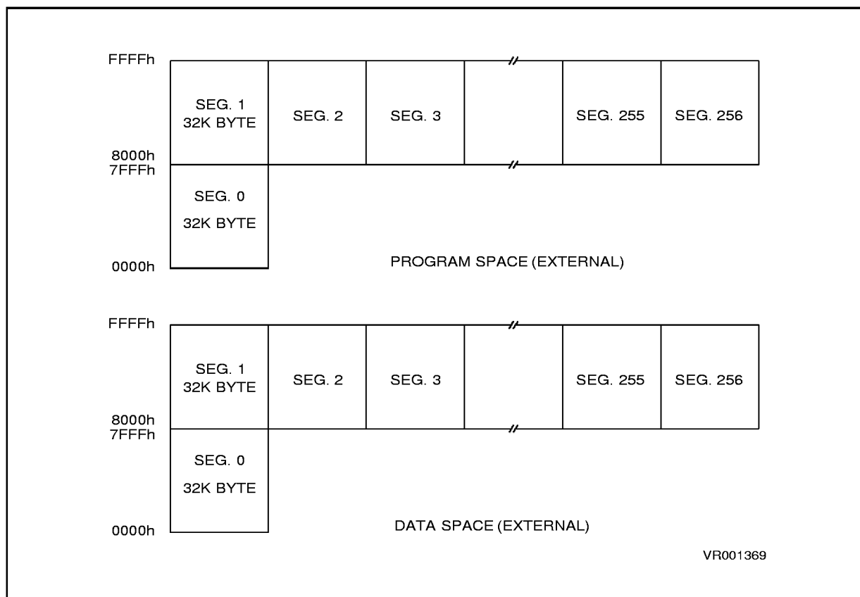
Figure 3-2. Bank Switch Memory Maps
