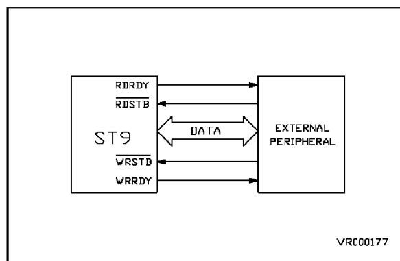
Figure 10-10. Four Line Bidirectional
