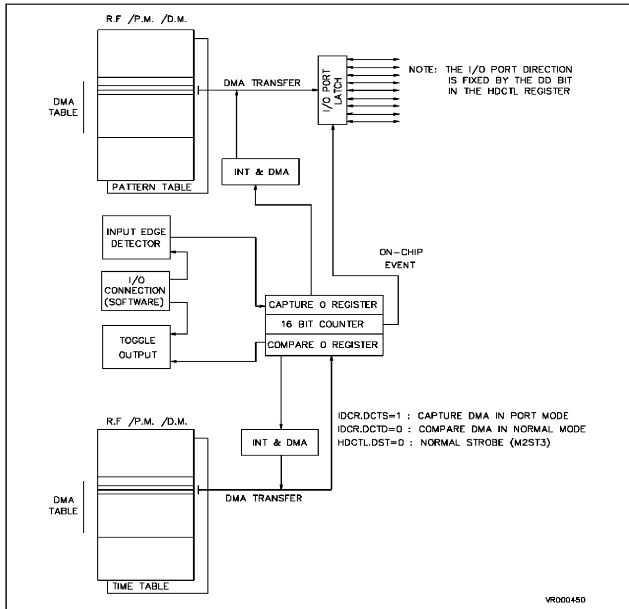
Figure 13-6. Timer DMA Channels Synchronization
