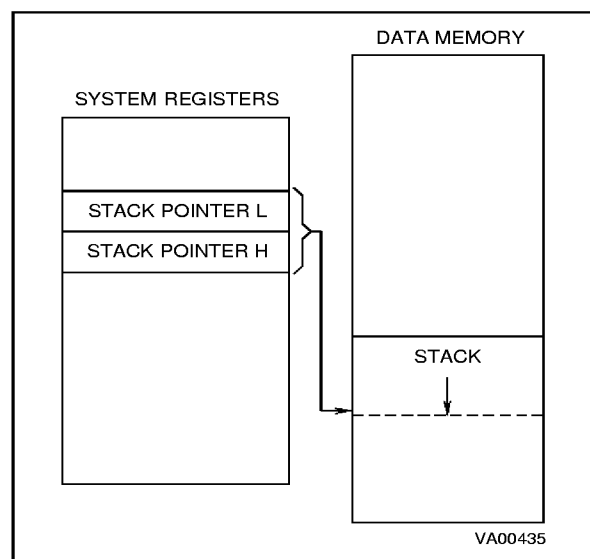
Figure 2-9. System and/or User Stack in Memory Stack Mode
