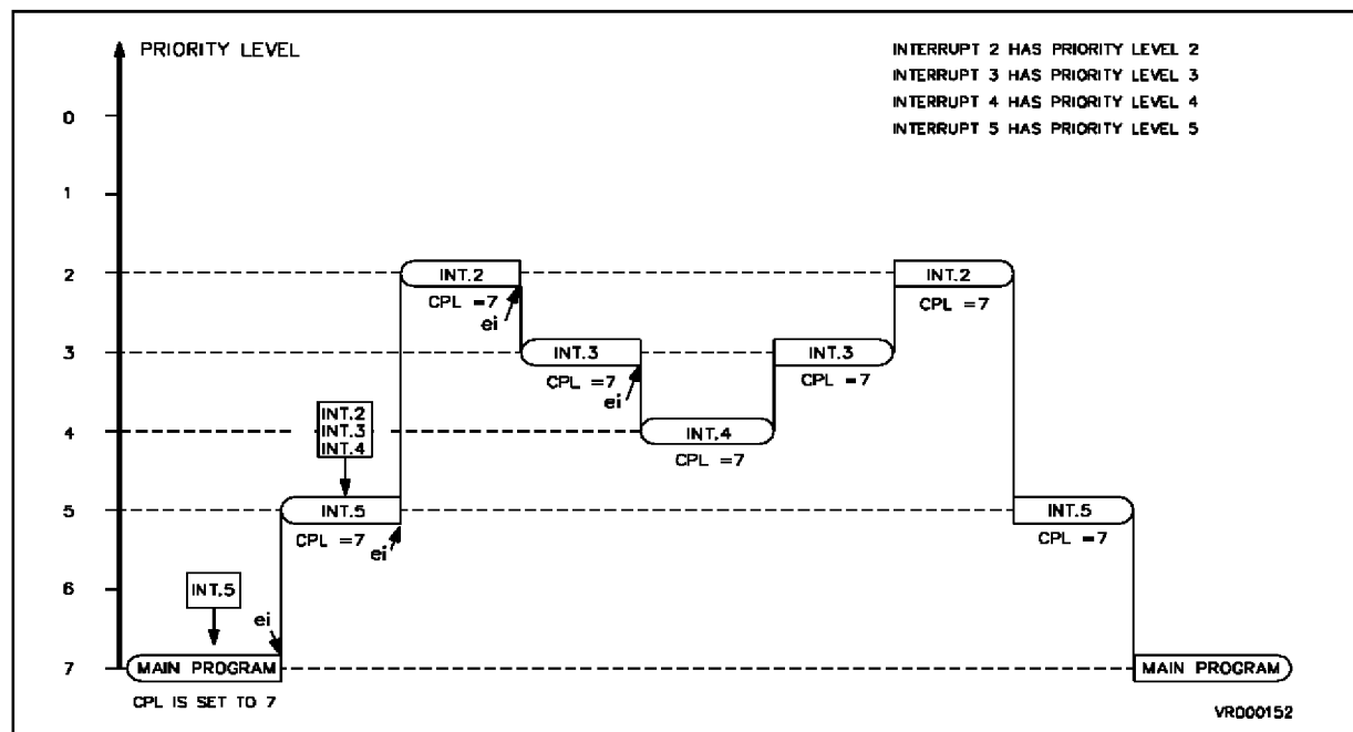
Figure 4-5. Example of a Sequence of Interrupt Requests with :
