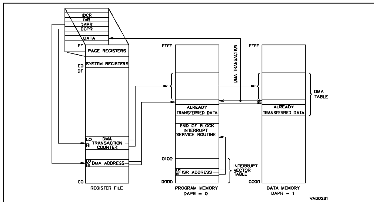
Figure 5-3. DMA Between Memory and peripherals
