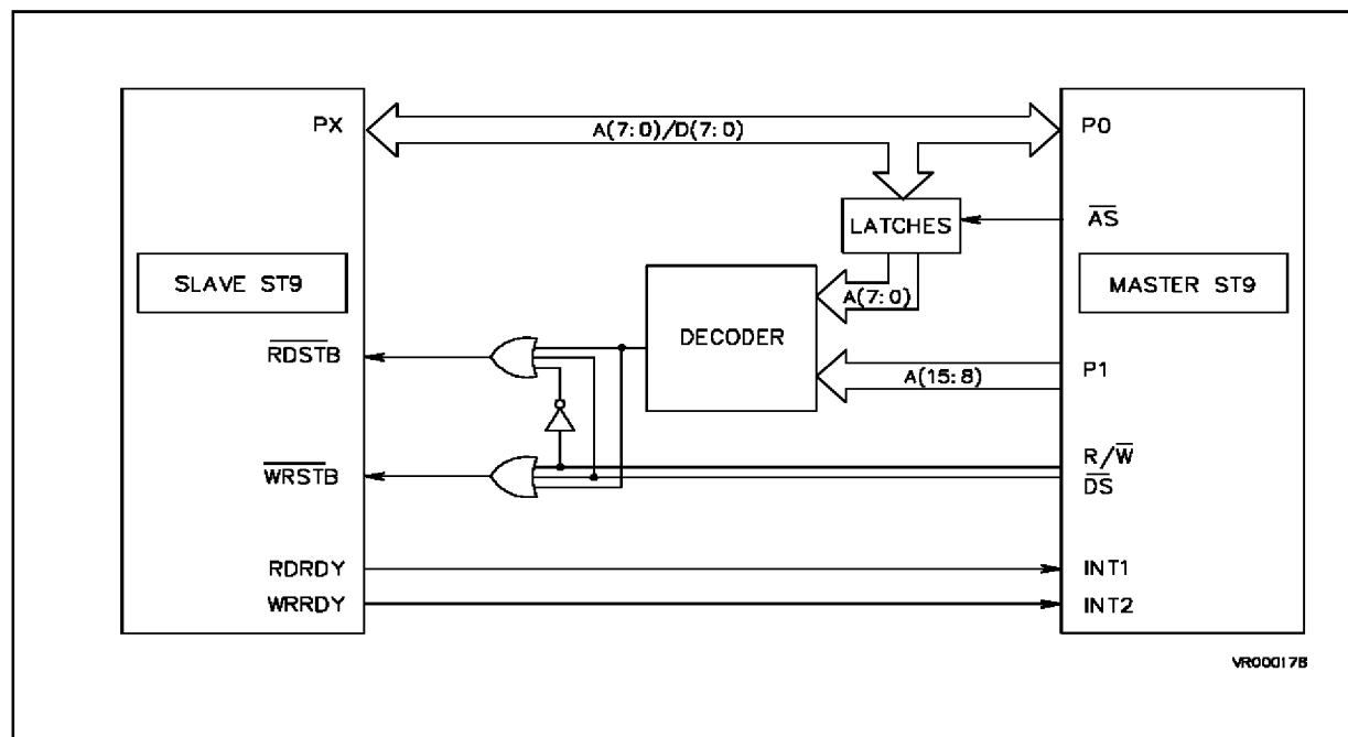
Figure 10-12. Bidirectional Application Example
