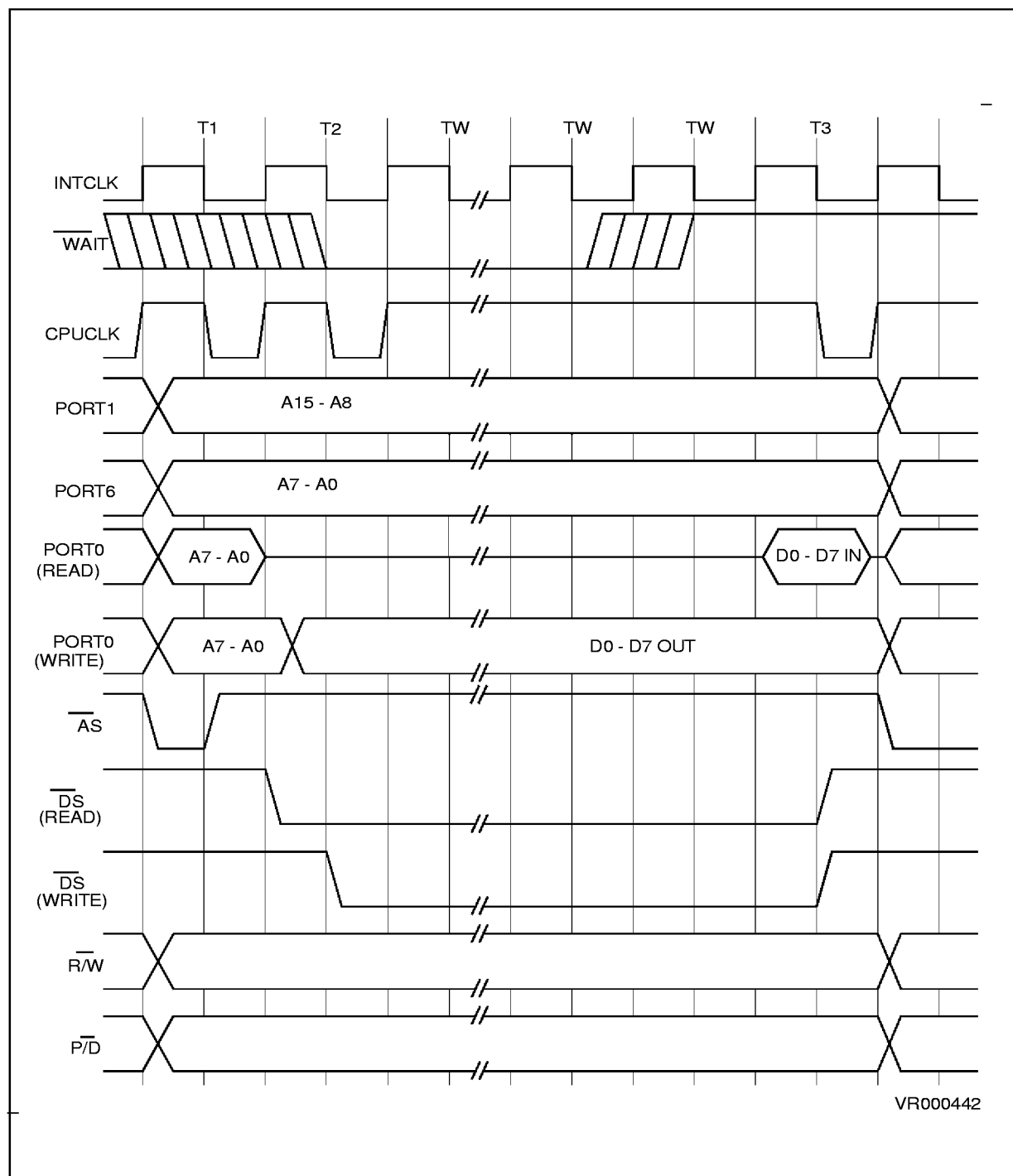
Figure 8-3. External Memory Read/Write Sequence with External Wait.
