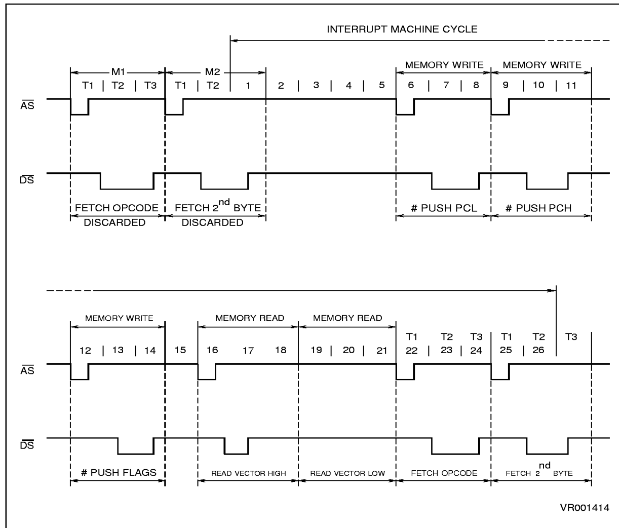
Figure 4-15. Interrupt Acknowledge Timing
