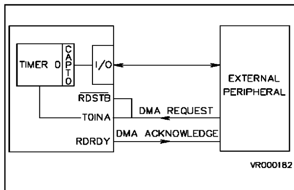
Figure 10-14. DMA output transfers with 2 lines output handshake
