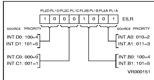
Figure 4-11. Priority Level Examples
