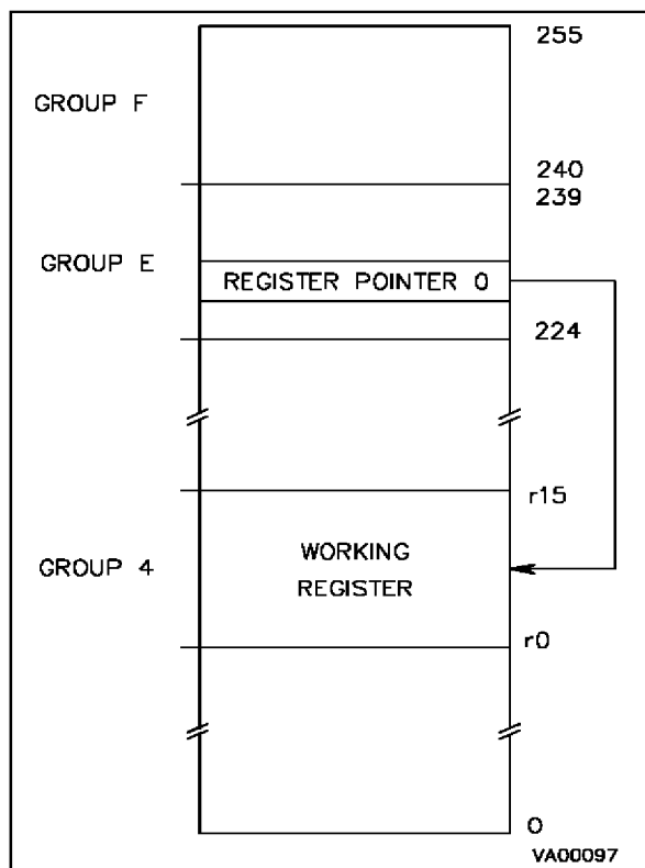
Figure 2-6. Single 16 Register pointing Mode
