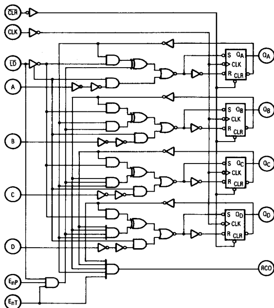
LOGIC DIAGRAM
