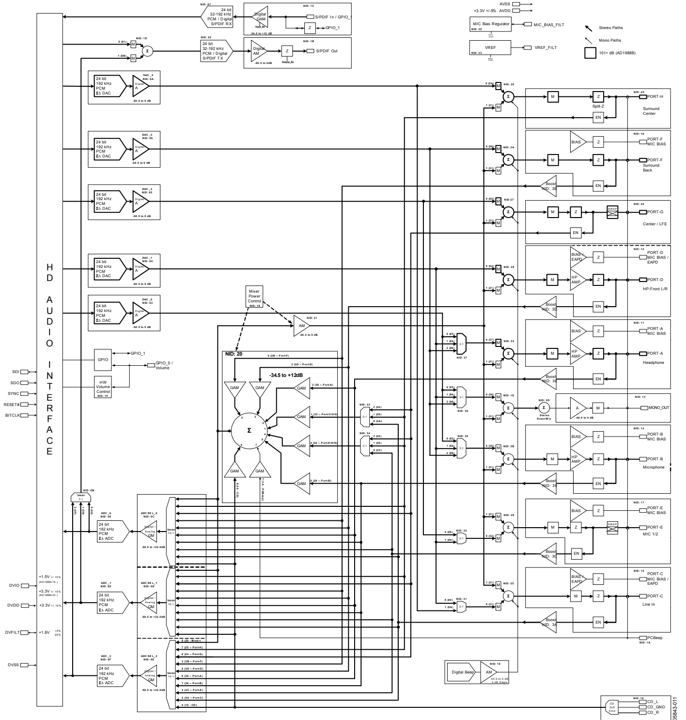
Figure 1. Block Diagram
