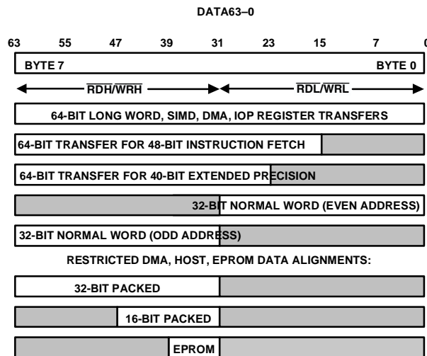
Figure 3. ADSP-21160N External Data Alignment Options
